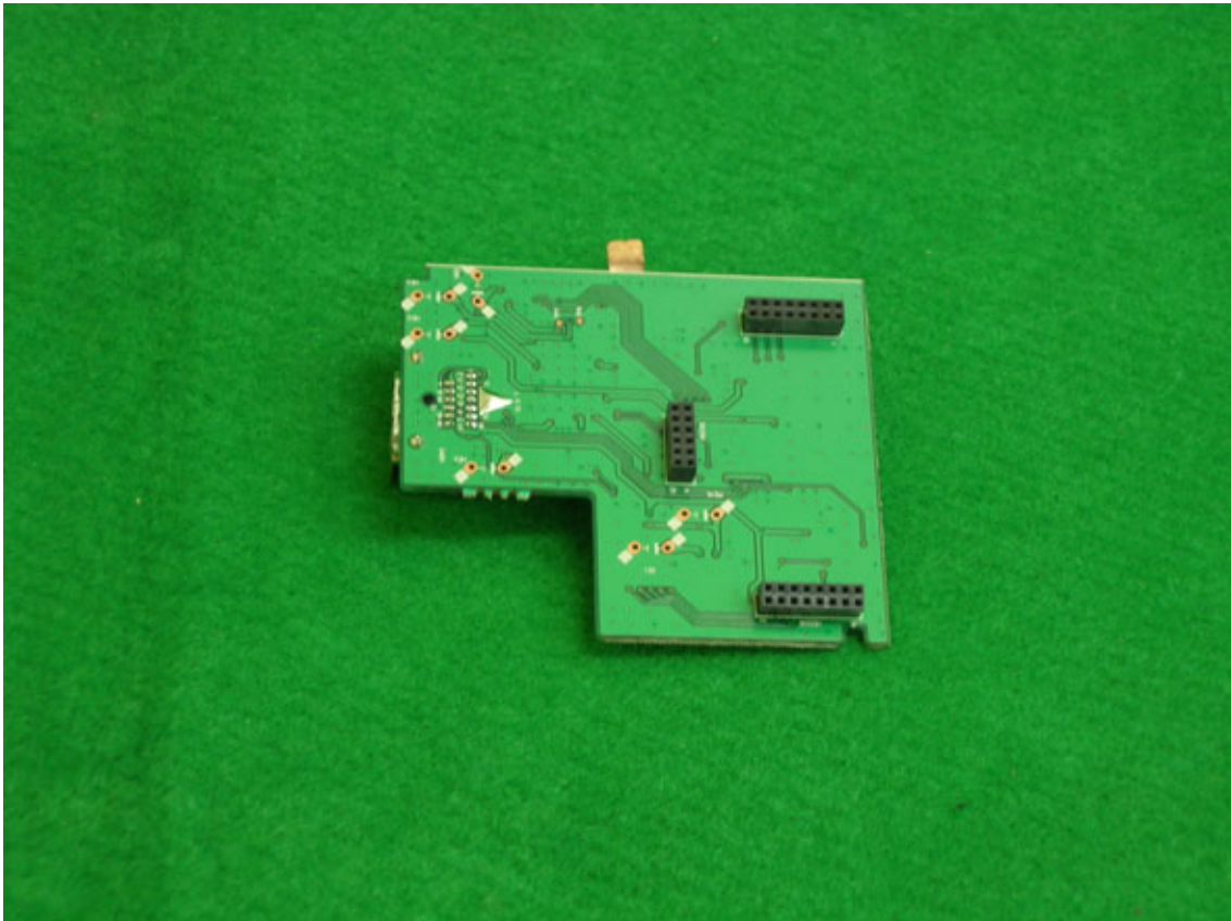
Bottom of SMPS PCB View
