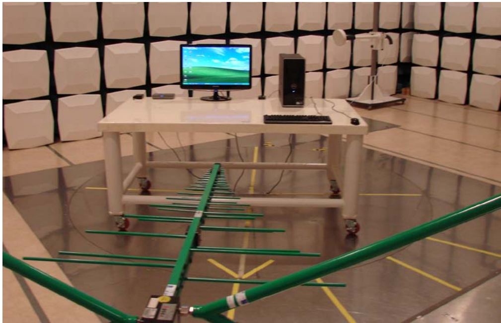
[ Radiated Disturbance for Below 1 GHz – Front ]
