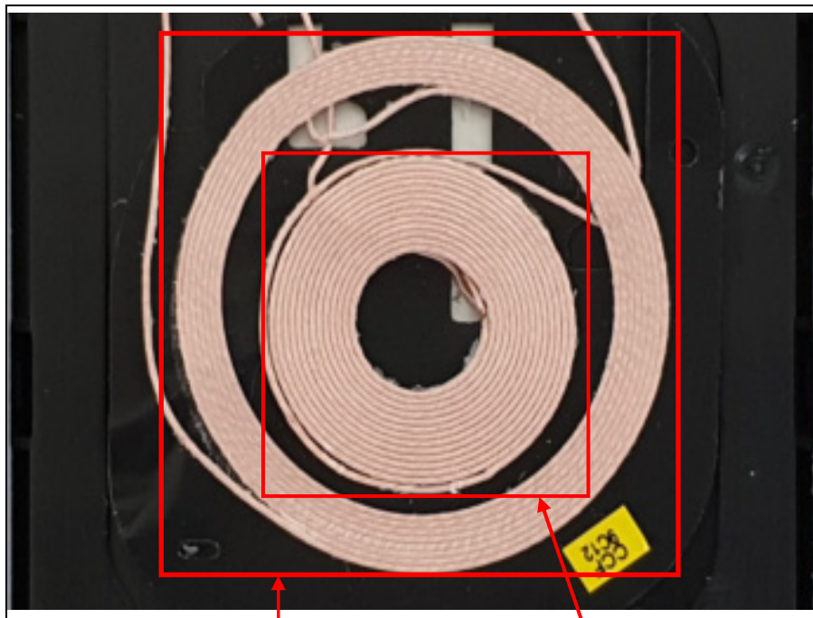
Loop coil antenna (ANT1)
