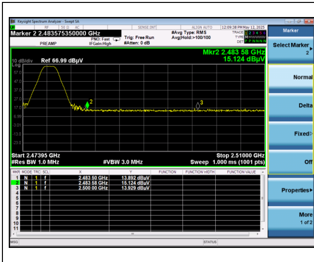
High channel band edge (Peak)
