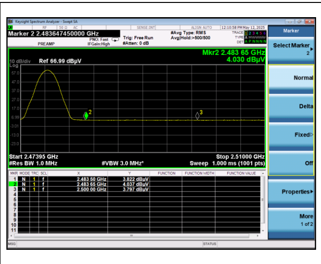
High channel band edge (Average)
