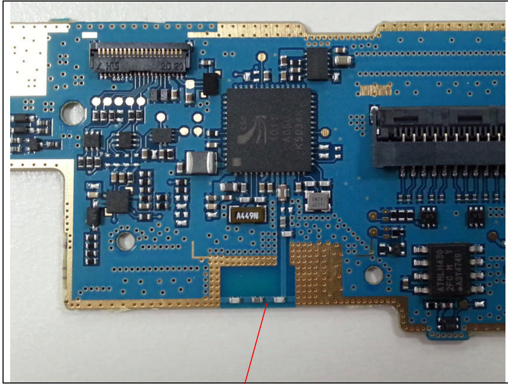
PCB Antenna
