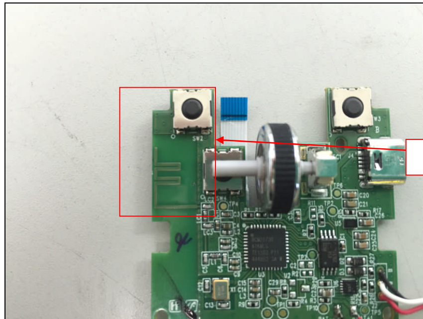
Pattern Antenna
