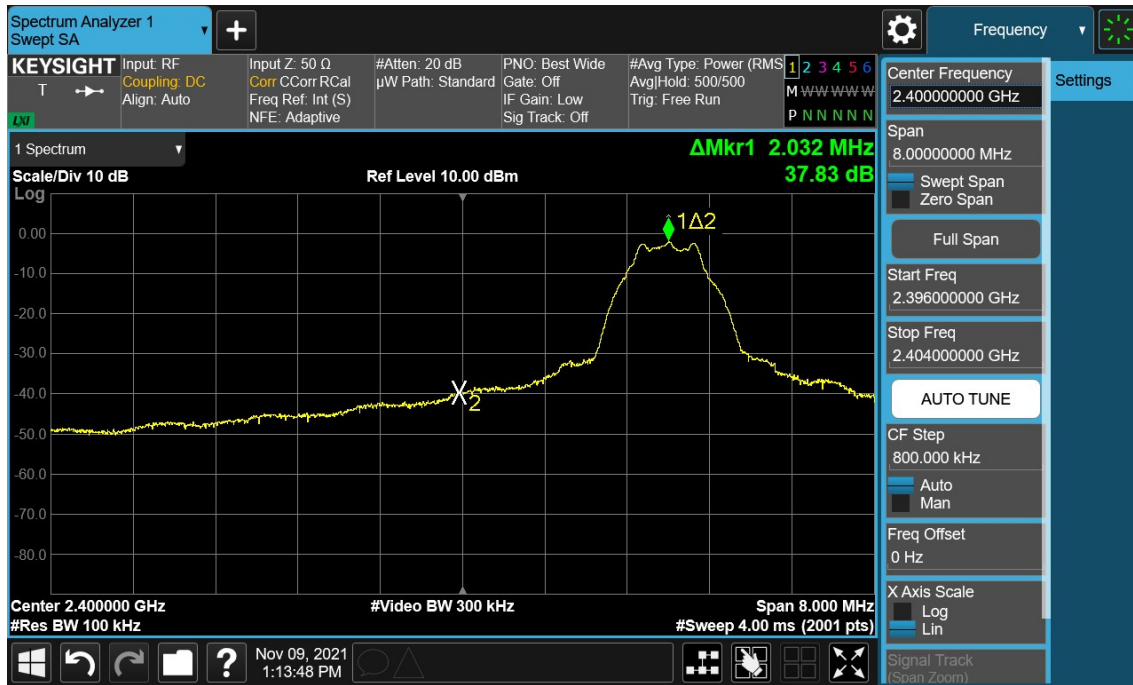
Plot 7-10. Band Edge Plot (Bluetooth (LE), 1Mbps – Ch. 0)
