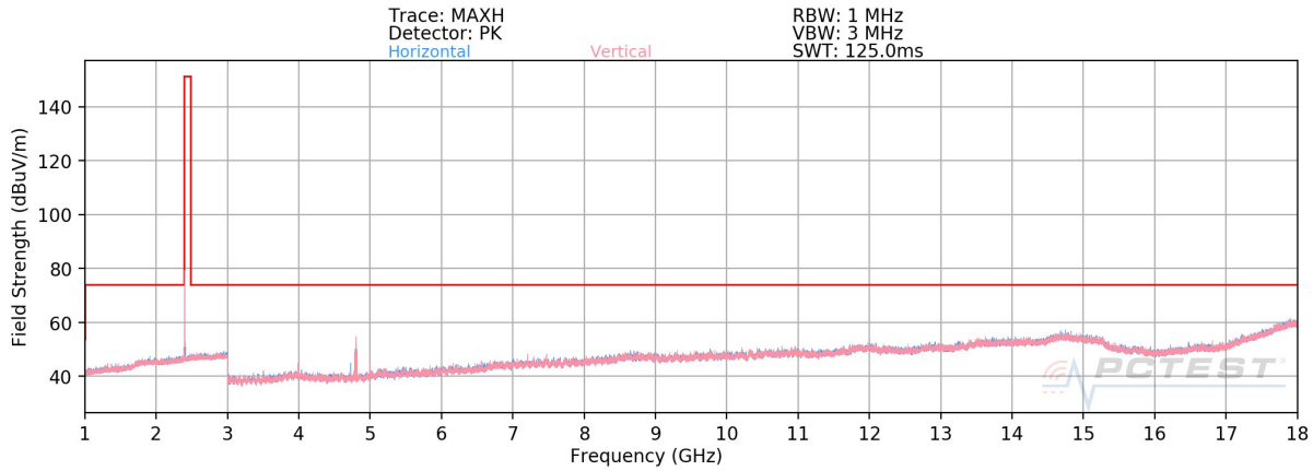
Plot 7-18. Radiated Spurious Plot above 1GHz (Bluetooth (LE) – Ch. 0)
