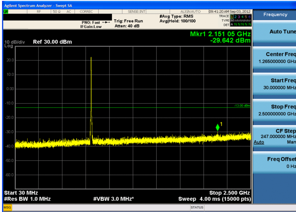
Plot 7-1. Conducted Spurious Plot (Cellular WCDMA Mode – Ch. 4132)
