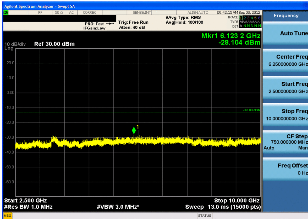
Plot 7-2. Conducted Spurious Plot (Cellular WCDMA Mode – Ch. 4132)
