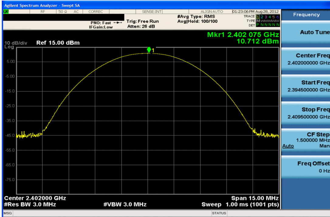
Plot 6-10 Peak Conducted Power (1Mbps – Ch. 0)
