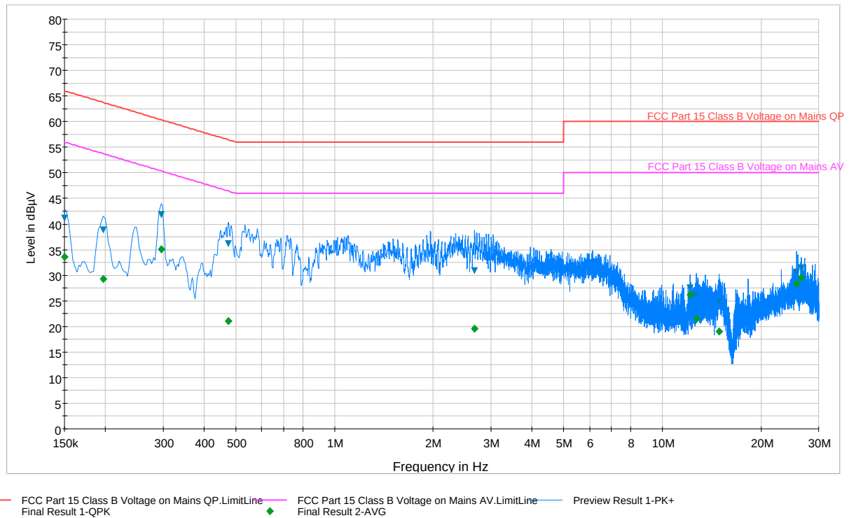
Plot 6-42. Line-Conducted Test Plot (L1)
