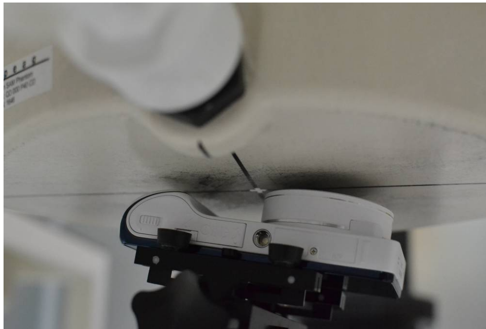
SAR Test Setup Photo 2 – Front Side at 0.5 cm
