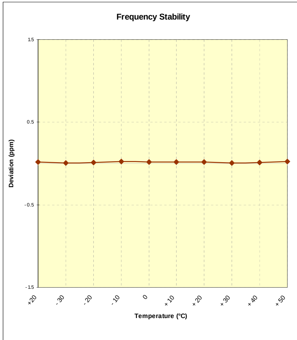
Figure 6-1. Frequency Stability Graph
