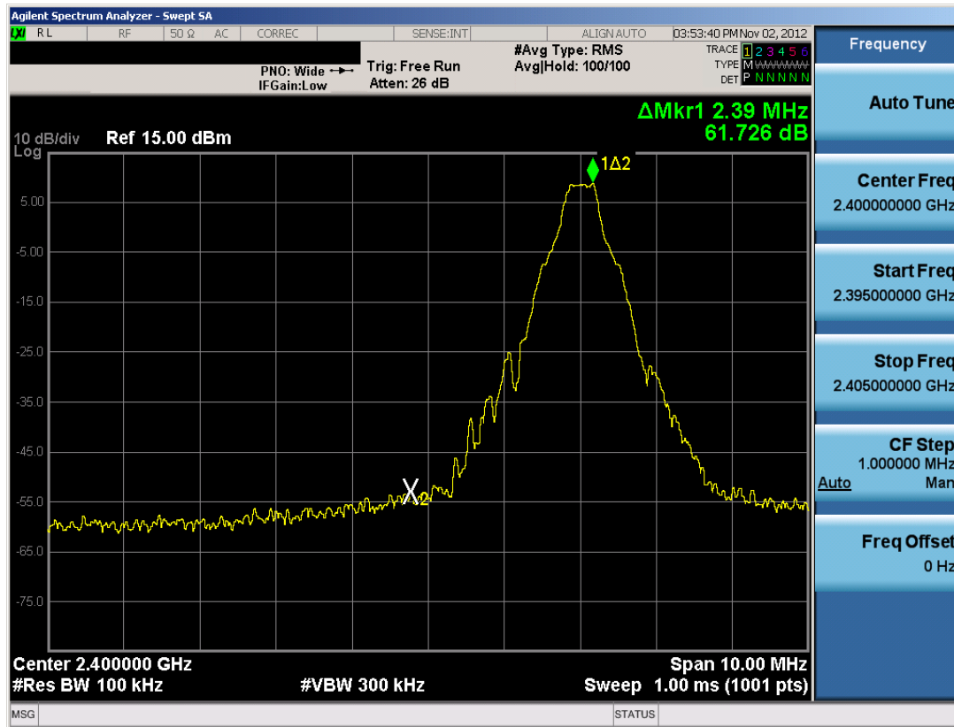
Plot 6-19. Band Edge Plot (Bluetooth with Hopping Disabled, 1Mbps – Ch. 0)
