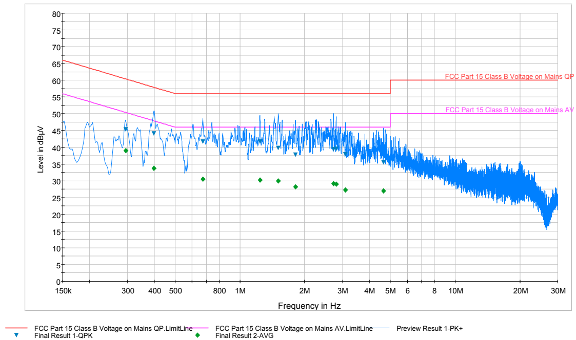
Plot 6-33. Line-Conducted Test Plot (L1)
