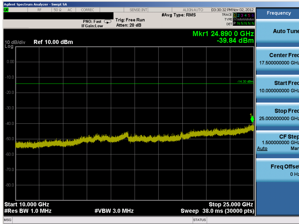
Plot 6-28. Conducted Spurious Plot (Bluetooth, 1Mbps – Ch. 0)
