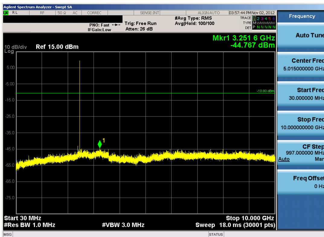
Plot 6-31. Conducted Spurious Plot (Bluetooth, 1Mbps – Ch. 78)
