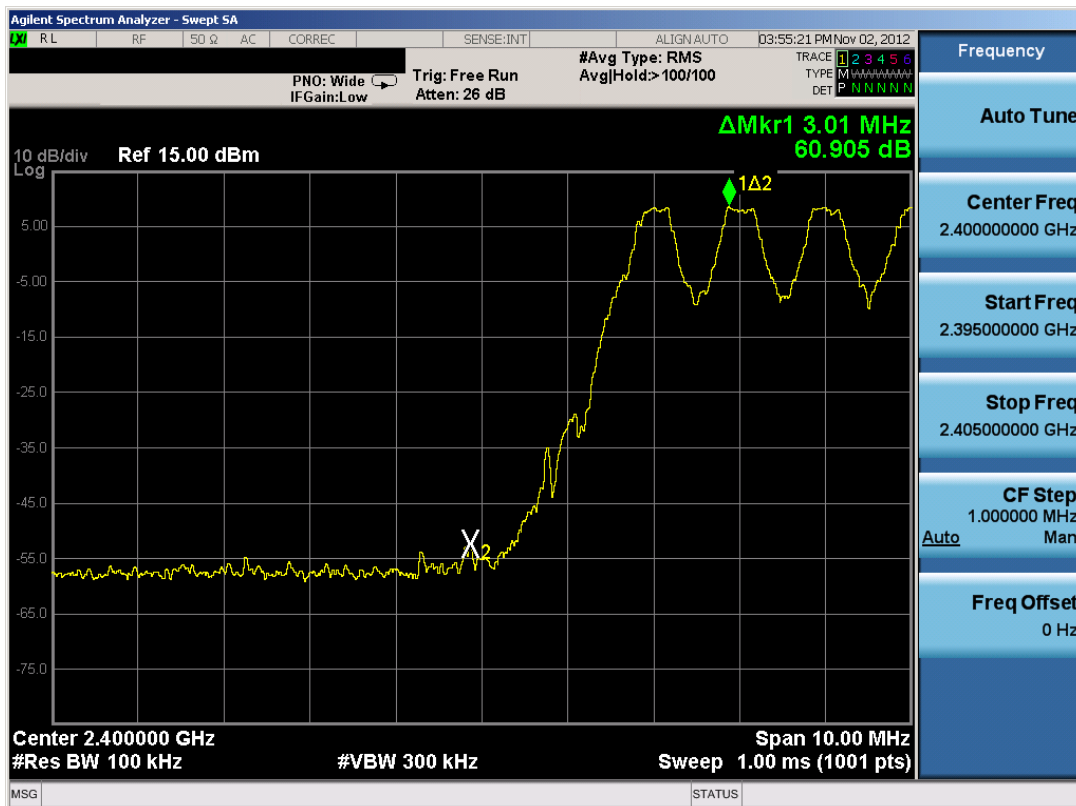
Plot 6-21. Band Edge Plot (Bluetooth with Hopping Enabled, 1Mbps)
