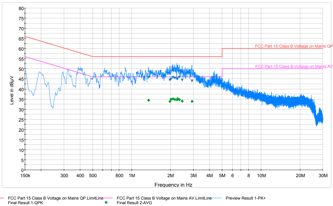
Plot 6-34. Line-Conducted Test Plot (N)
