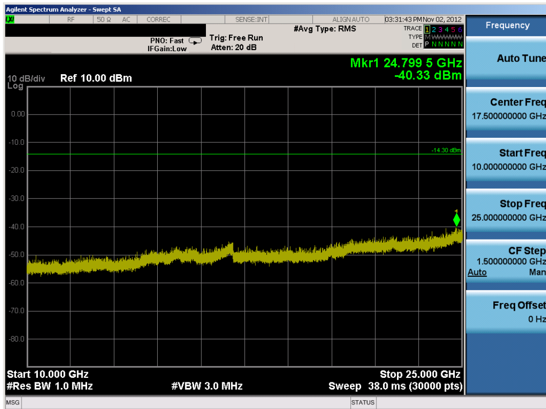
Plot 6-32. Conducted Spurious Plot (Bluetooth, 1Mbps – Ch. 78)
