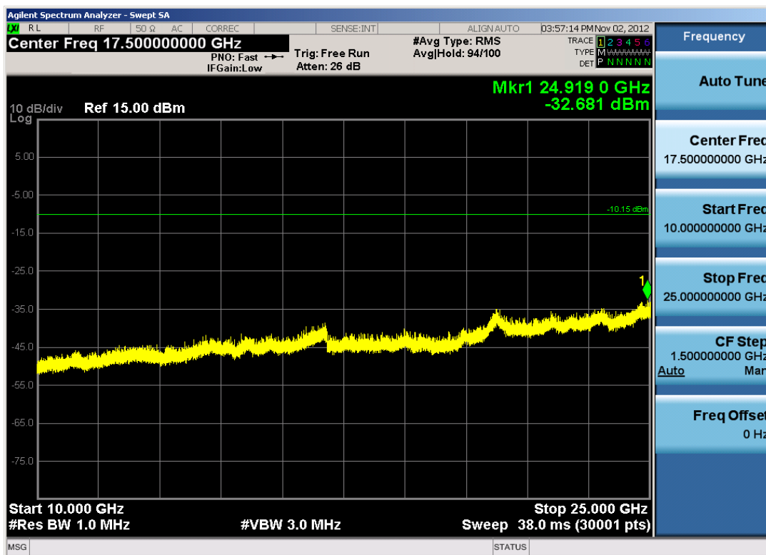
Plot 6-30. Conducted Spurious Plot (Bluetooth, 1Mbps – Ch. 39)
