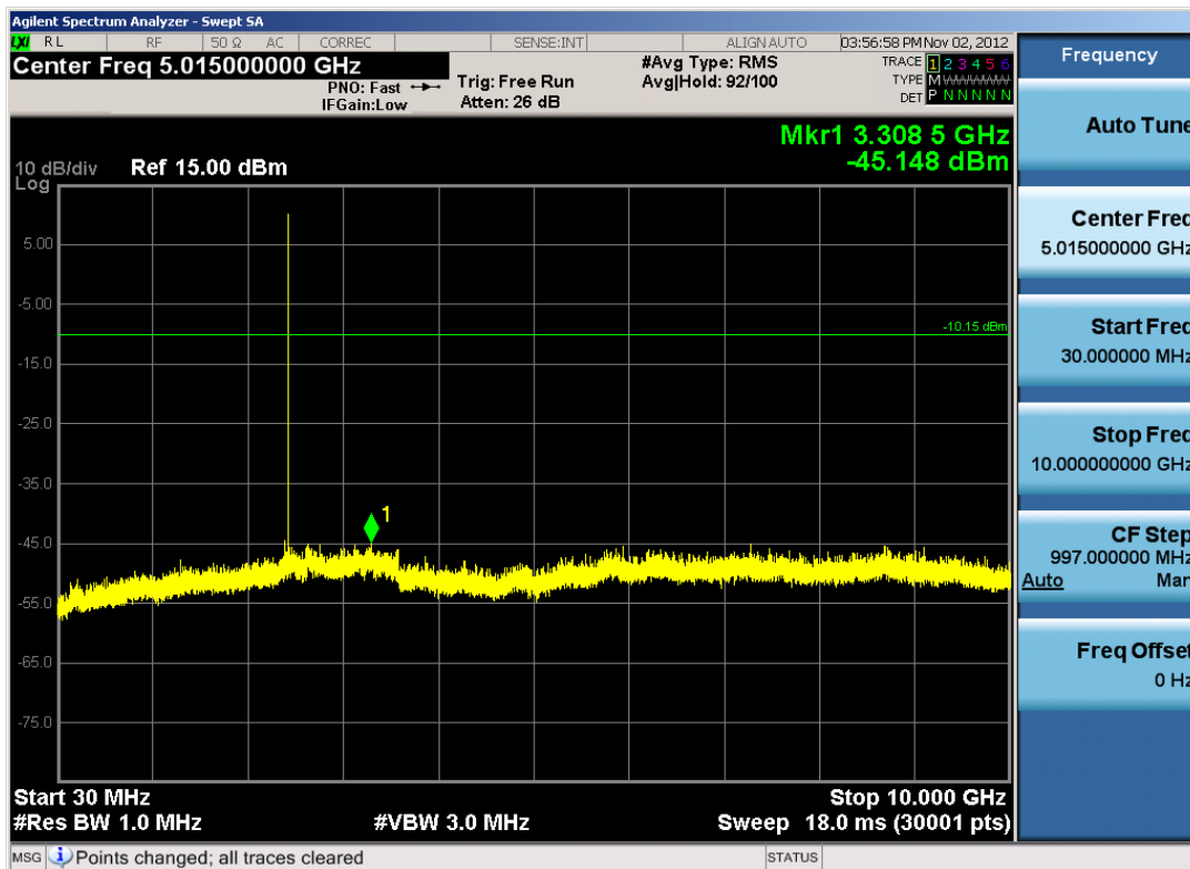
Plot 6-29. Conducted Spurious Plot (Bluetooth, 1Mbps – Ch. 39)
