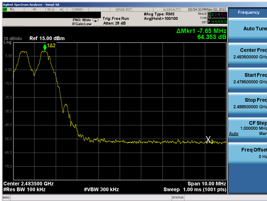
Plot 6-22. Band Edge Plot (Bluetooth with Hopping Enabled, 1Mbps)
