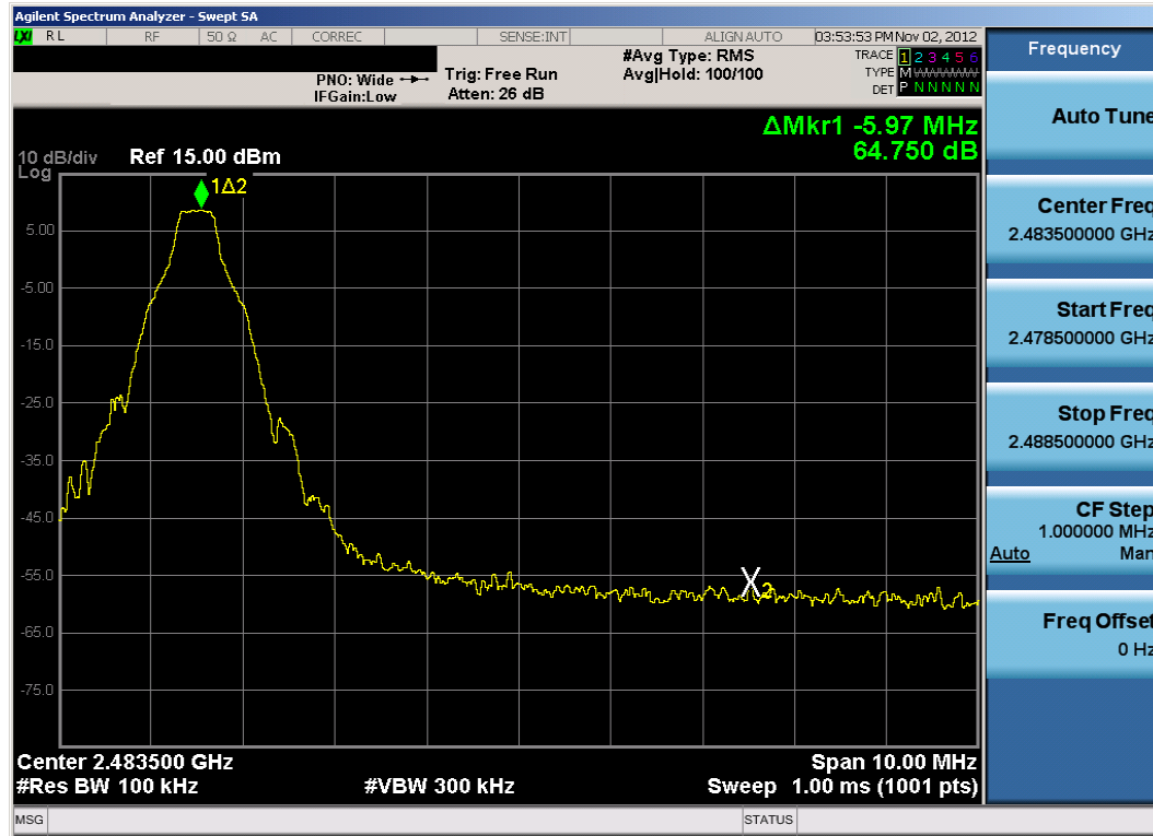
Plot 6-20. Band Edge Plot (Bluetooth with Hopping Disabled, 1Mbps – Ch. 78)
