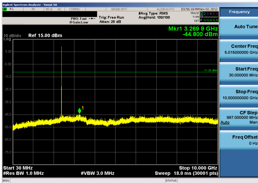
Plot 6-27. Conducted Spurious Plot (Bluetooth, 1Mbps – Ch. 0)
