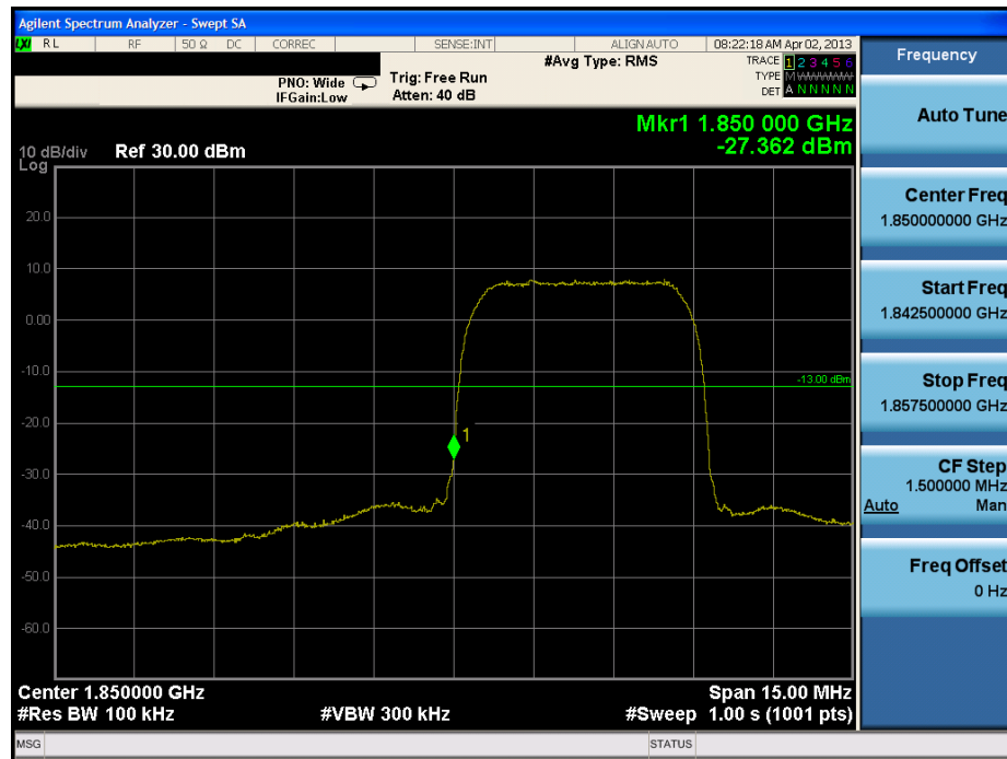
Plot 7-12. Band Edge Plot (PCS WCDMA Mode – Ch. 9262)
