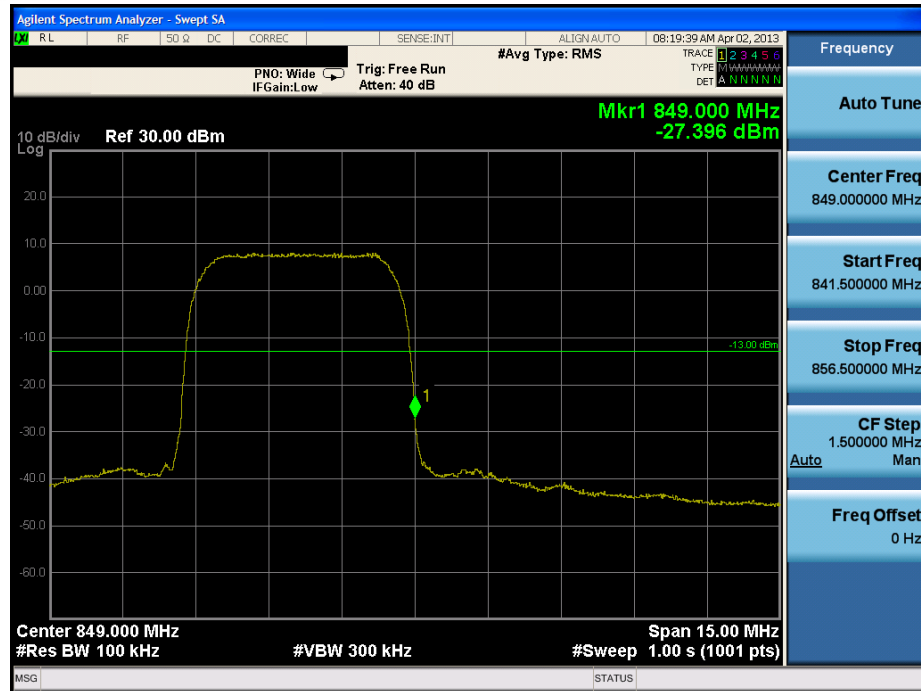
Plot 7-9. Band Edge Plot (Cellular WCDMA Mode - Ch. 4233)
