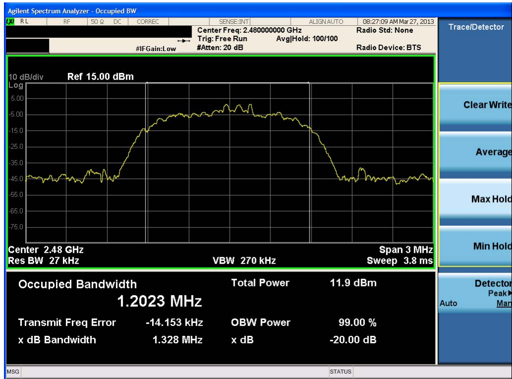
Plot 6-9. 20dB Bandwidth Plot (Bluetooth, 3Mbps – Ch. 78)
