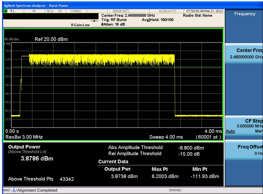
Plot 6-24. Average Conducted Power (2Mbps – Ch. 78)
