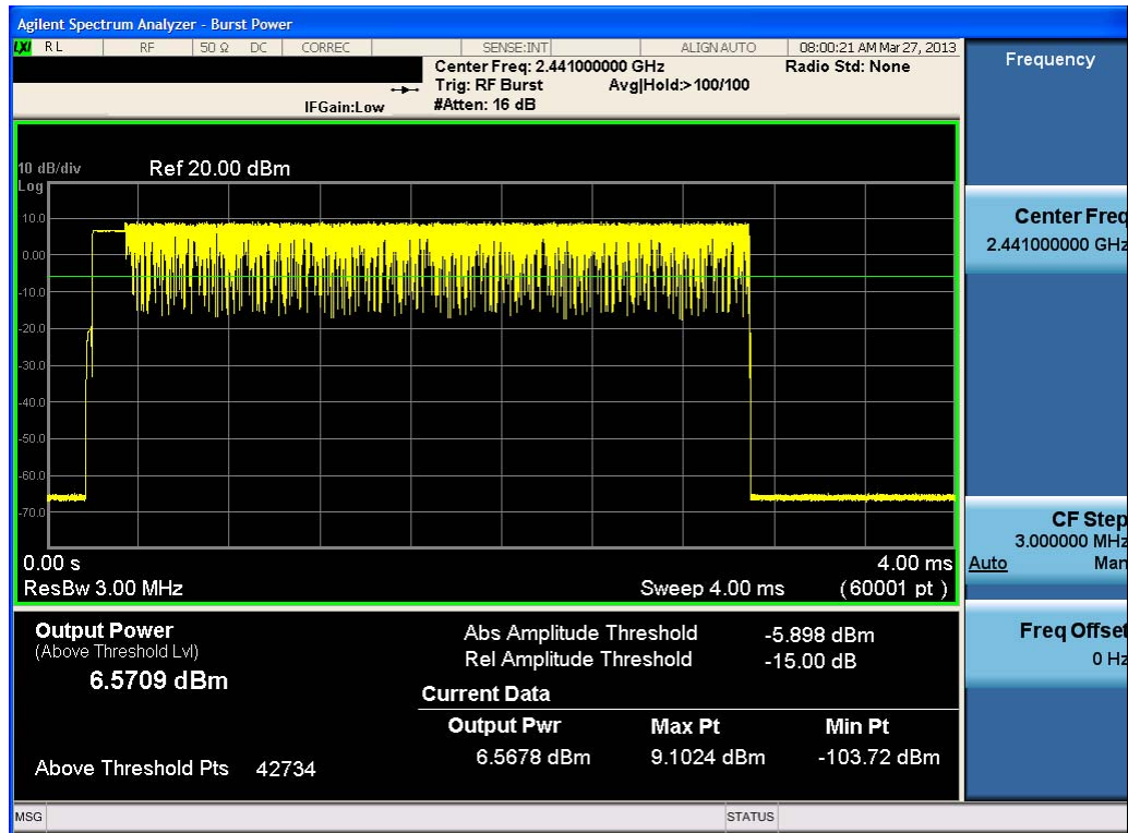
Plot 6-26. Average Conducted Power (3Mbps – Ch. 39)
