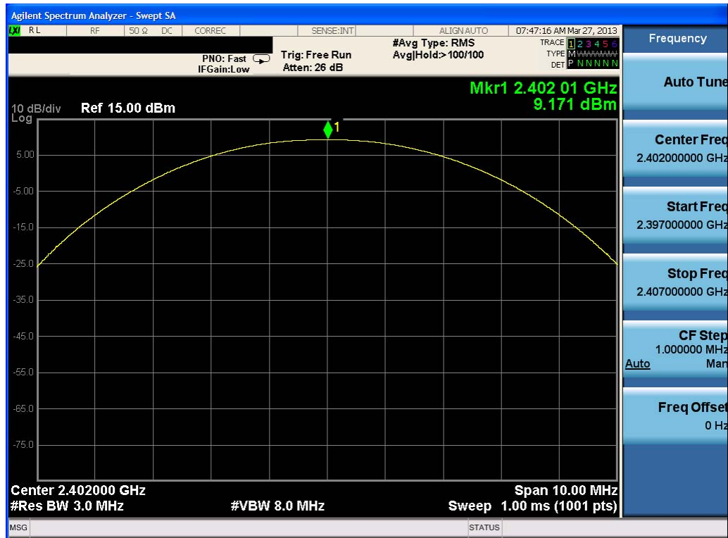
Plot 6-10. Peak Conducted Power (1Mbps – Ch. 0)
