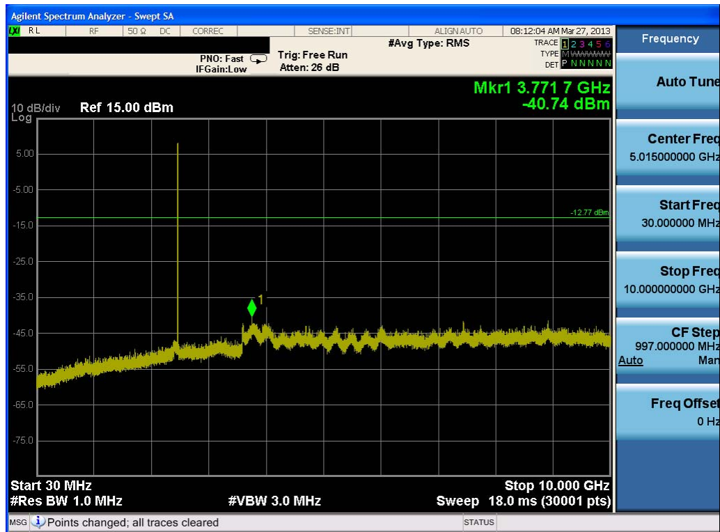
Plot 6-40. Conducted Spurious Plot (Bluetooth, 1Mbps – Ch. 78)
