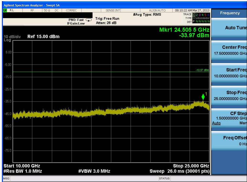
Plot 6-37. Conducted Spurious Plot (Bluetooth, 1Mbps – Ch. 0)
