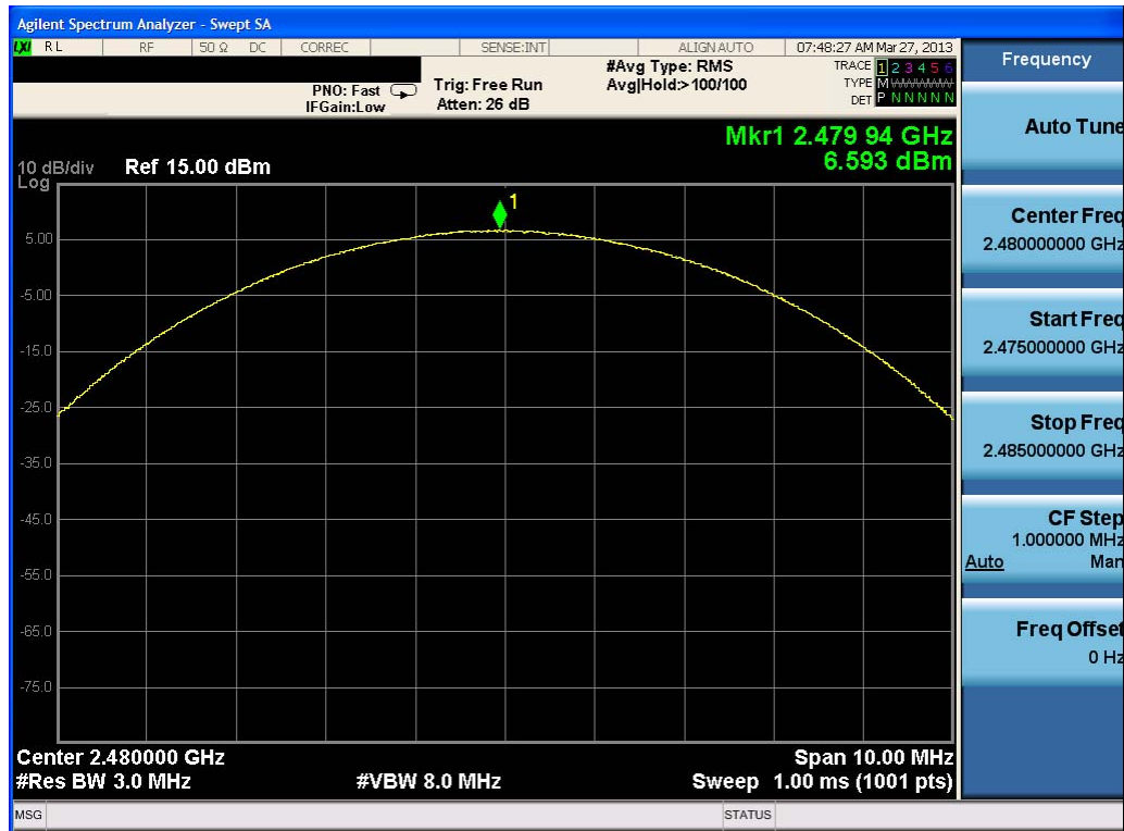
Plot 6-18. Peak Conducted Power (3Mbps – Ch. 78)
