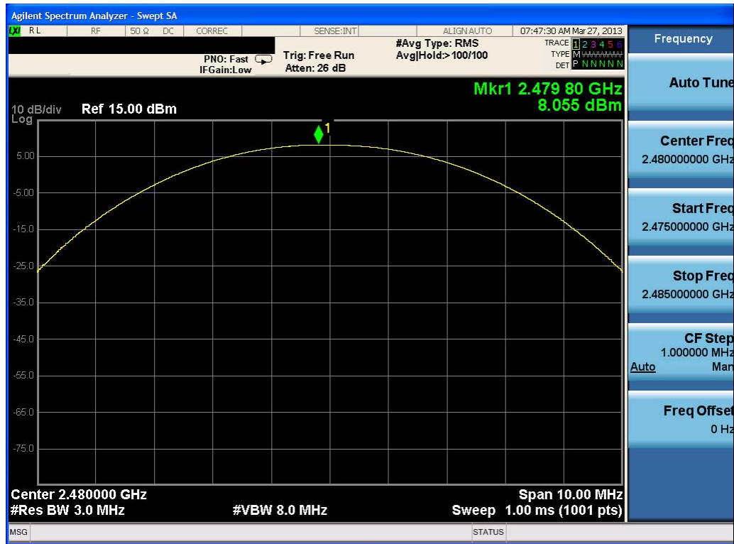
Plot 6-12. Peak Conducted Power (1Mbps – Ch. 78)
