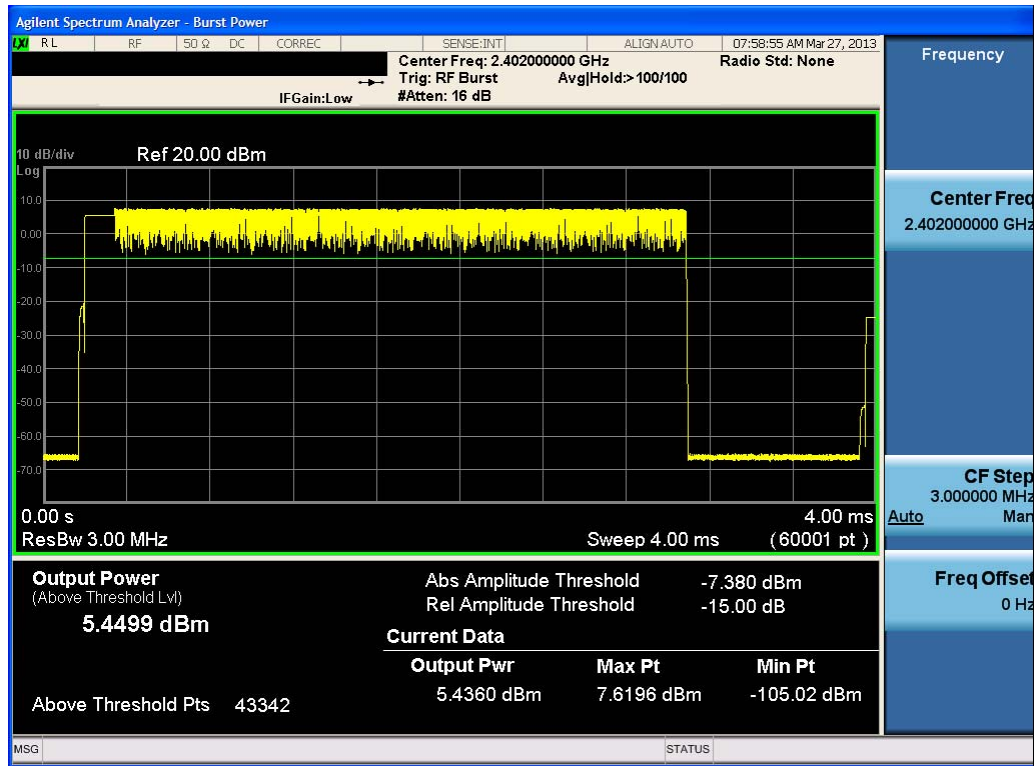
Plot 6-22. Average Conducted Power (2Mbps – Ch. 0)
