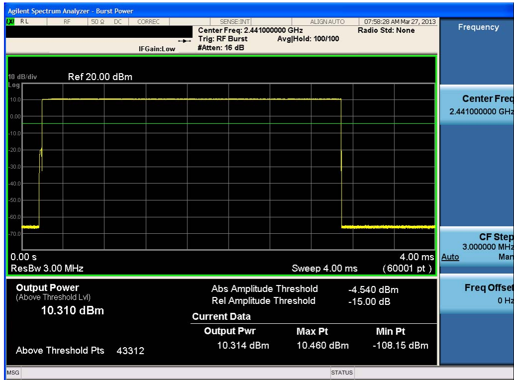
Plot 6-20. Average Conducted Power (1Mbps – Ch. 39)
