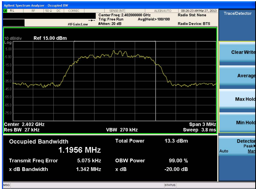
Plot 6-4. 20dB Bandwidth Plot (Bluetooth, 2Mbps – Ch. 0)
