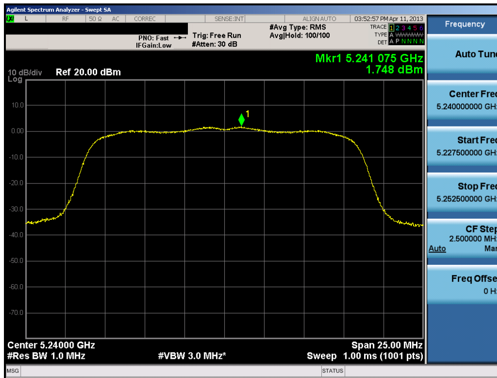
Plot 6-28. Peak Power Spectral Density Plot (802.11a (UNII Band 1) – Ch. 48)
