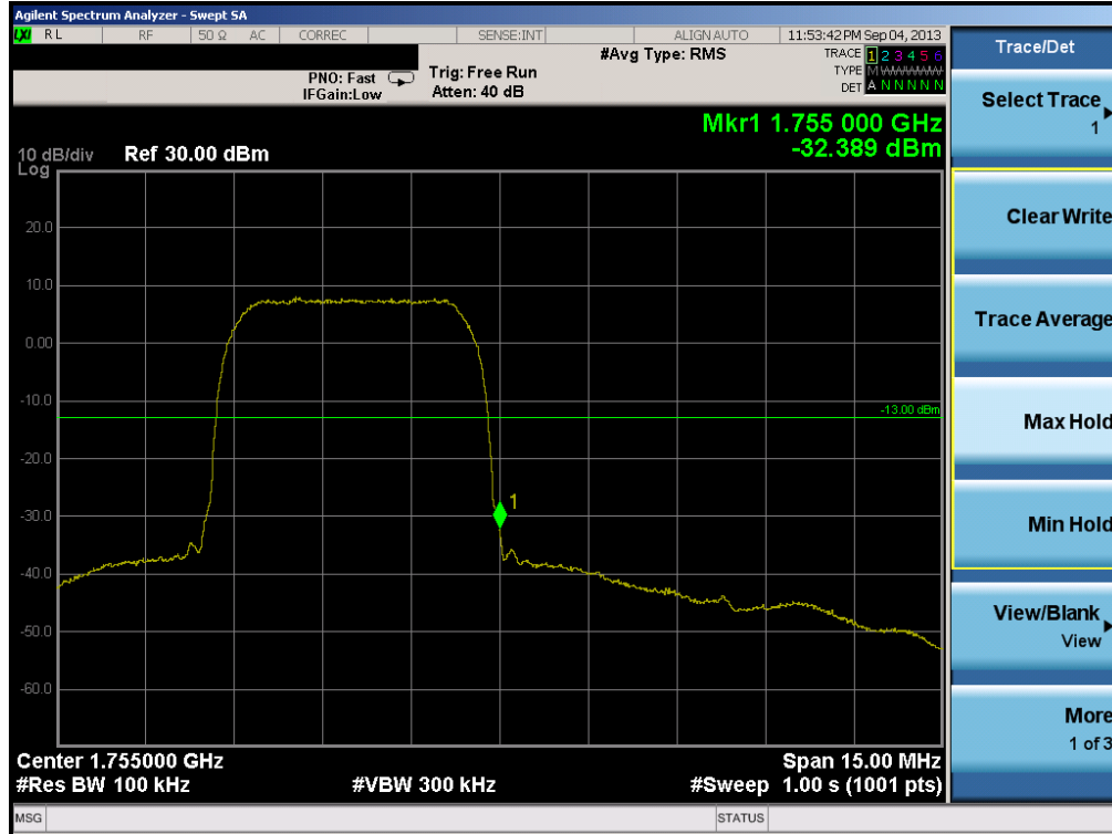
Plot 6-26. Band Edge Plot (AWS WCDMA Mode – Ch. 1862)
