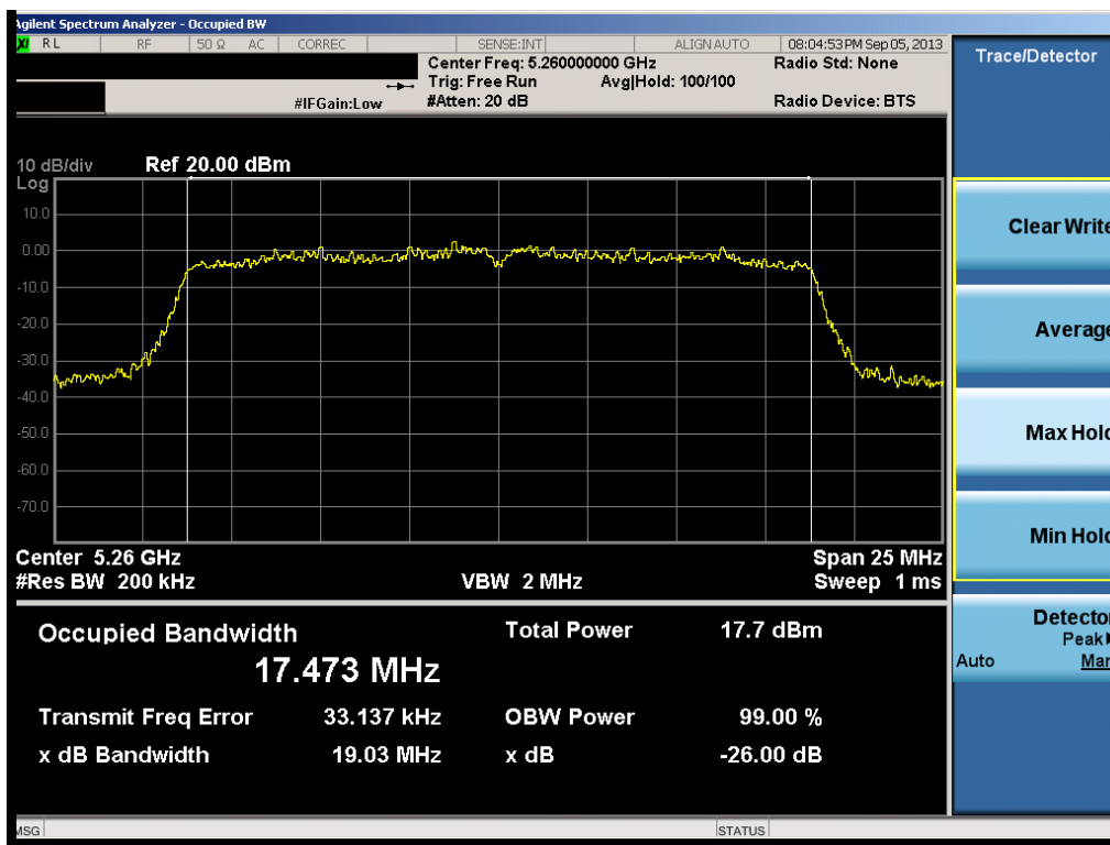
Plot 6-12. 26dB Bandwidth Plot (20MHz BW 802.11n (UNII Band 2) – Ch. 52)
