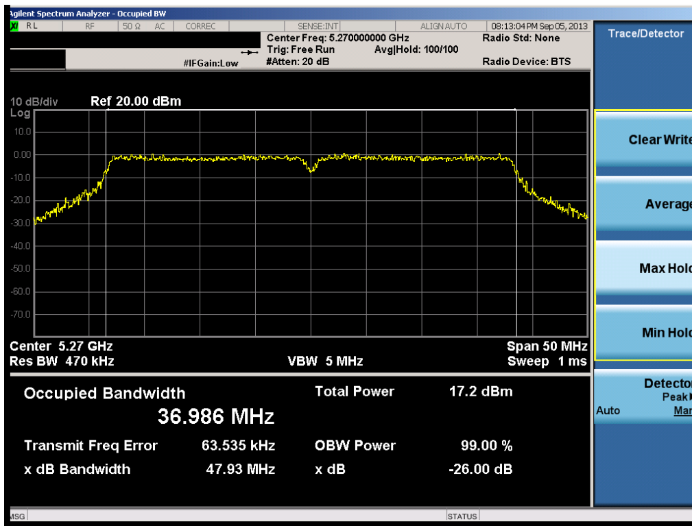
Plot 6-15. 26dB Bandwidth Plot (40MHz BW 802.11n (UNII Band 2) – Ch. 54)
