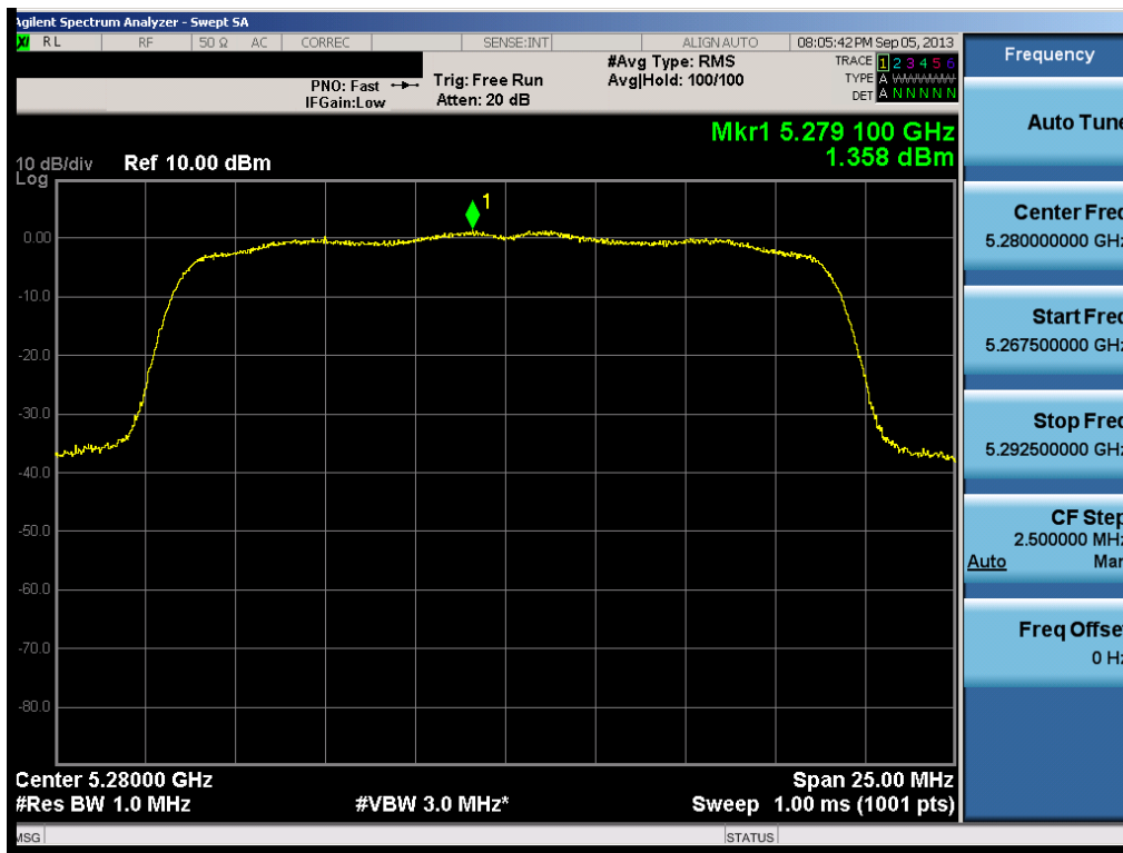
Plot 6-38. Peak Power Spectral Density Plot (20MHz BW 802.11n (UNII Band 2) – Ch. 56)
