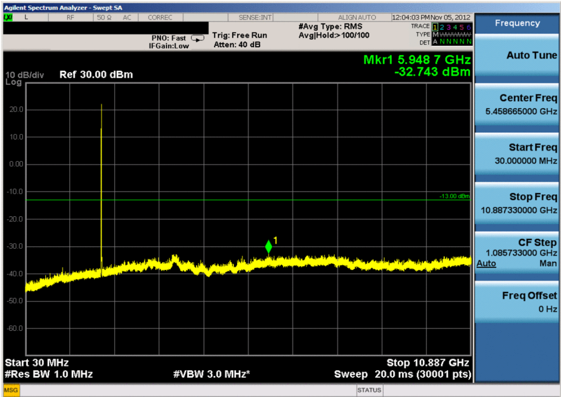
Plot 7-5. Conducted Spurious Plot (PCS WCDMA Mode – Ch. 9400)
