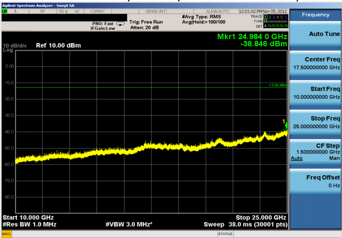
Plot 7-6. Conducted Spurious Plot (PCS WCDMA Mode – Ch. 9400)
