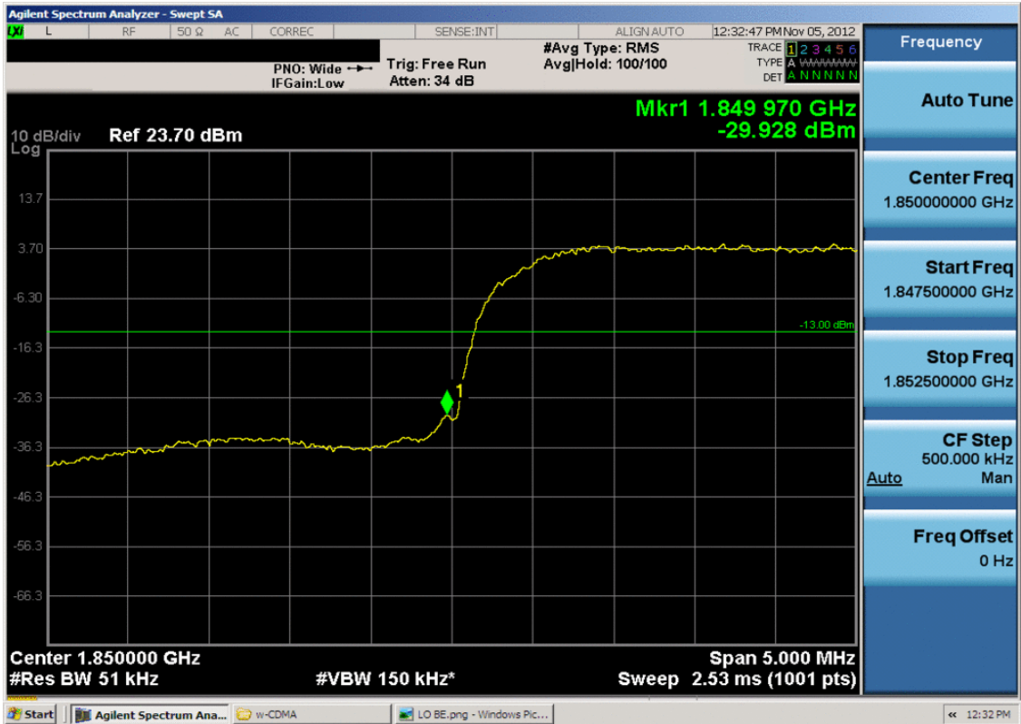
Plot 7-3. Band Edge Plot (PCS WCDMA Mode – Ch. 9262)
