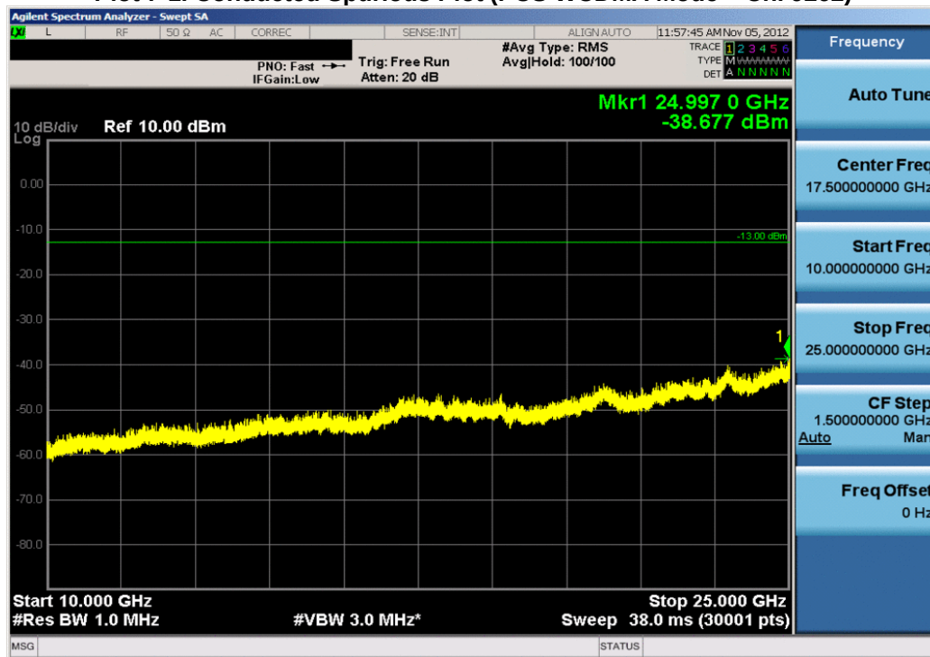
Plot 7-2. Conducted Spurious Plot (PCS WCDMA Mode – Ch. 9262)
