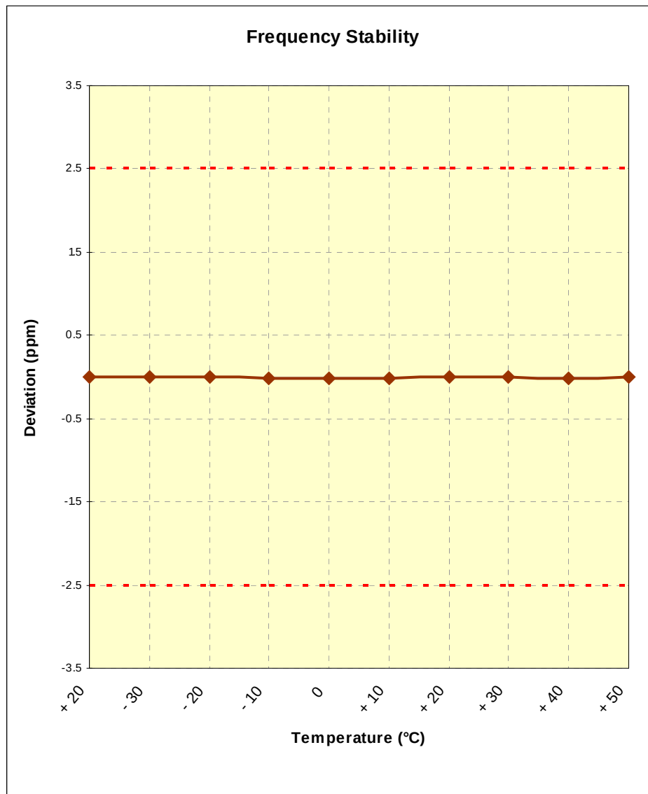
Figure 6-1. Frequency Stability Graph (PCS WCDMA Mode – Ch. 9400)
