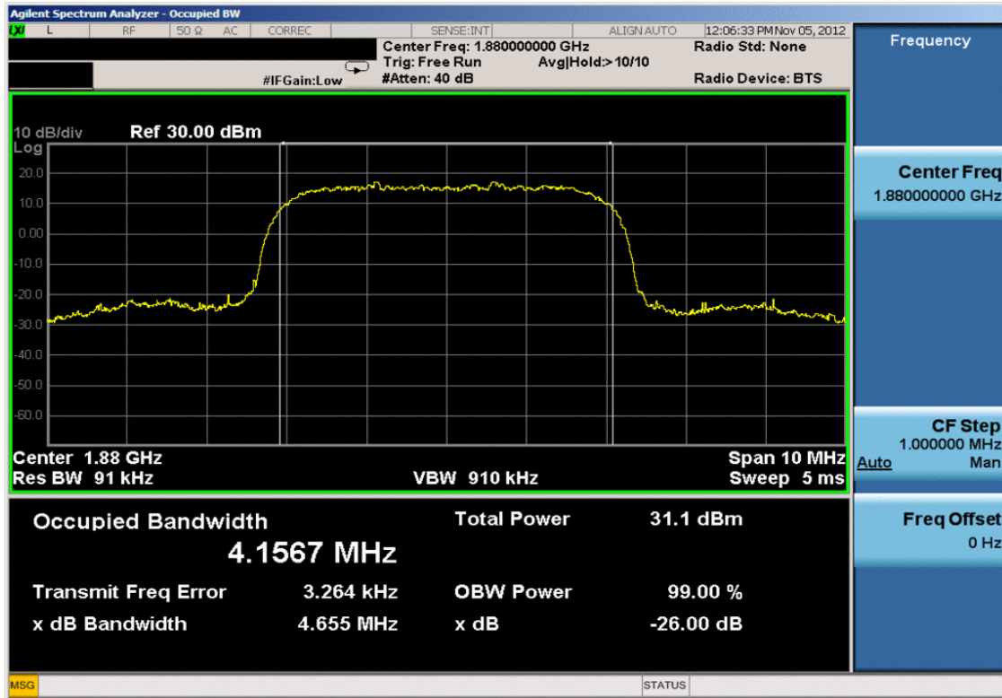
Plot 7-7. Occupied Bandwidth Plot (PCS WCDMA Mode – Ch. 9400)
