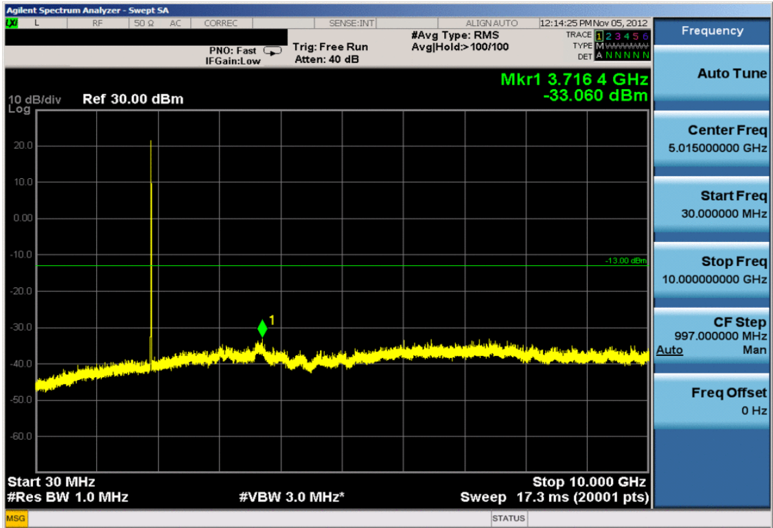
Plot 7-9. Conducted Spurious Plot (PCS WCDMA Mode – Ch. 9538)
