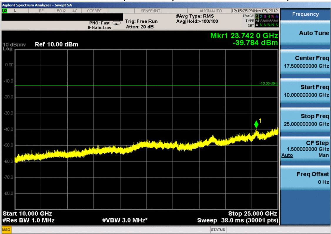
Plot 7-10. Conducted Spurious Plot (PCS WCDMA Mode – Ch. 9538)
