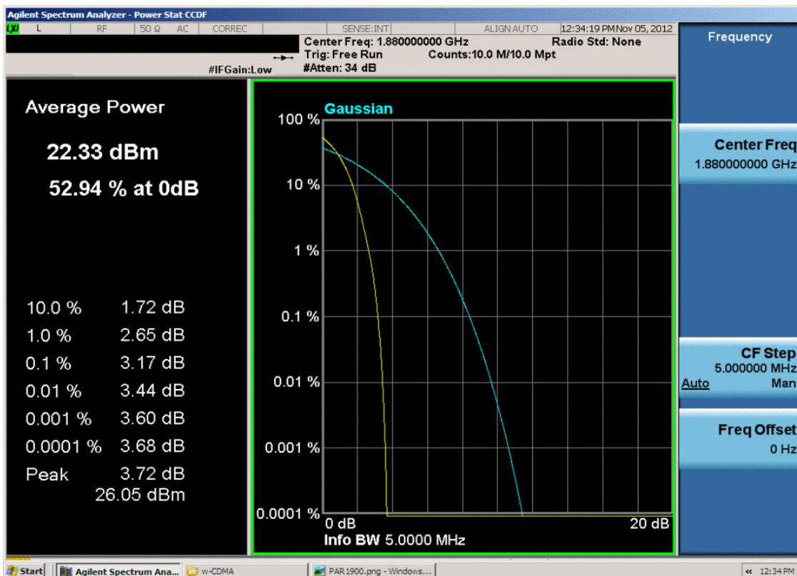
Plot 7-8. Peak-Average Ratio Plot (PCS WCDMA Mode – Ch. 9400)
