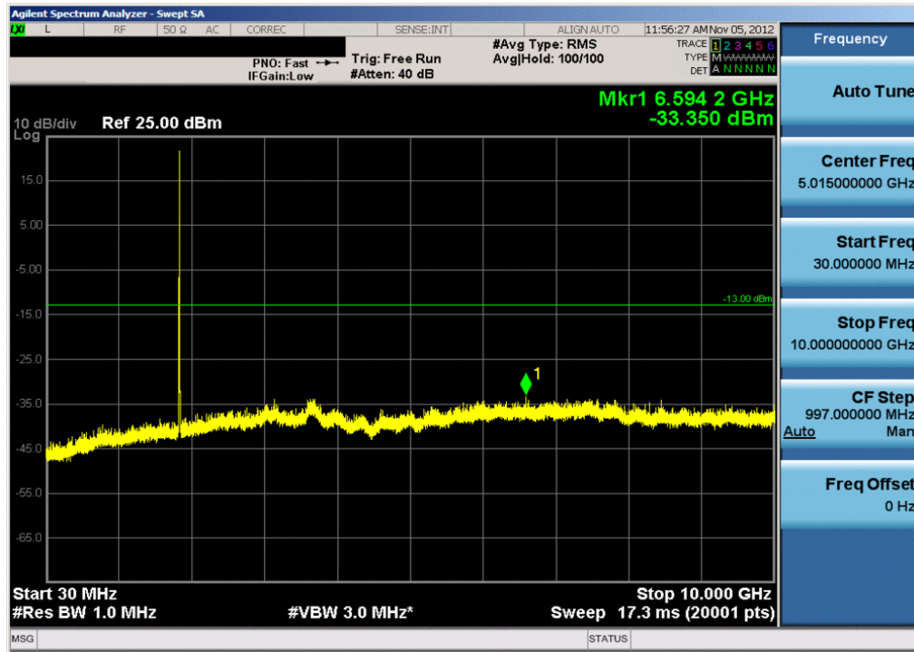
Plot 7-1. Conducted Spurious Plot (PCS WCDMA Mode – Ch. 9262)
