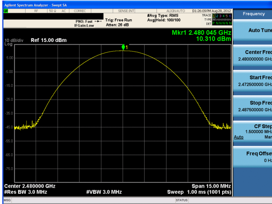
Plot 6-12. Peak Conducted Power (1Mbps – Ch. 78)
