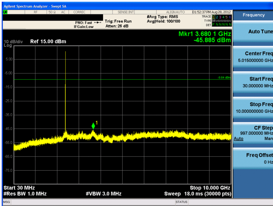
Plot 6-36. Conducted Spurious Plot (Bluetooth, 1Mbps – Ch. 0)
