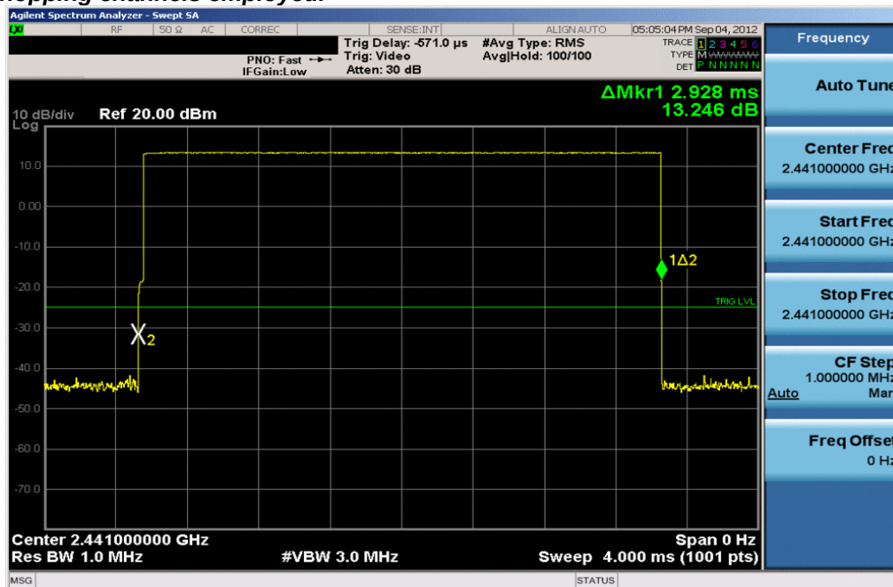
Plot 6-33. Time of Occupancy Plot (Bluetooth)
