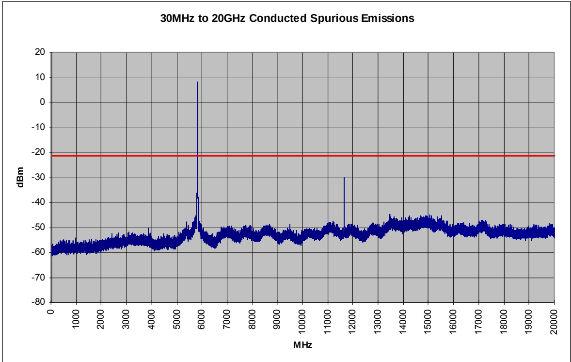
Plot 6-57. Conducted Spurious Plot (802.11a – Ch. 165)
