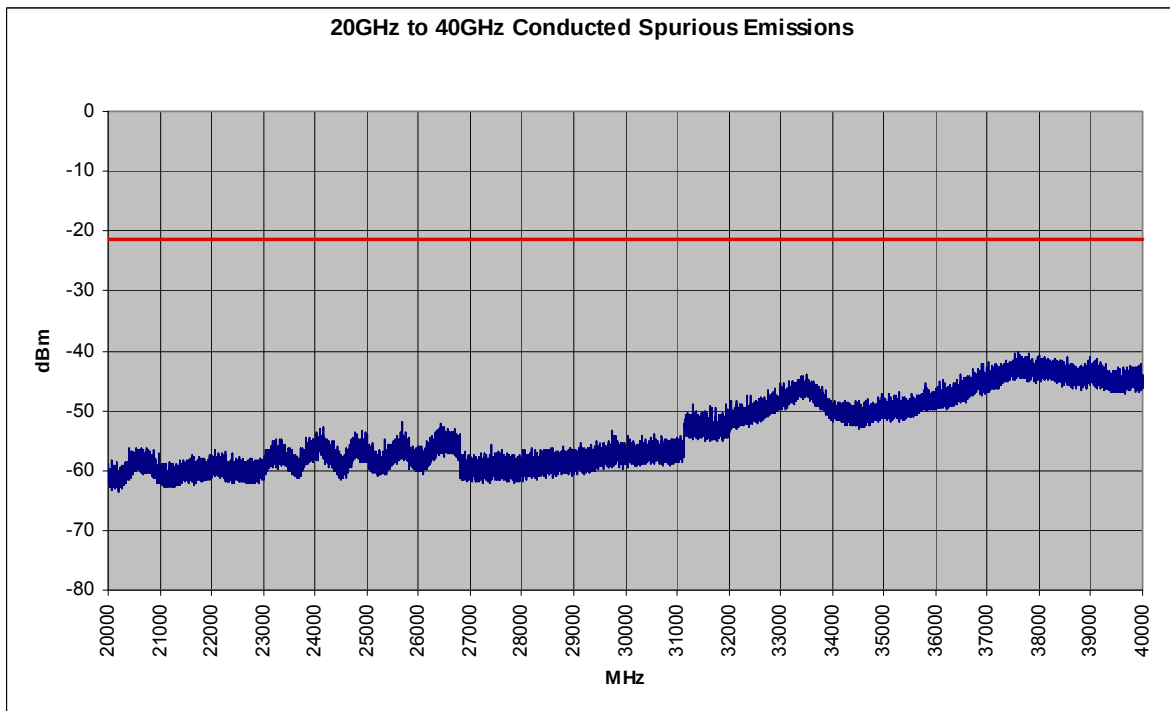
Plot 6-54. Conducted Spurious Plot (802.11a – Ch. 149)
