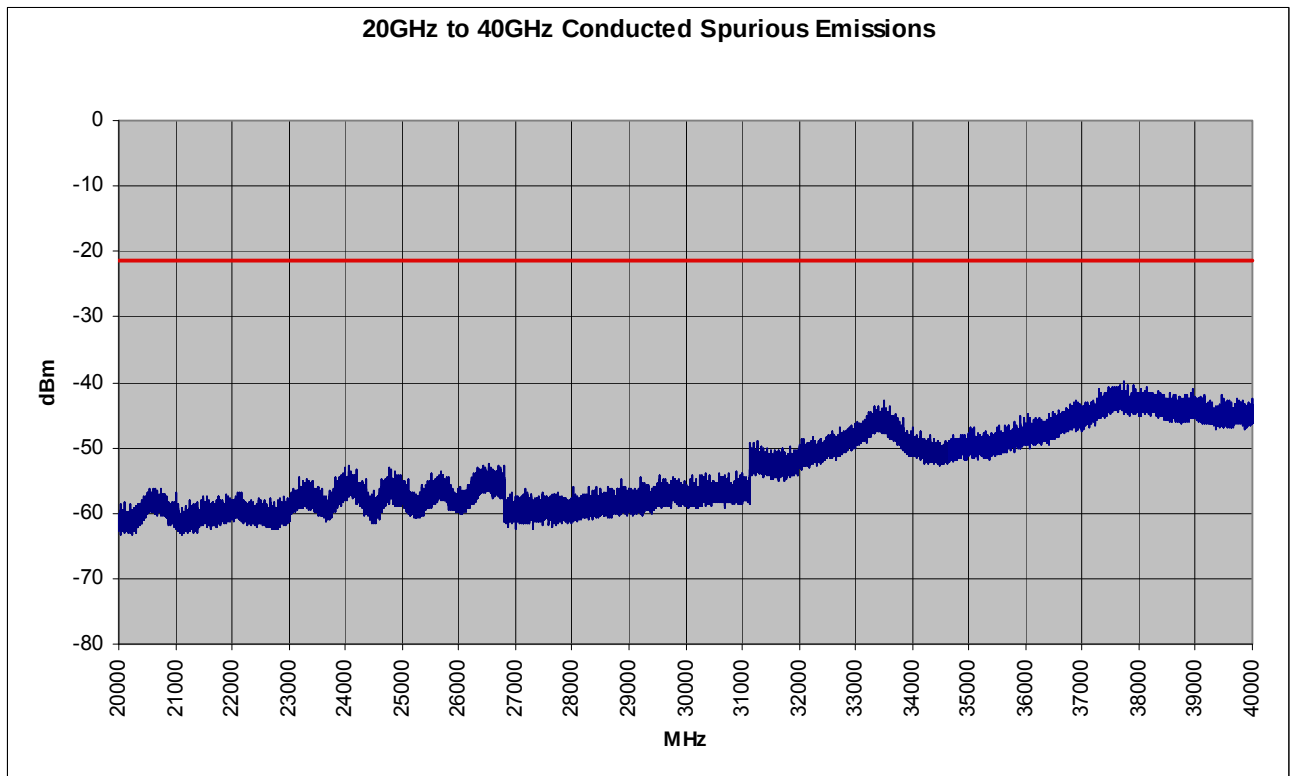
Plot 6-58. Conducted Spurious Plot (802.11a – Ch. 165)
