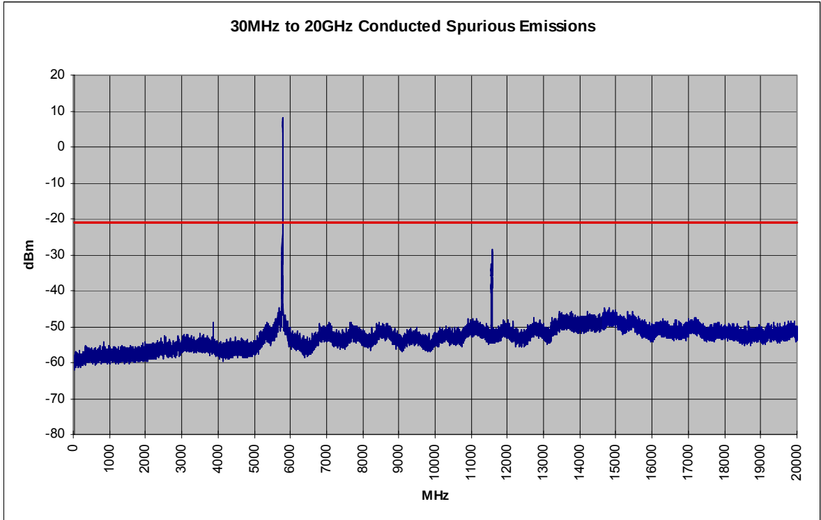
Plot 6-55. Conducted Spurious Plot (802.11a – Ch. 157)
