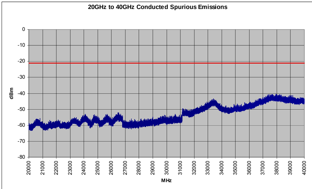
Plot 6-56. Conducted Spurious Plot (802.11a – Ch. 157)
