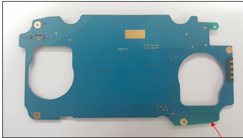
PCB Antenna
