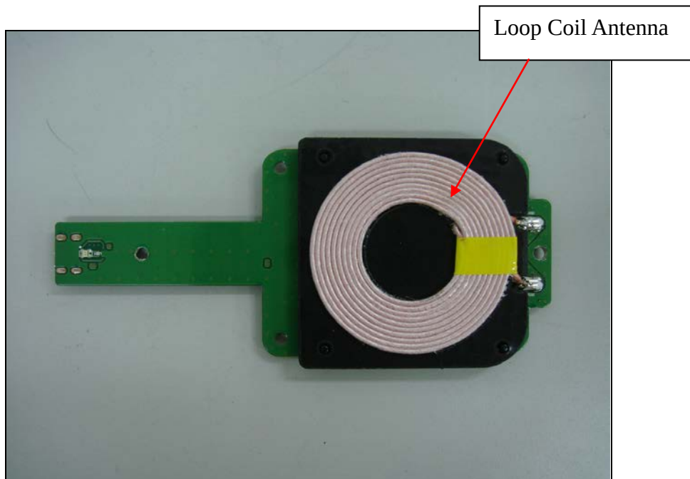
Bottom view of main board
