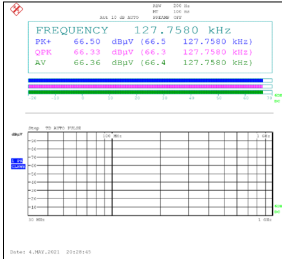
Ant. 1 (126.7 ~ 128.7 kHz)
