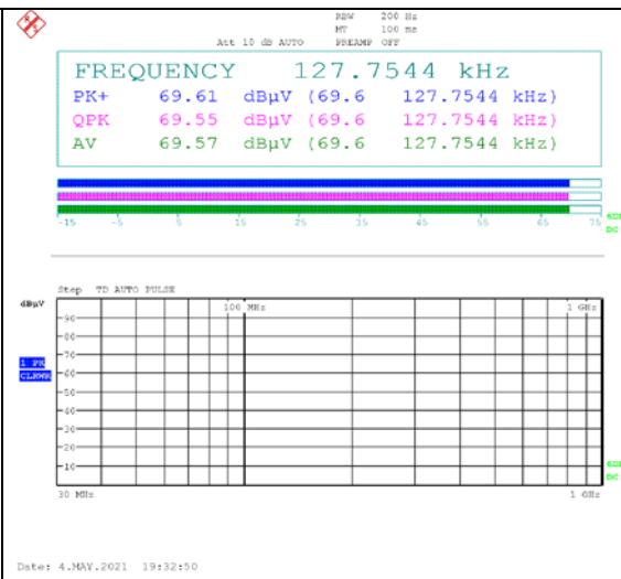
Ant. 2 (126.7 ~ 128.7 kHz)
