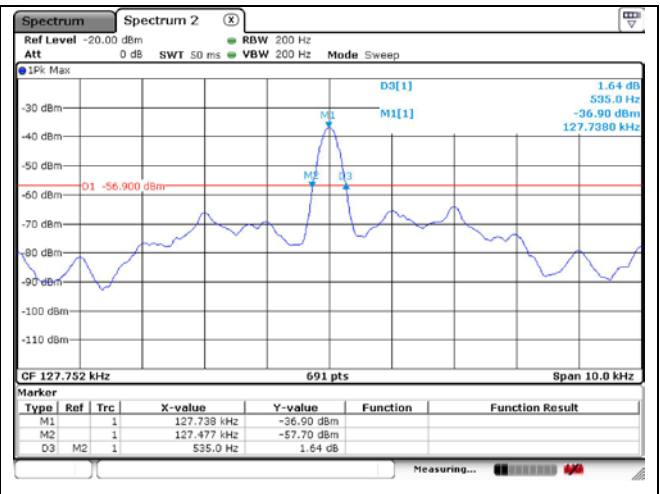
Ant. 2 (126.7 ~ 128.7 kHz)
