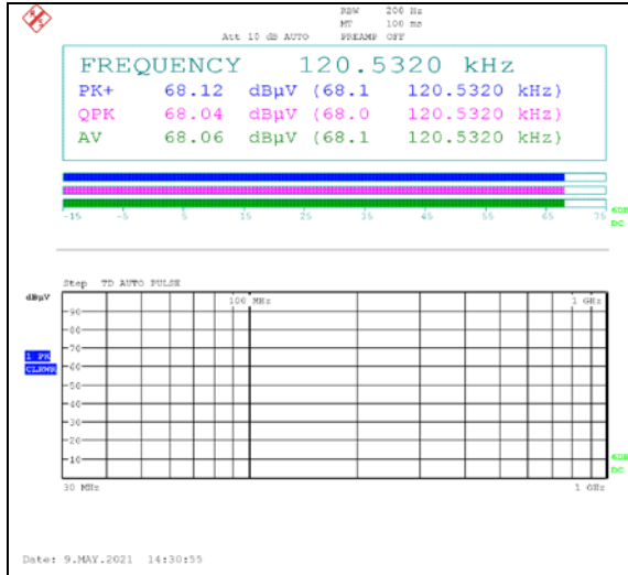
Ant. 2 (120.5 kHz)
