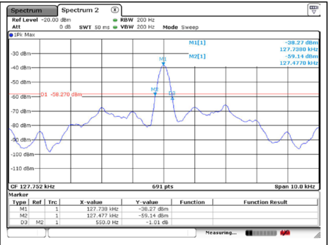
Ant. 2 (126.7 ~ 128.7 kHz)
