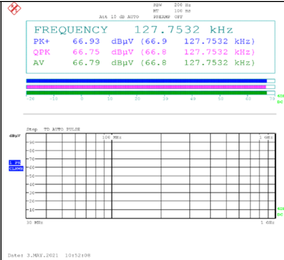
Ant. 2 (126.7 ~ 128.7 kHz)
