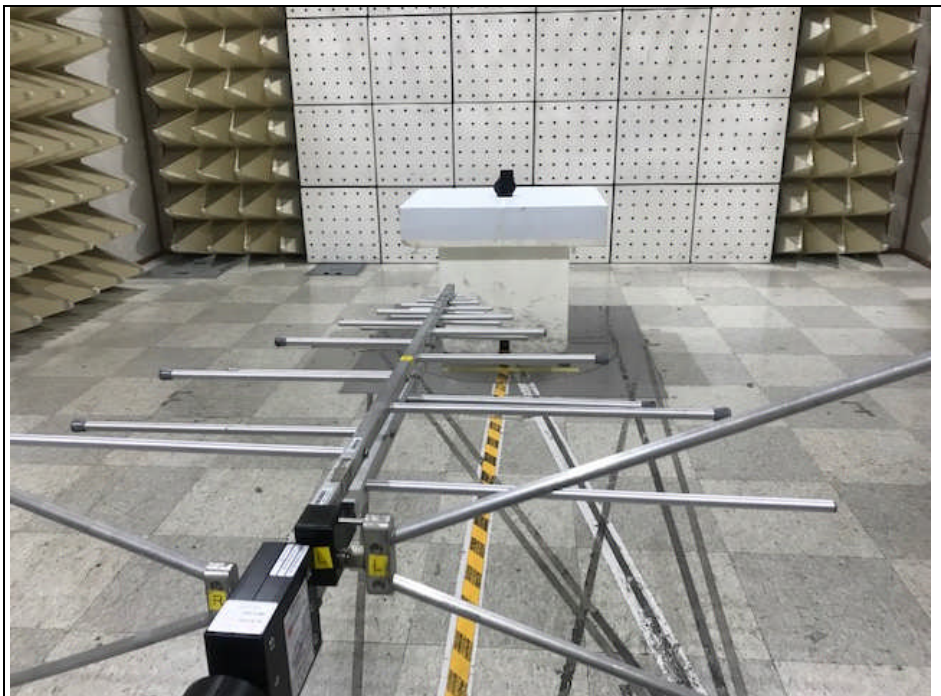
Photo of Test Set up (30 MHz ~ 1 000 MHz)
