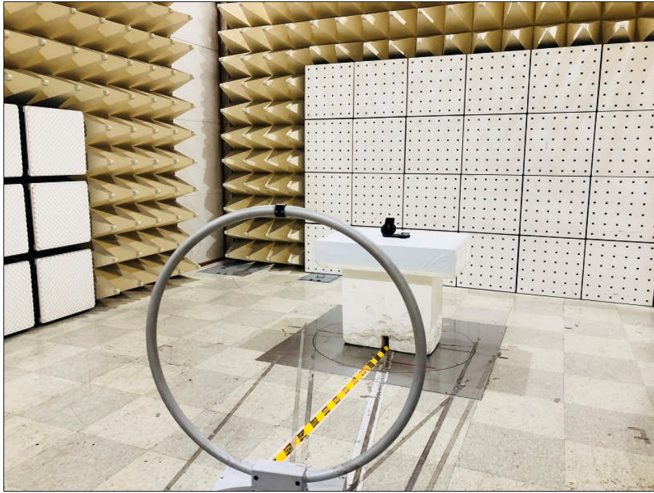
Photo of Test Set up (9 kHz ~ 30 MHz)
