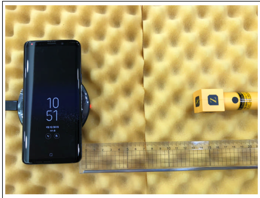
Photo of MPE Test Set up (E-field)
