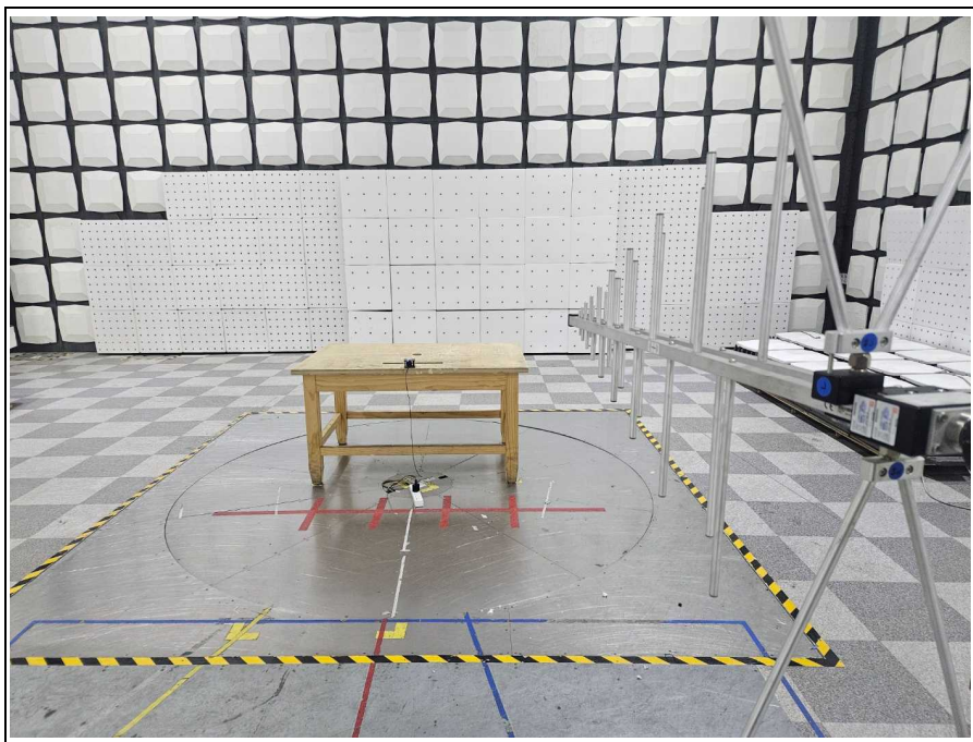
Photo of Radiated Spurious Emission Test (Above 30 MHz)
