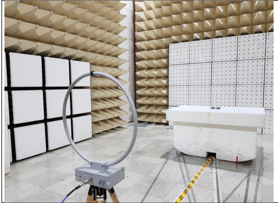
Photo of Test Set up (9 kHz ~ 30 MHz)
