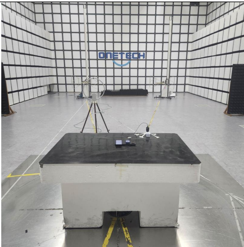
Below 30 MHz_Phoen+Buds_B-H
