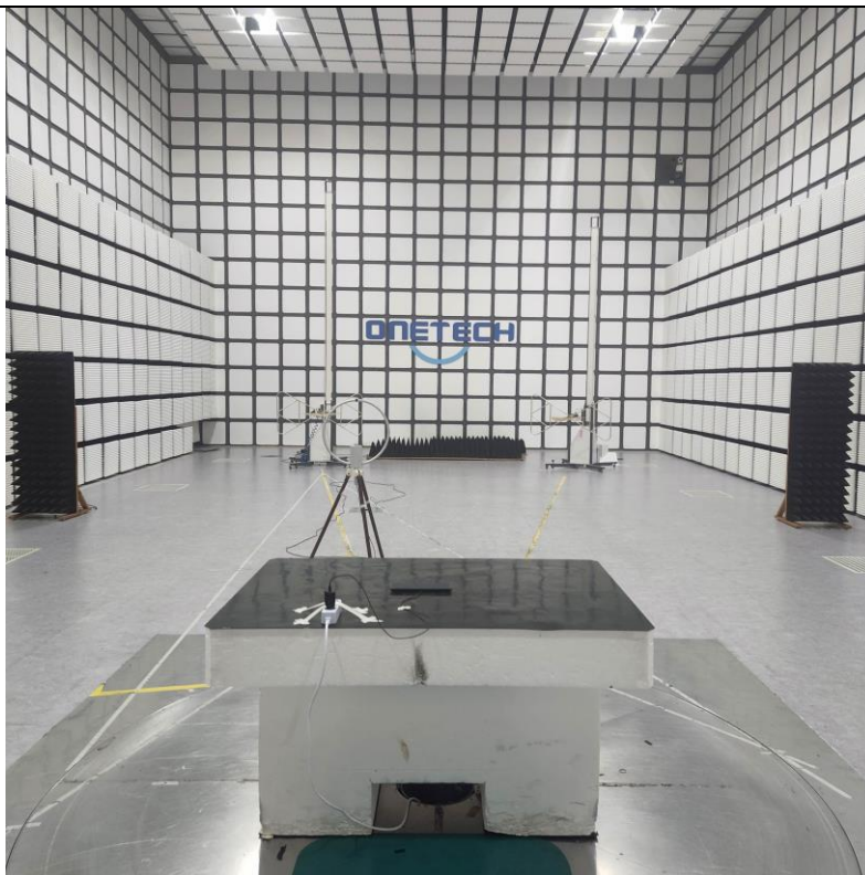
Below 30 MHz_idel_F-H
