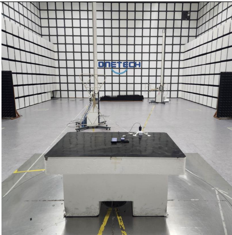
Above 30 MHz_Phone+Buds_B-V
