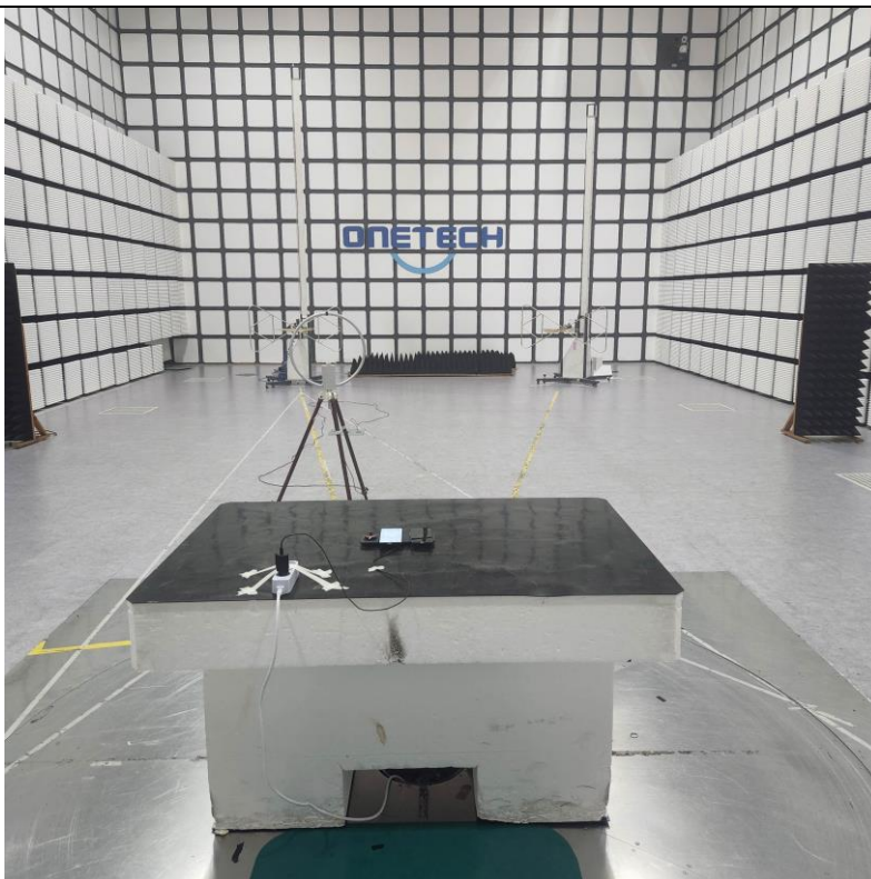
Below 30 MHz_Phone+Phone_F-H
