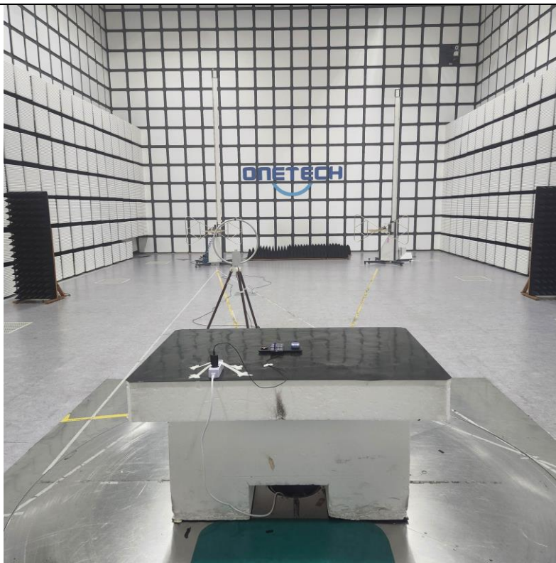
Below 30 MHz_Phoen+Buds_F-H
