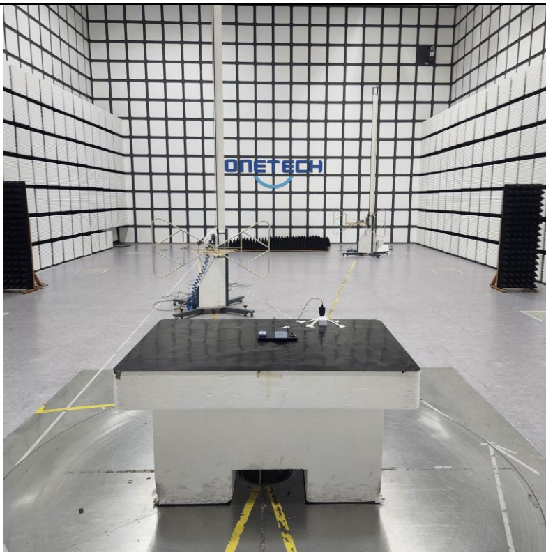
Above 30 MHz_Buds+Phone_B-H
