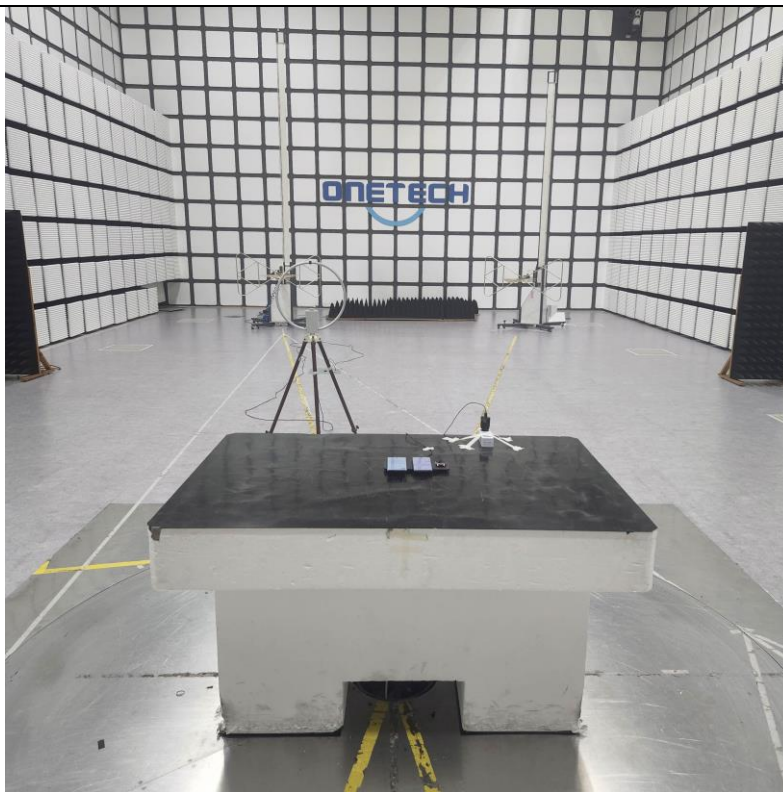
Below 30 MHz_Phone+Phone_B-H
