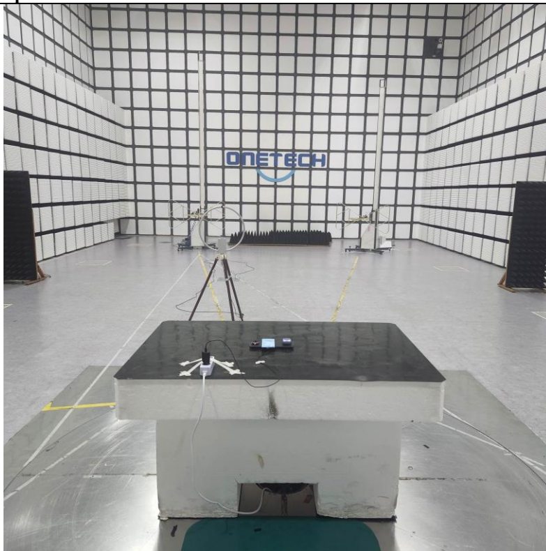
Below 30 MHz_Buds+Phone_F-H
