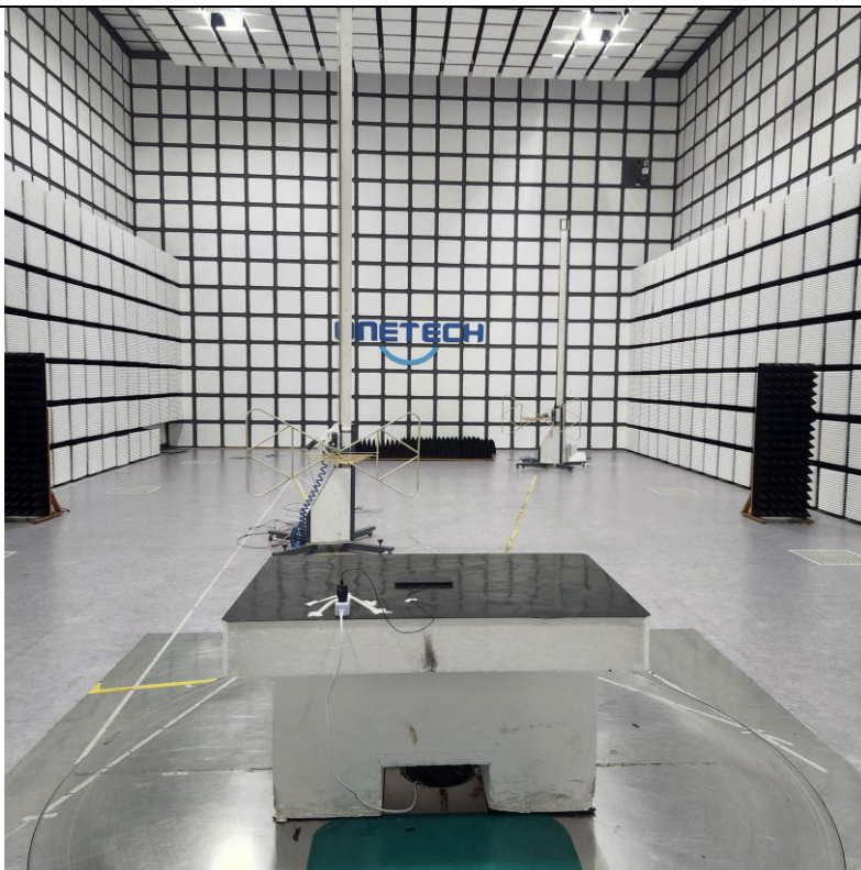
Above 30 MHz_Idle_F-H
