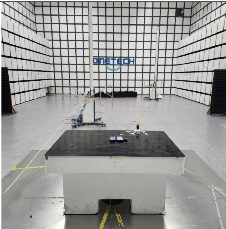
Above 30 MHz_Phone+Phone_B-H
