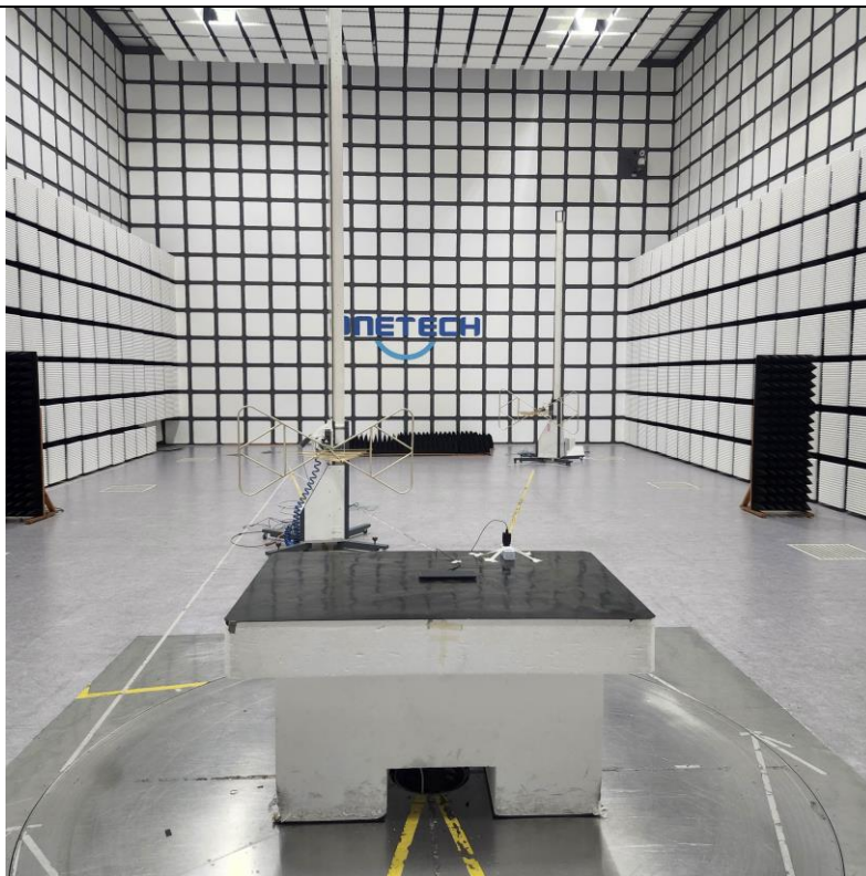
Above 30 MHz_Idle_B-H
