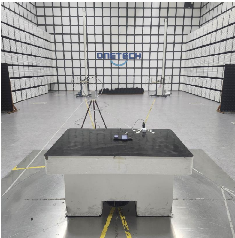
Below 30 MHz_Phone+Buds_B-H
