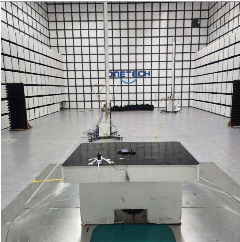
Above 30 MHz_Phone+Phone_F-V
