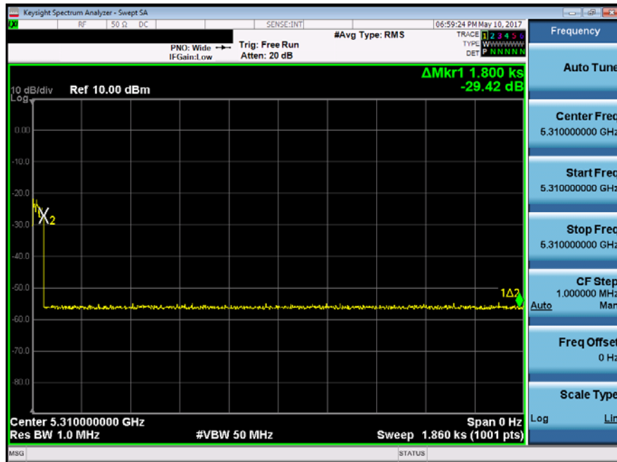
Plot 5-19. Band 2A Non-Occupancy Period - Monitoring Live Spectrum Elapsed time - 30 minutes
