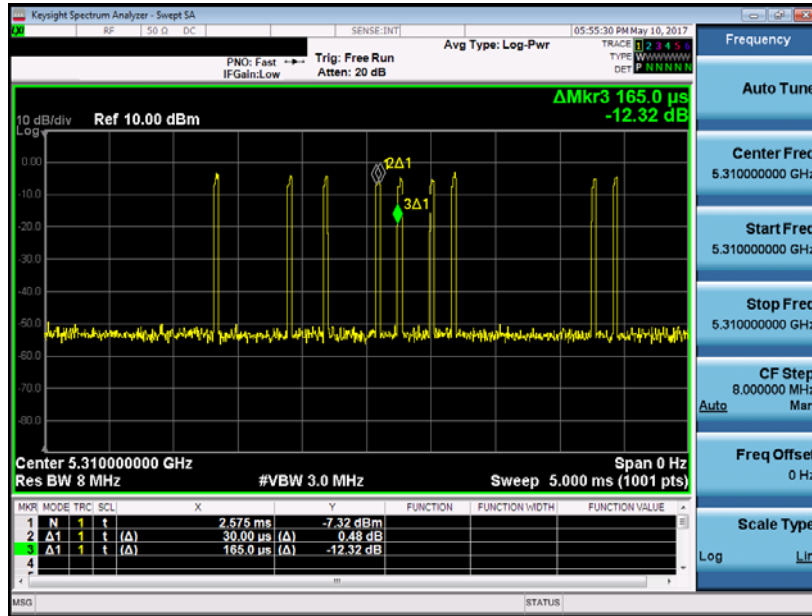
Plot 5-9. Band 2A Pulse Width / Period
