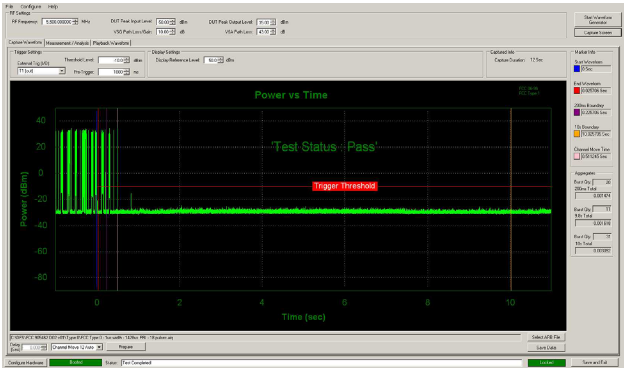
Plot 5-18. Band 2C Channel Move Time and Aggregate Time
