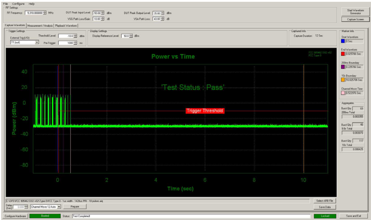
Plot 5-17. Band 2A Channel Move Time and Aggregate Time
