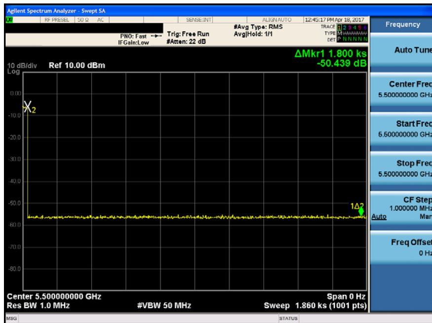
Plot 5-20. Band 2C Non-Occupancy Period - Monitoring Live Spectrum Elapsed time - 30 minutes
