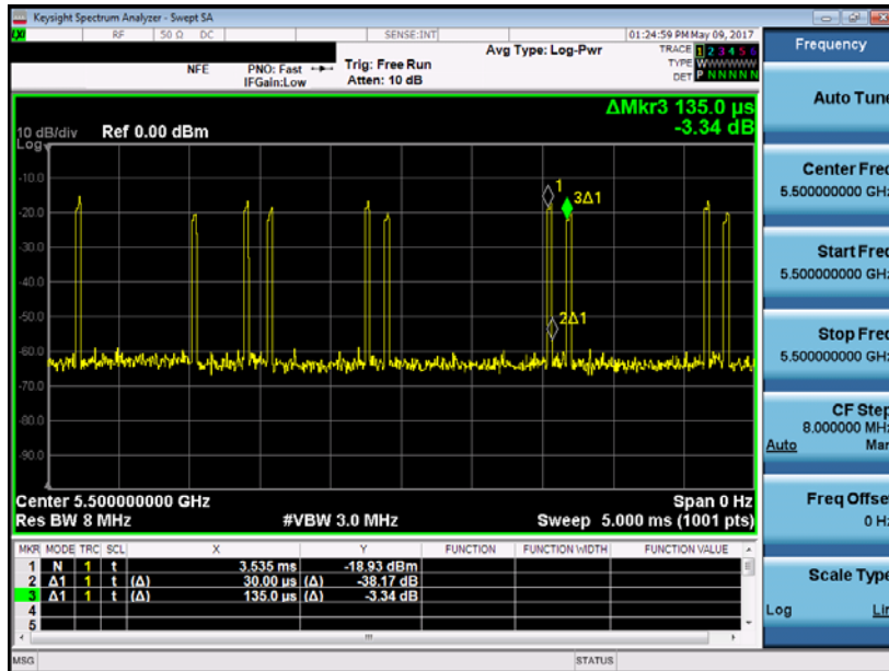
Plot 5-10. Band 2C Pulse Width / Period
