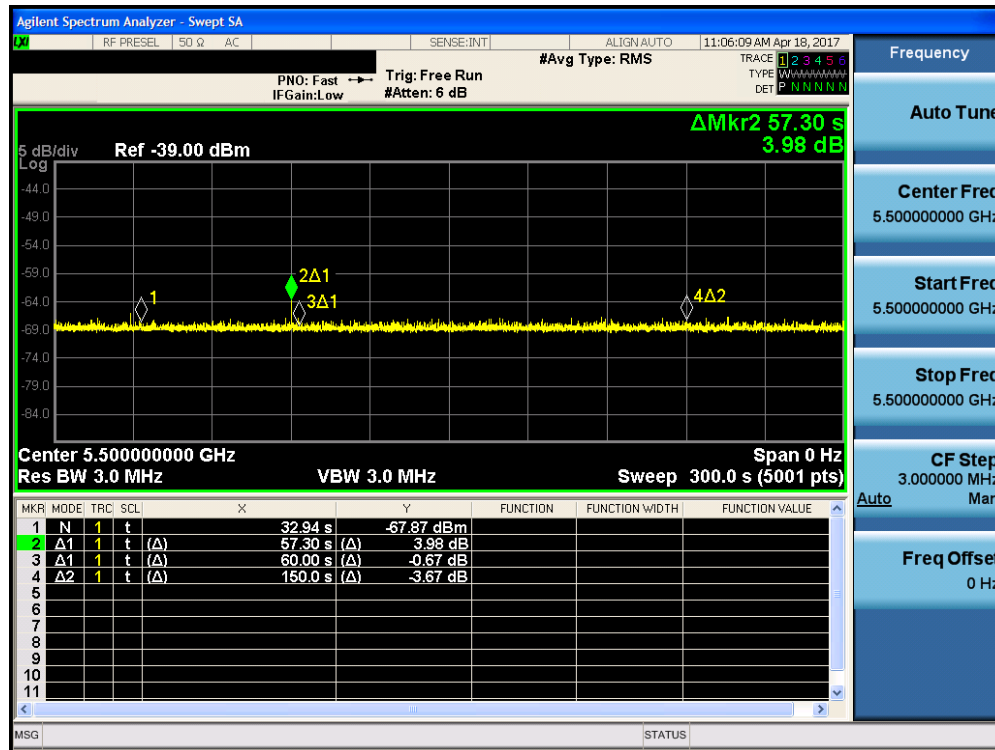
Plot 5-16. Radar Burst at End of CAC Time
