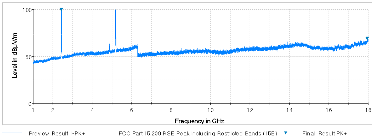
Plot 7-90. Radiated Spurious Plot above 1GHz (2.4GHz – 5GHz, Ant. Pol. V)
