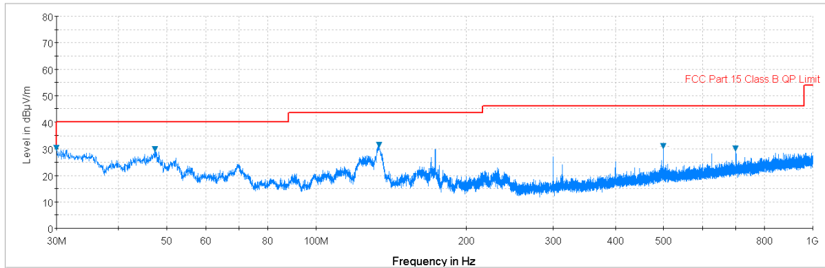
Plot 7-133. Radiated Spurious Plot below 1GHz (802.11a – U3 Ch. 157, Ant. Pol. H)
