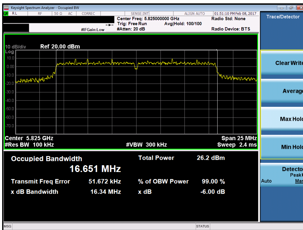
Plot 7-21. 6dB Bandwidth Plot (802.11a (UNII Band 3) – Ch. 165)
