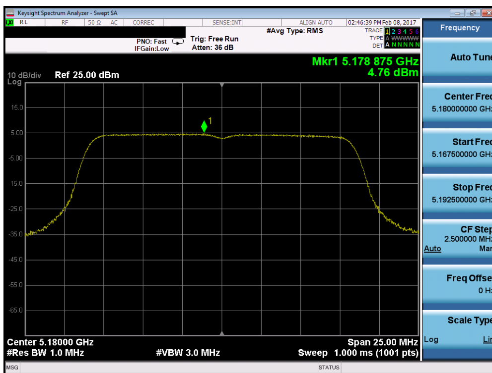
Plot 7-55. Power Spectral Density Plot (802.11a (UNII Band 1) – Ch. 36)
