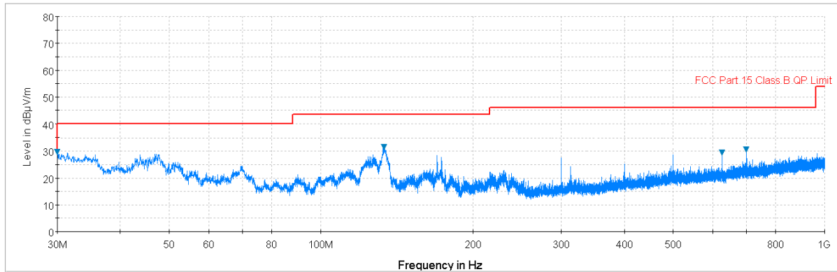
Plot 7-131. Radiated Spurious Plot below 1GHz (802.11a – U3 Ch. 157, Ant. Pol. H)
