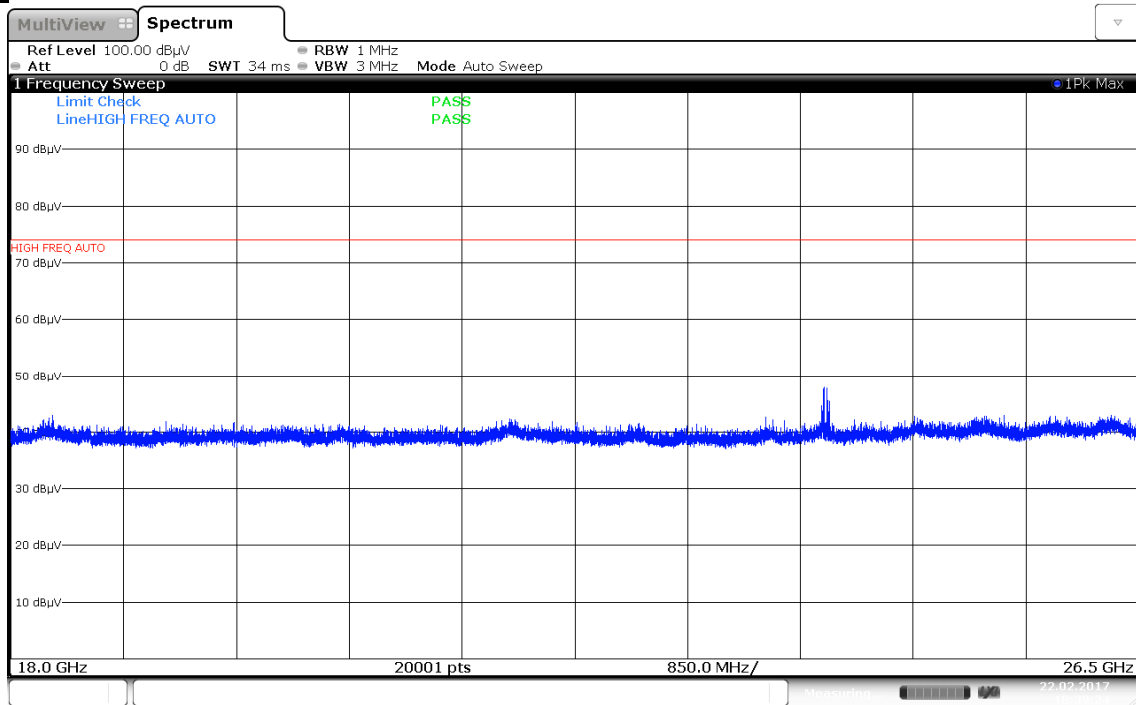
Plot 7-85. Radiated Spurious Plot above 18GHz - 26.5GHz (802.11a – Ant. Pol. H)
