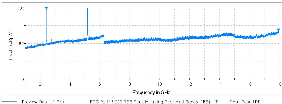
Plot 7-89. Radiated Spurious Plot above 1GHz (2.4GHz – 5GHz, Ant. Pol. H)
