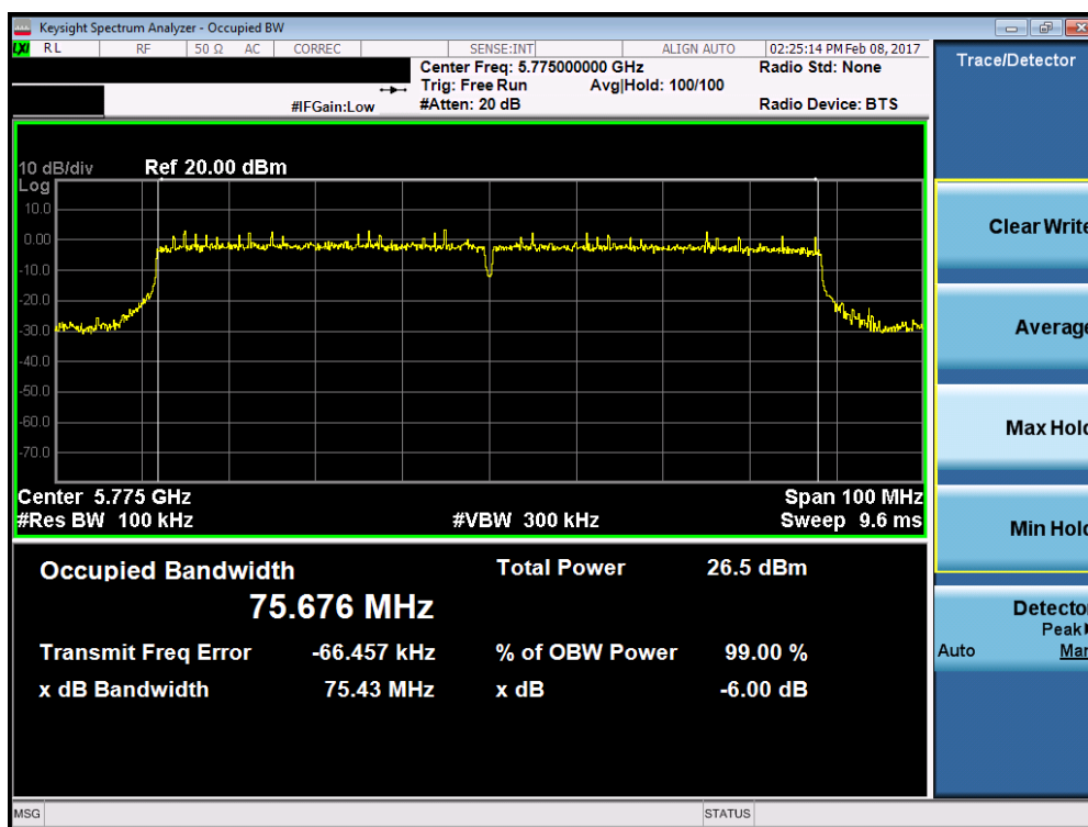
Plot 7-27. 6dB Bandwidth Plot (80MHz BW 802.11ac (UNII Band 3) – Ch. 155)
