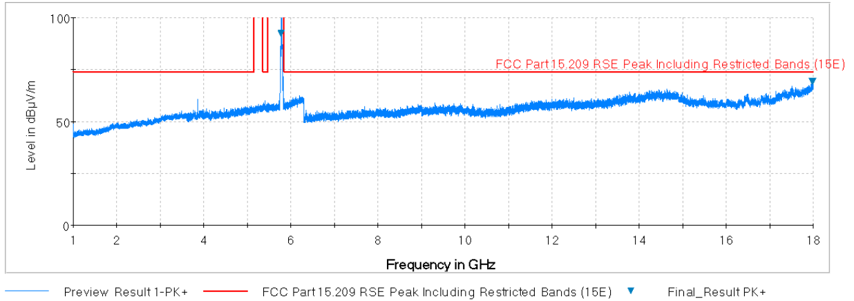
Plot 7-84. Radiated Spurious Plot above 1GHz (802.11a – U3 Ch. 157, Ant. Pol. V)
