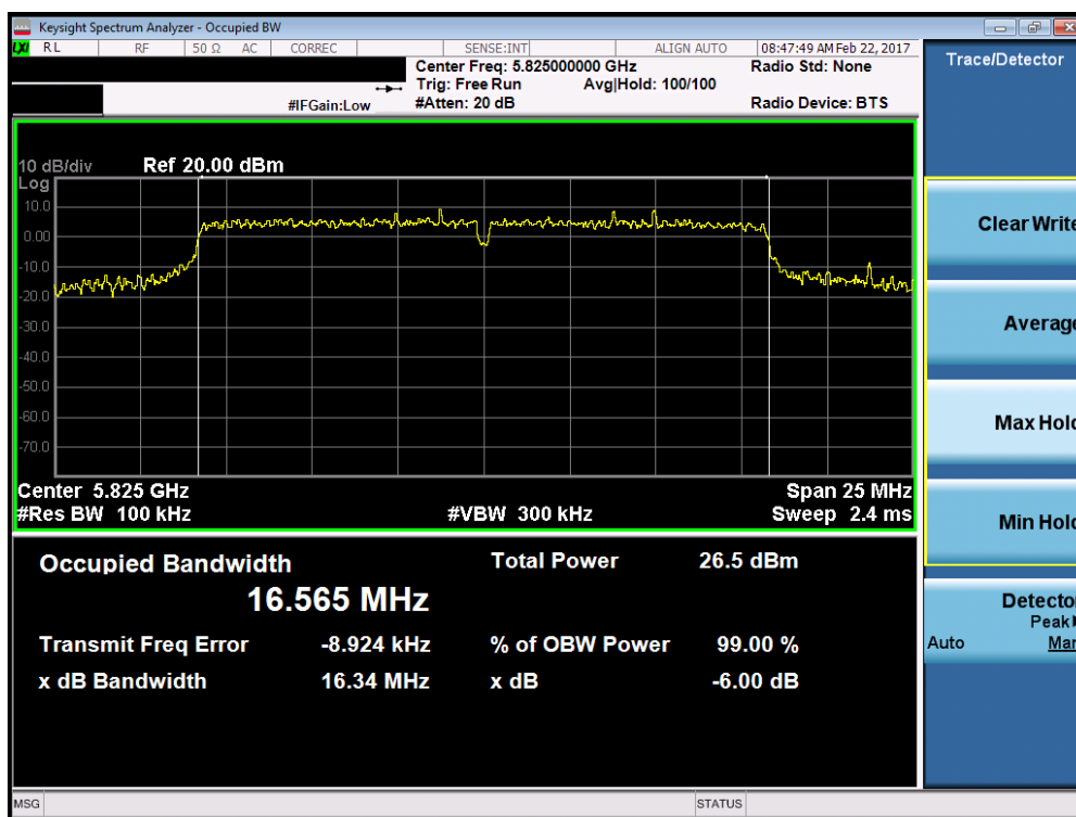
Plot 7-30. 6dB Bandwidth Plot (802.11a (UNII Band 3) – Ch. 165)
