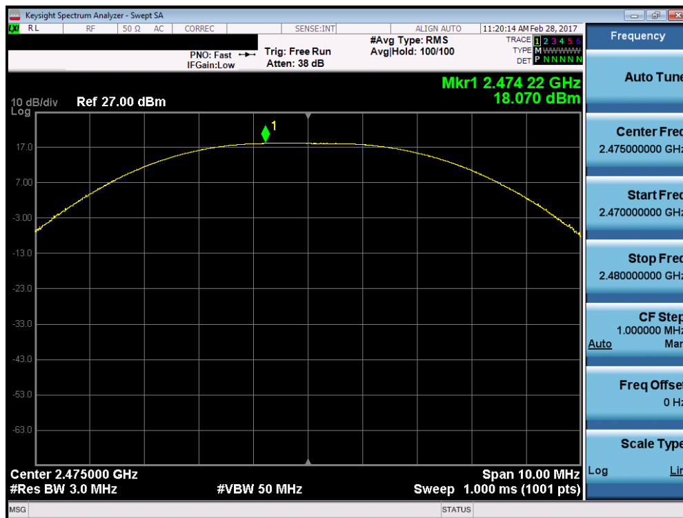
Plot 7-6. Peak Conducted Power (ZigBee – Ch. 25)
