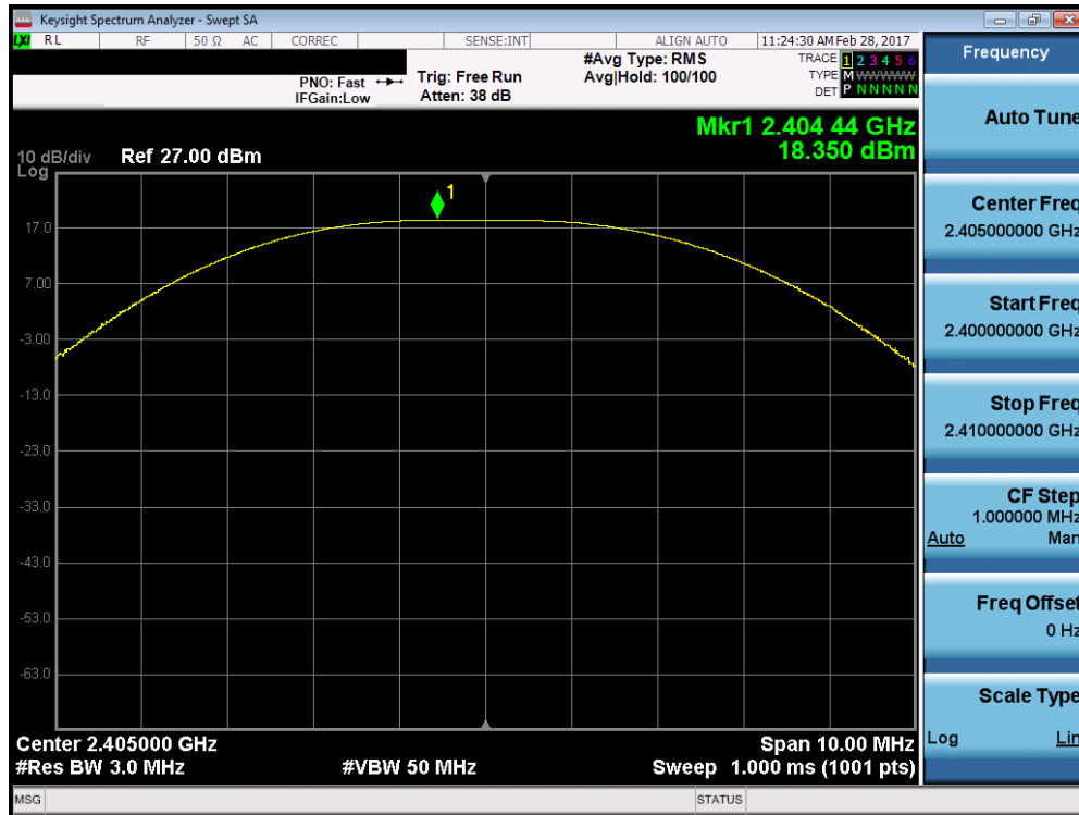
Plot 7-4. Peak Conducted Power (ZigBee – Ch. 11)
