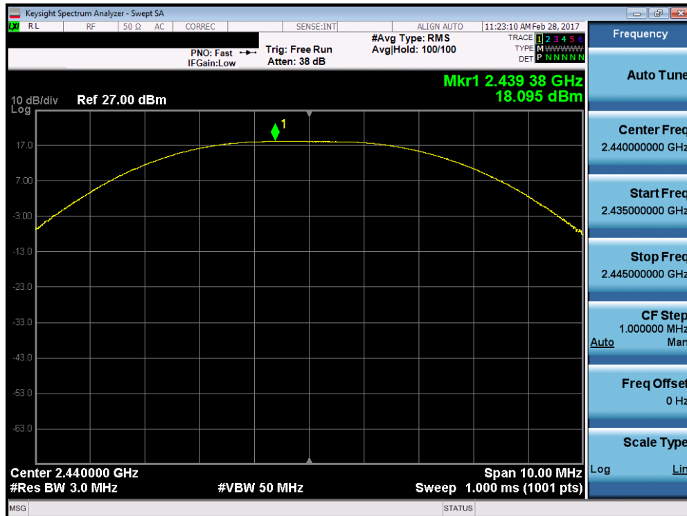
Plot 7-5. Peak Conducted Power (ZigBee – Ch. 18)
