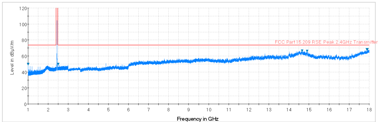
Plot 7-23. Radiated Spurious Plot above 1GHz (Zigbee – Ch. 18, Ant. Pol. H)
