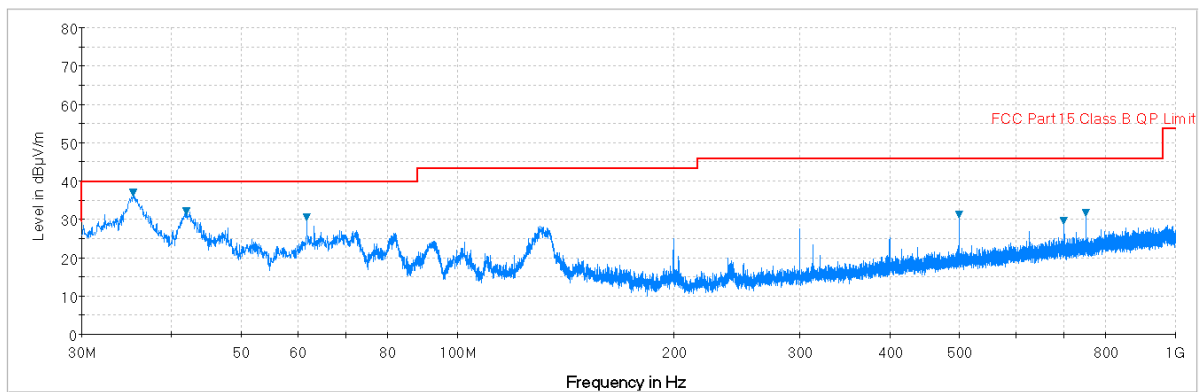
Plot 7-34. Radiated Spurious Plot below 1GHz (Pol. V)
