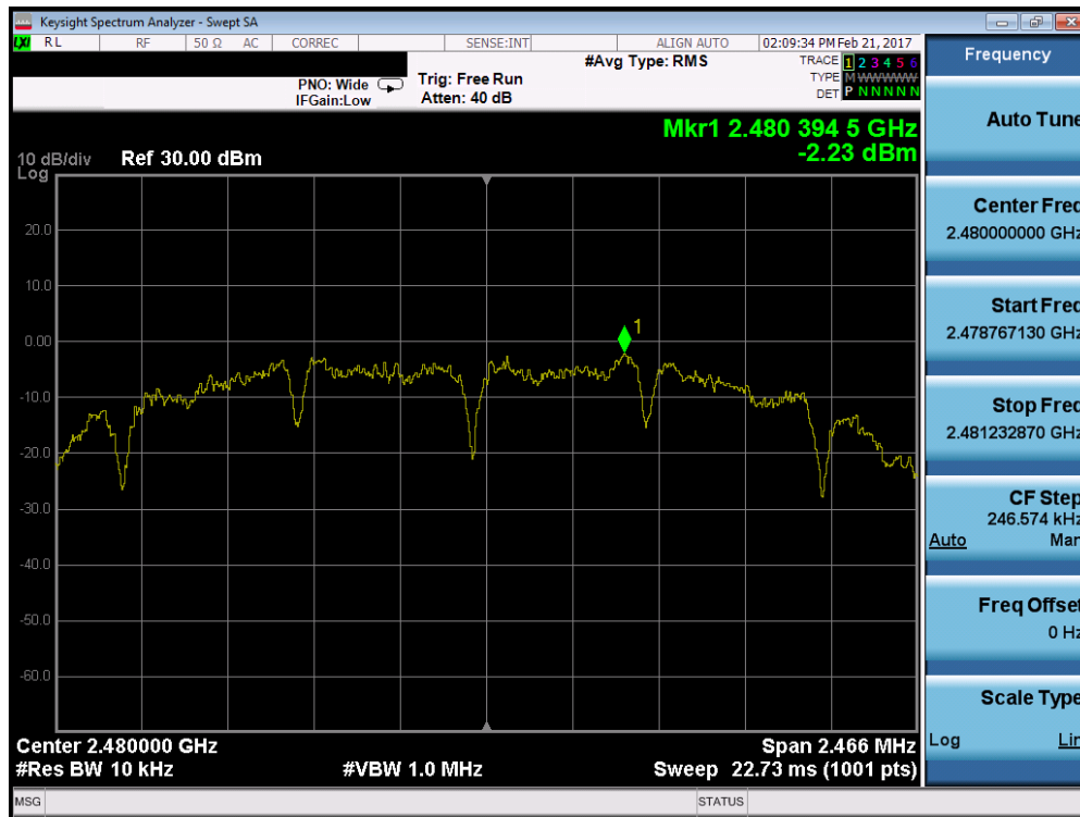
Plot 7-11. Power Spectral Density Plot (ZigBee – Ch. 26)
