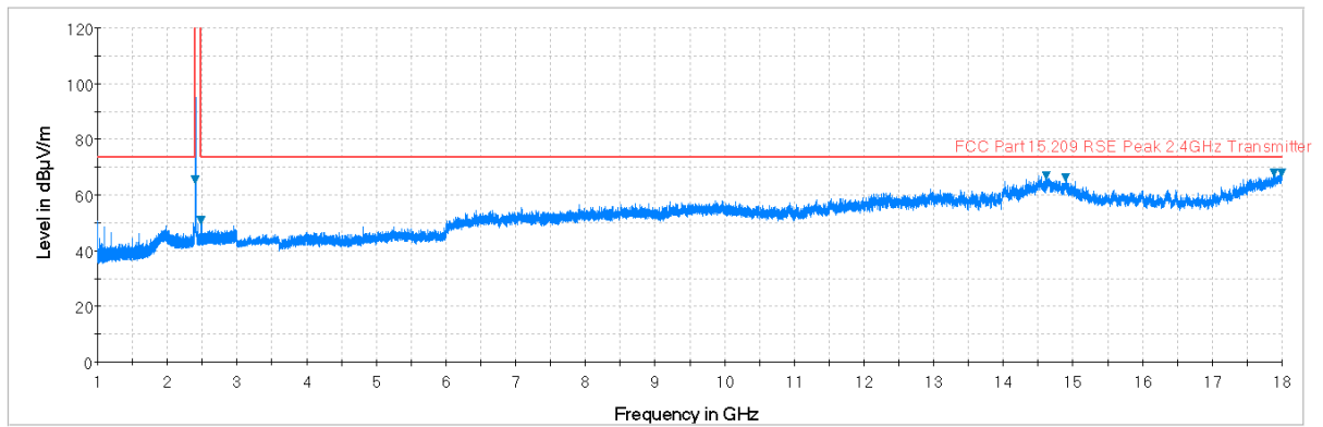
Plot 7-22. Radiated Spurious Plot above 1GHz (Zigbee – Ch. 11, Ant. Pol. V)
