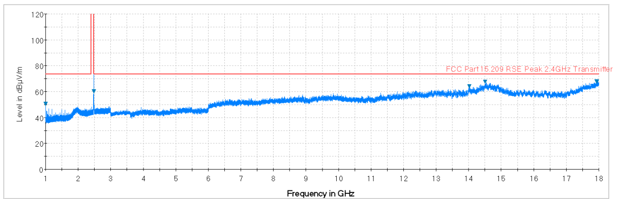
Plot 7-25. Radiated Spurious Plot above 1GHz (Zigbee – Ch. 26, Ant. Pol. H)
