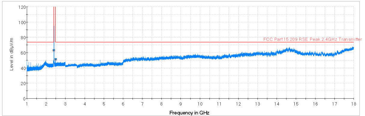
Plot 7-21. Radiated Spurious Plot above 1GHz (Zigbee – Ch. 11, Ant. Pol. H)
