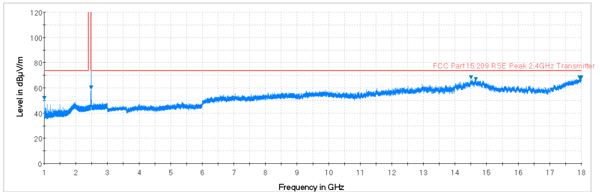
Plot 7-26. Radiated Spurious Plot above 1GHz (Zigbee – Ch. 26, Ant. Pol. V)
