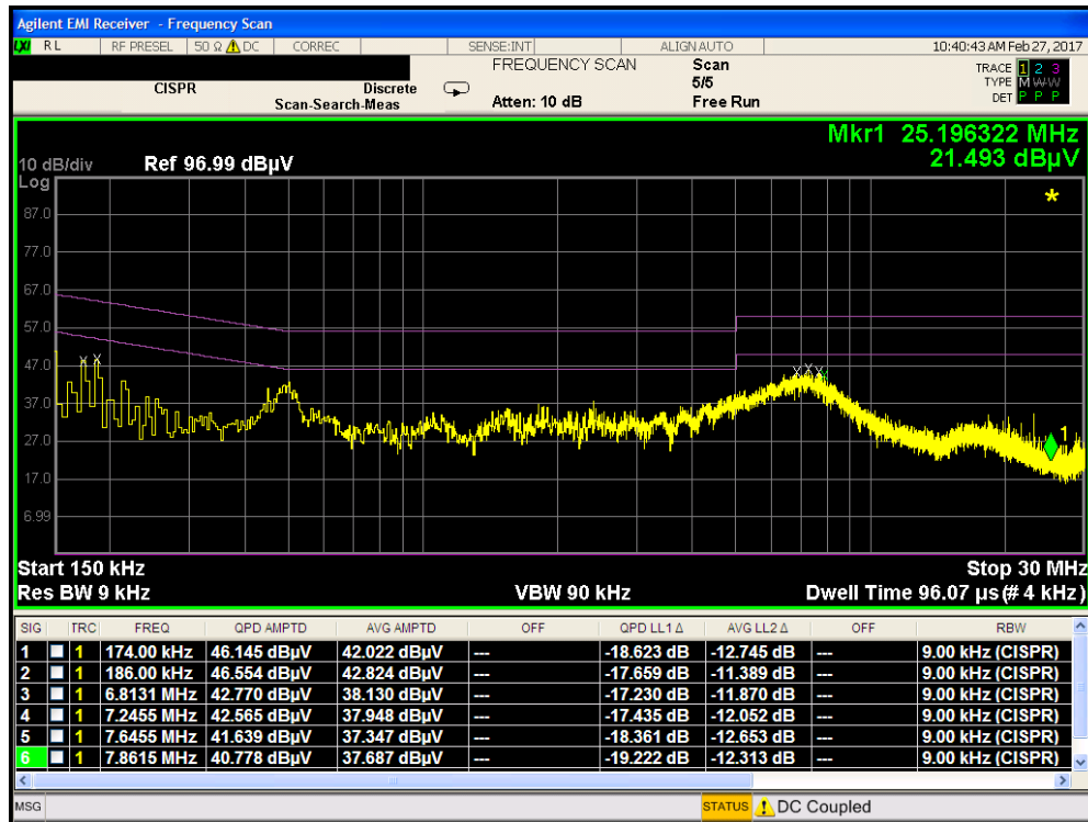
Plot 7-35. Line-Conducted Test Plot (L1)
