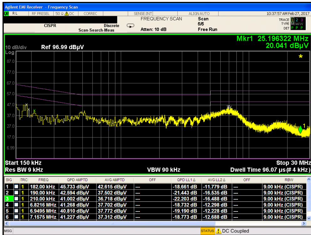
Plot 7-36. Line-Conducted Test Plot (N)
