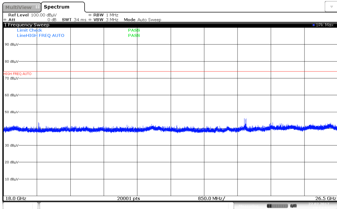
Plot 7-28. Radiated Spurious Plot above 18GHz (Pol. V)
