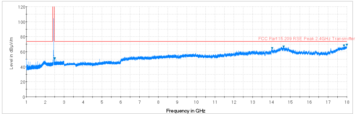
Plot 7-24. Radiated Spurious Plot above 1GHz (Zigbee – Ch. 18, Ant. Pol. V)
