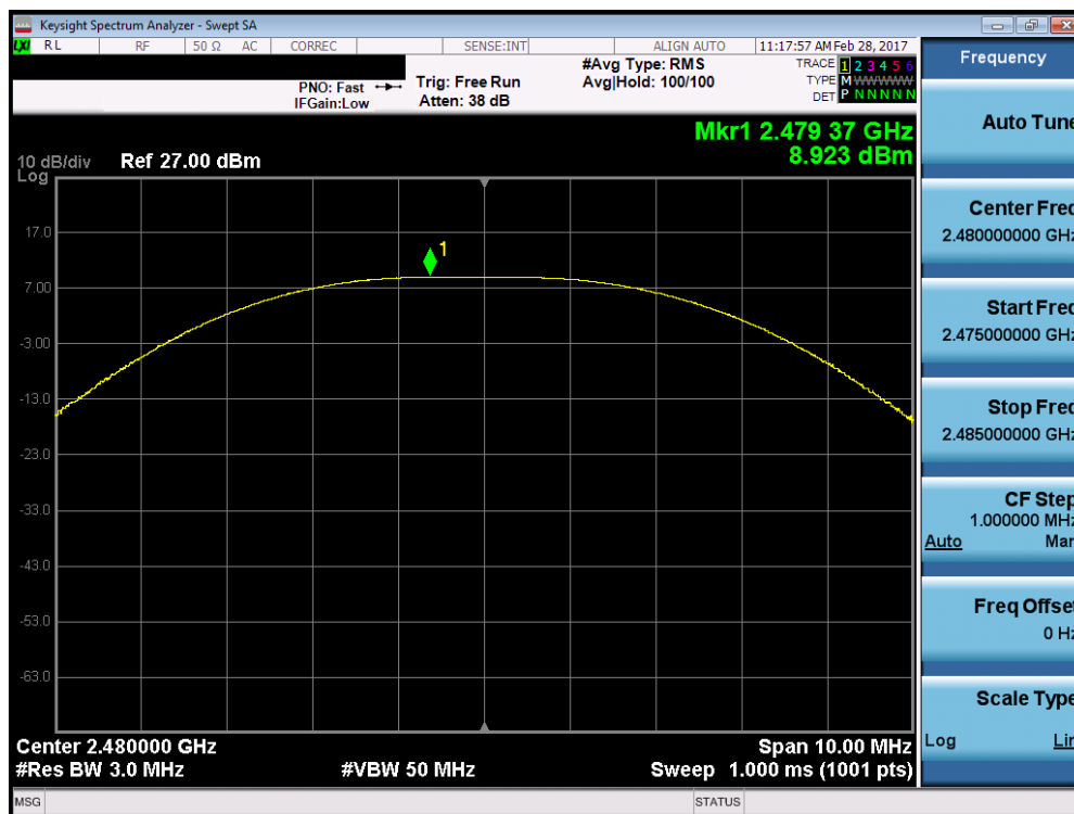
Plot 7-7. Peak Conducted Power (ZigBee – Ch. 26)
