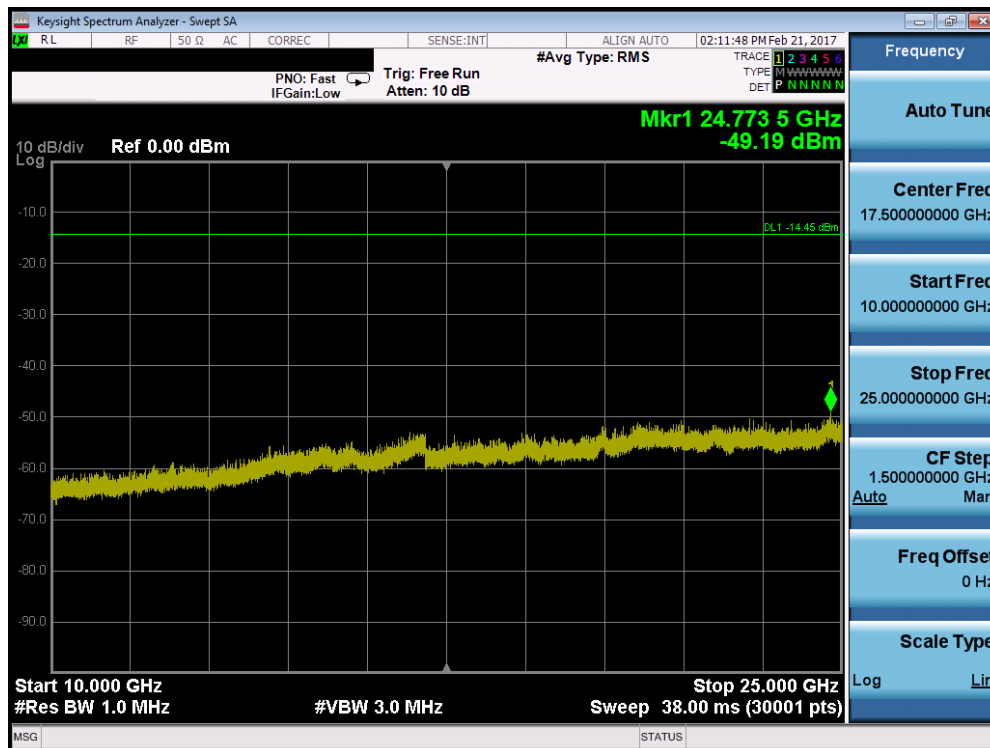
Plot 7-20. Conducted Spurious Plot (ZigBee – Ch. 25)
