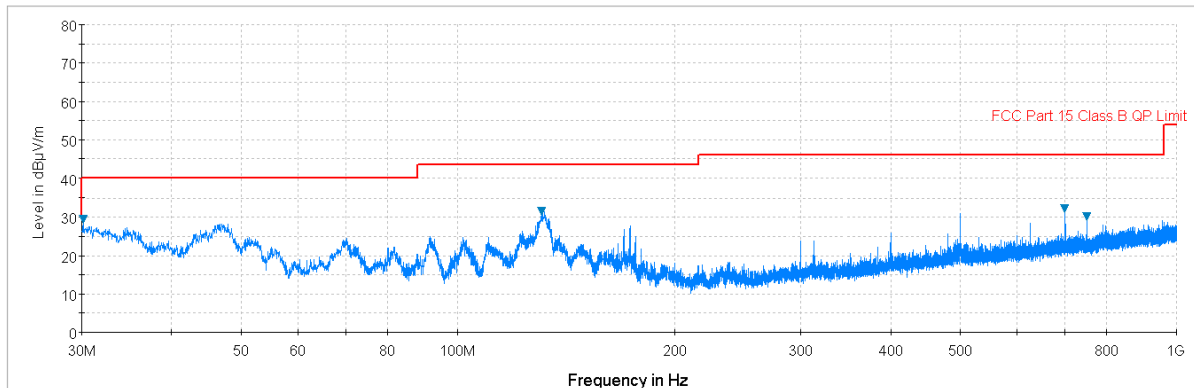
Plot 7-33. Radiated Spurious Plot below 1GHz (Pol. H)
