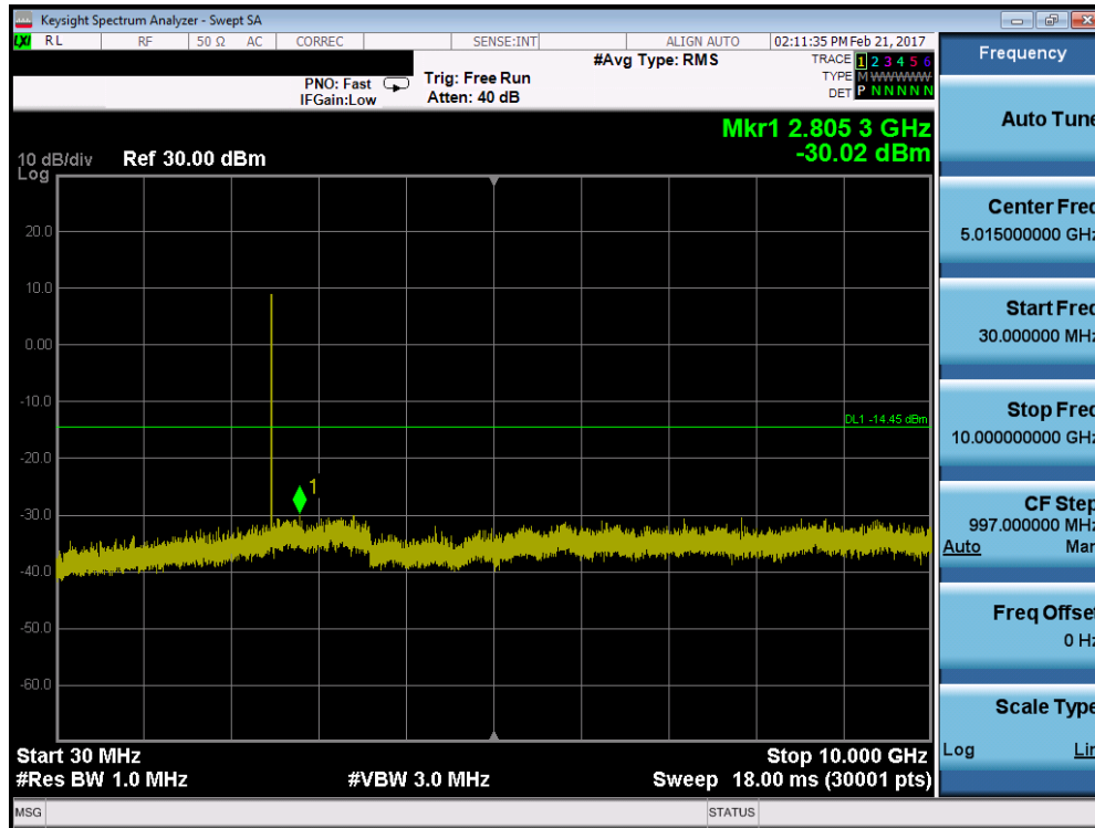
Plot 7-19. Conducted Spurious Plot (ZigBee – Ch. 25)
