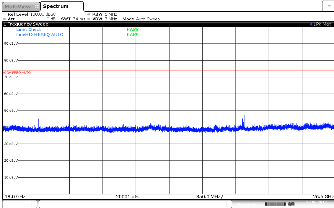
Plot 7-27. Radiated Spurious Plot above 18GHz (Pol. H)
