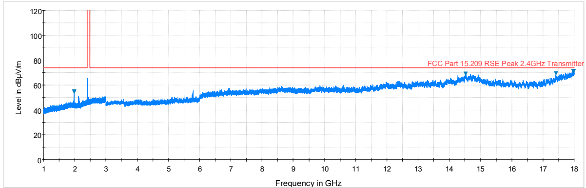
Plot 7-5. Radiated Pre-Scan Plot at 3-meters above 1 GHz (Ant. Pol. H)
