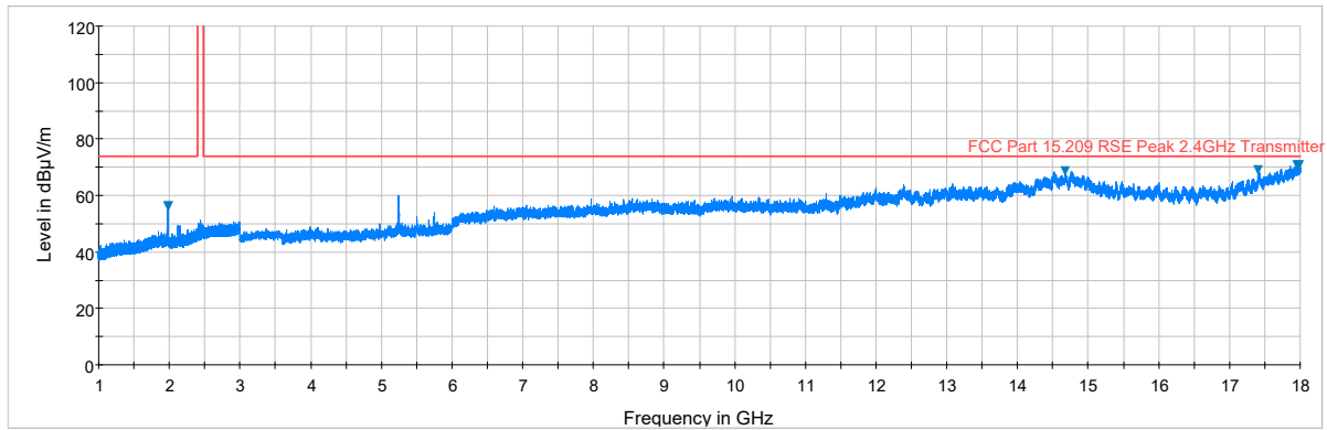
Plot 7-6. Radiated Pre-Scan Plot at 3-meters above 1 GHz (Ant. Pol. V)
