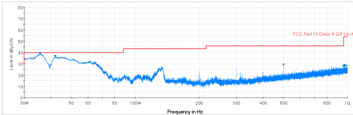
Plot 7-132. Radiated Spurious Plot below 1GHz (802.11a – U3 Ch. 157, Ant. Pol. V)
