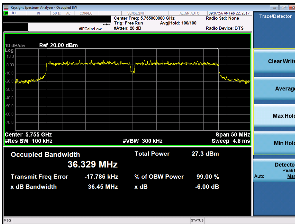
Plot 7-34. 6dB Bandwidth Plot (40MHz BW 802.11n (UNII Band 3) – Ch. 151)
