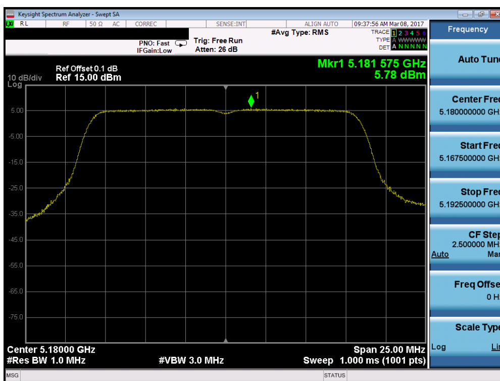
Plot 7-37. Power Spectral Density Plot (802.11a (UNII Band 1) – Ch. 36)
