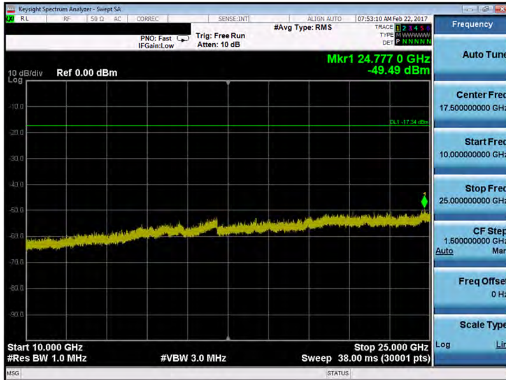
Plot 7-72. Conducted Spurious Plot (802.11b – Ch. 1)
