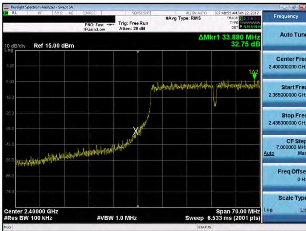
Plot 7-63. Band Edge Plot (40MHz 802.11n/ac – Ch. 3)
