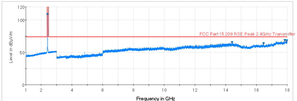
Plot 7-85. Radiated Spurious Plot above 1GHz (802.11b – Ch. 1, Ant. Pol. H)
