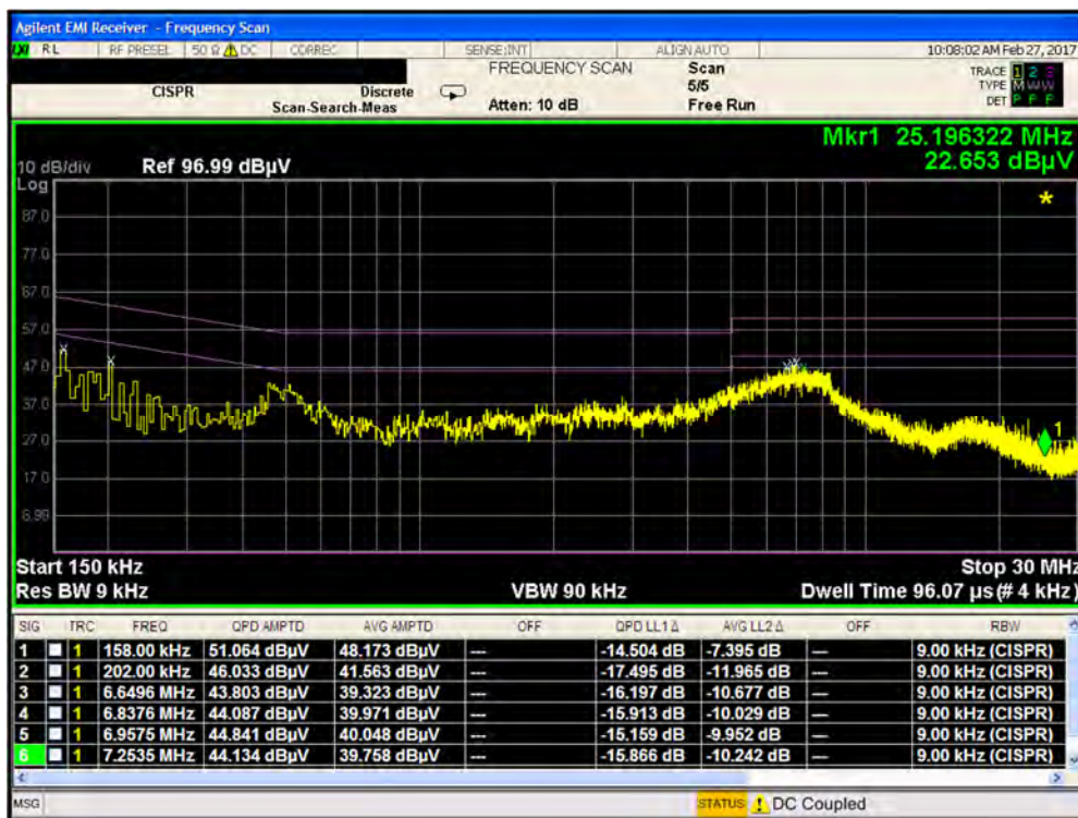
Plot 7-121. Line Conducted Plot with 802.11b (L1)
