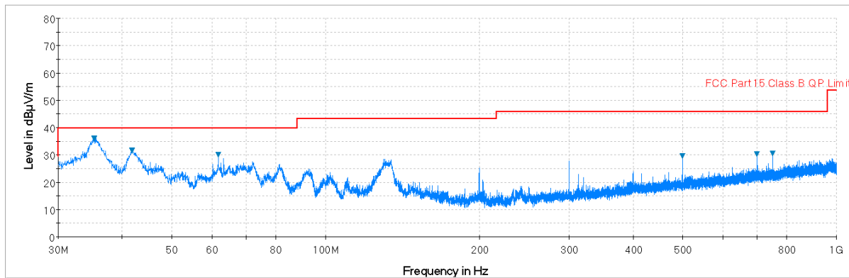
Plot 7-118. Radiated Spurious Plot below 1GHz (Pol. V)
