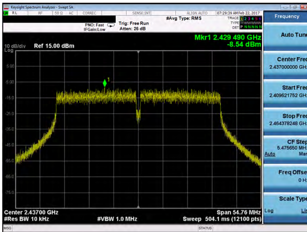
Plot 7-44. Power Spectral Density Plot (40MHz 802.11 n/ac – Ch. 6)
