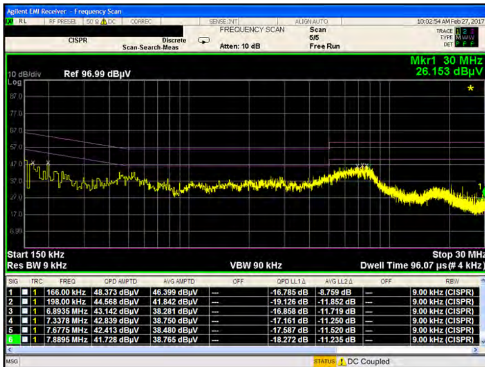
Plot 7-122. Line Conducted Plot with 802.11b (N)
