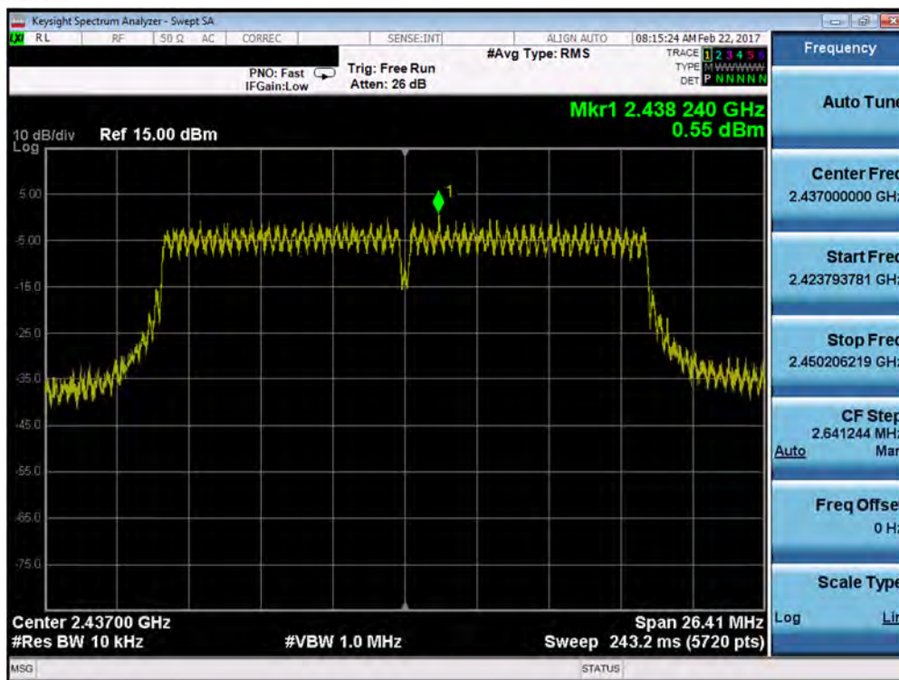
Plot 7-41. Power Spectral Density Plot (802.11n (2.4GHz) – Ch. 6)
