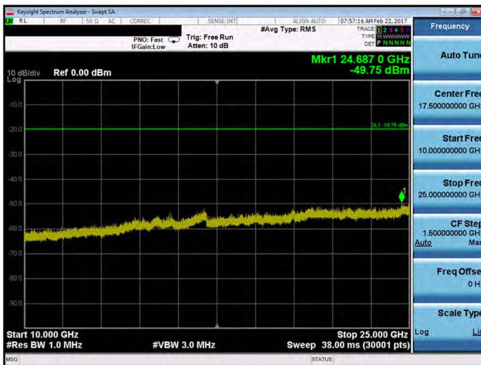
Plot 7-76. Conducted Spurious Plot (802.11b – Ch. 11)
