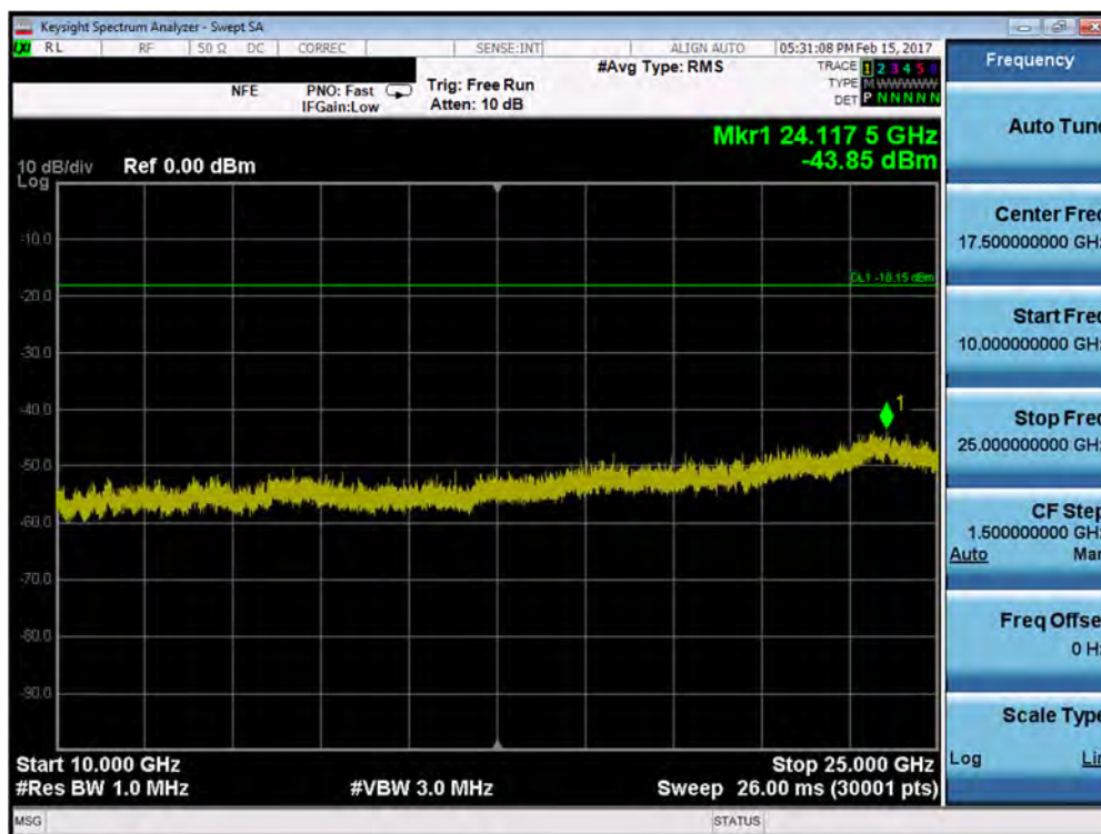
Plot 7-70. Conducted Spurious Plot (802.11b – Ch. 11)
