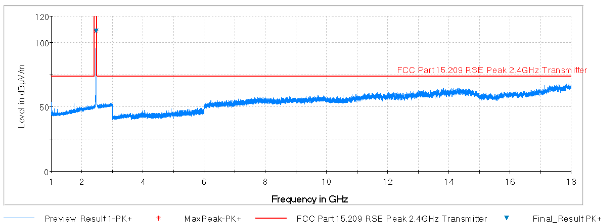
Plot 7-89. Radiated Spurious Plot above 1GHz (802.11b – Ch. 11, Ant. Pol. H)
