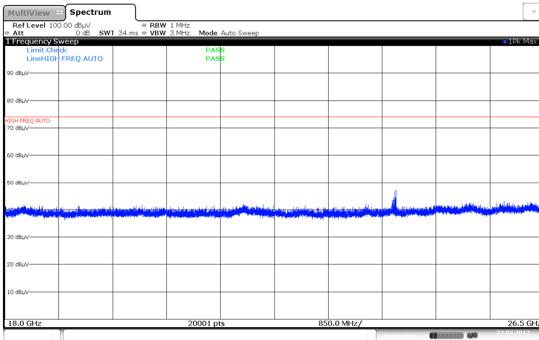
Plot 7-92. Radiated Spurious Plot above 18GHz (Pol. V)
