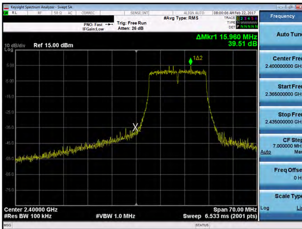
Plot 7-59. Band Edge Plot (20MHz 802.11g– Ch. 1)
