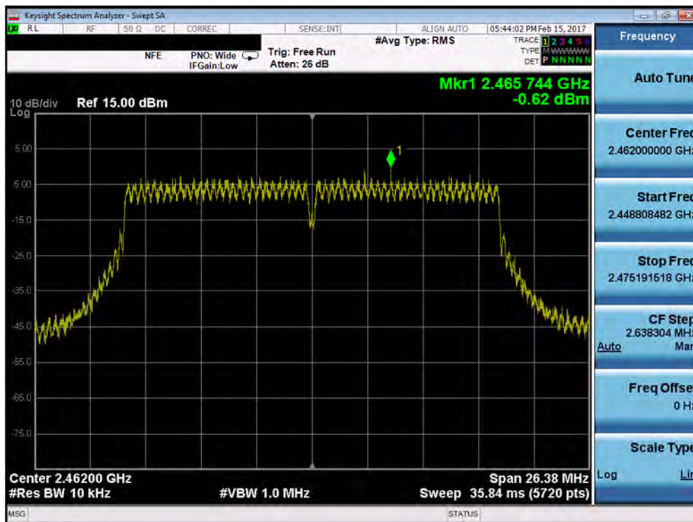
Plot 7-33. Power Spectral Density Plot (802.11n (2.4GHz) – Ch. 11)
