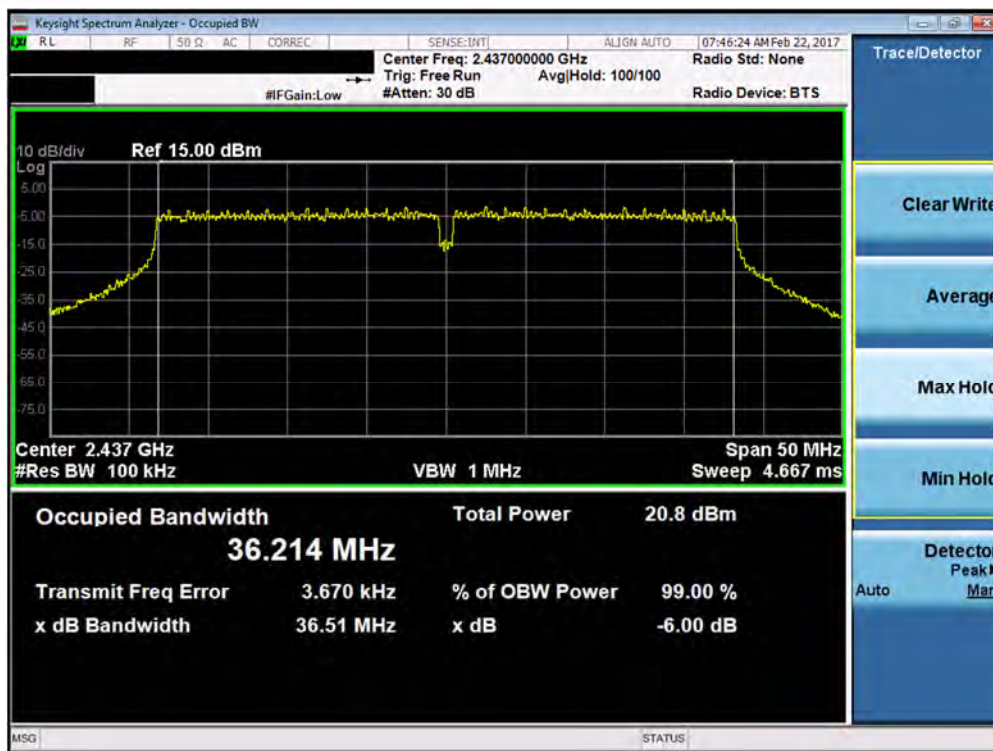
Plot 7-23. 6dB Bandwidth Plot (40MHz 802.11 n/ac – Ch. 6)
