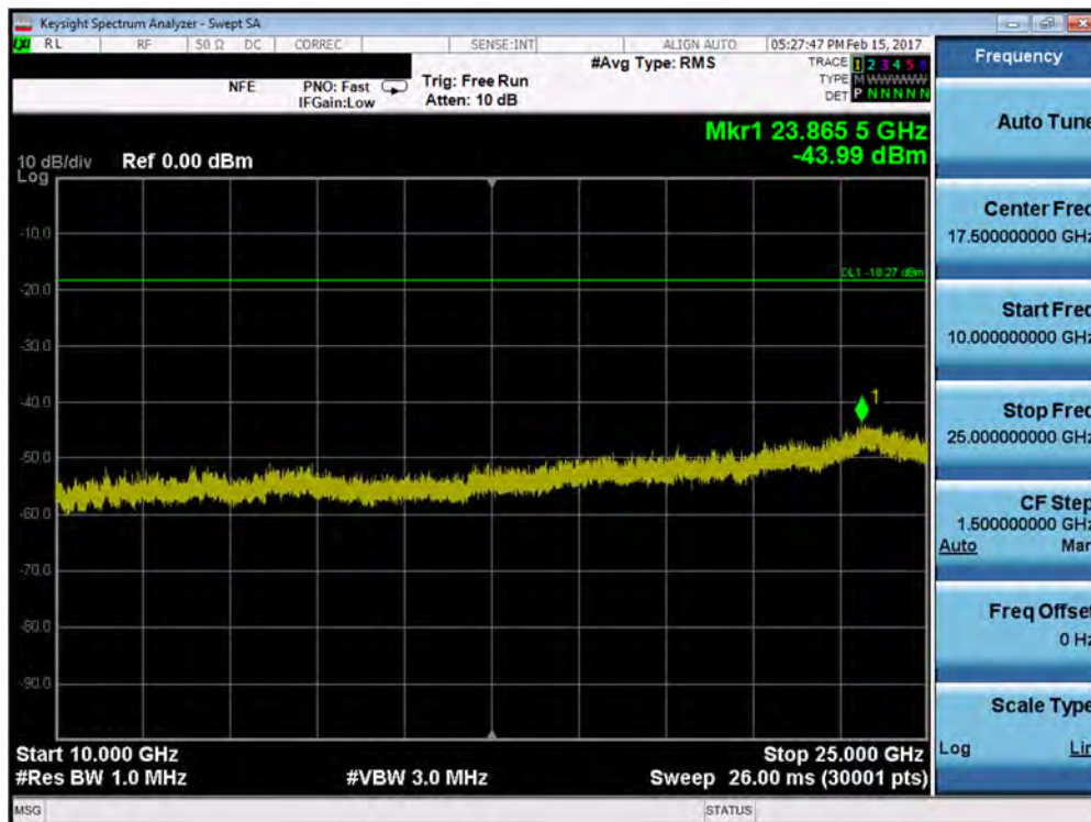
Plot 7-66. Conducted Spurious Plot (802.11b – Ch. 1)
