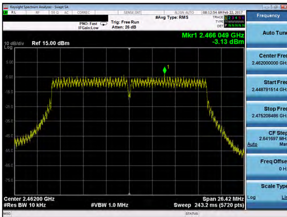
Plot 7-42. Power Spectral Density Plot (802.11n (2.4GHz) – Ch. 11)
