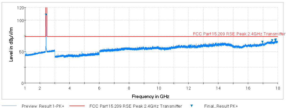
Plot 7-78. Radiated Spurious Plot above 1GHz (802.11b – Ch. 1, Ant. Pol. V)
