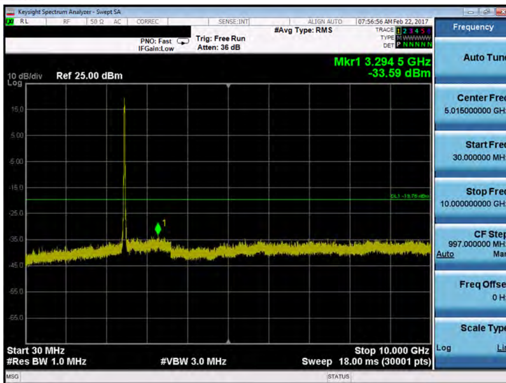
Plot 7-75. Conducted Spurious Plot (802.11b – Ch. 11)
