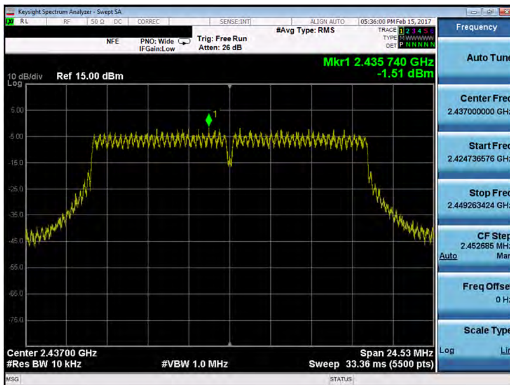
Plot 7-29. Power Spectral Density Plot (802.11g – Ch. 6)
