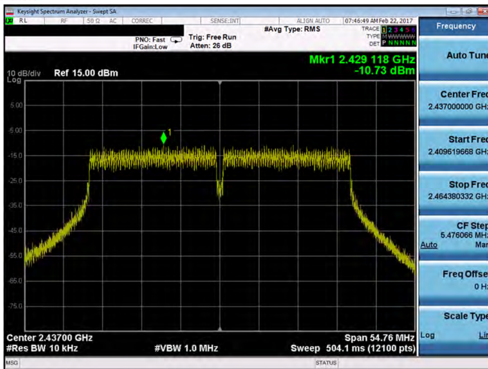
Plot 7-47. Power Spectral Density Plot (40MHz 802.11 n/ac – Ch. 6)
