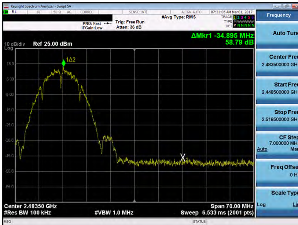
Plot 7-58. Band Edge Plot (20MHz 802.11b – Ch. 11)
