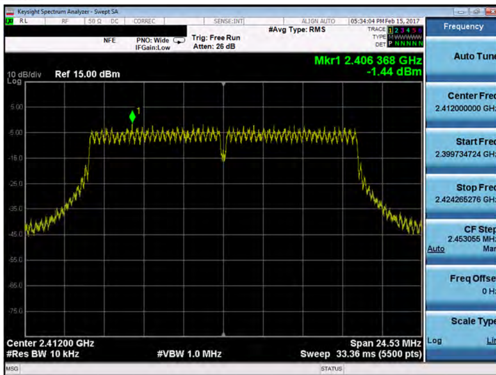
Plot 7-28. Power Spectral Density Plot (802.11g – Ch. 1)
