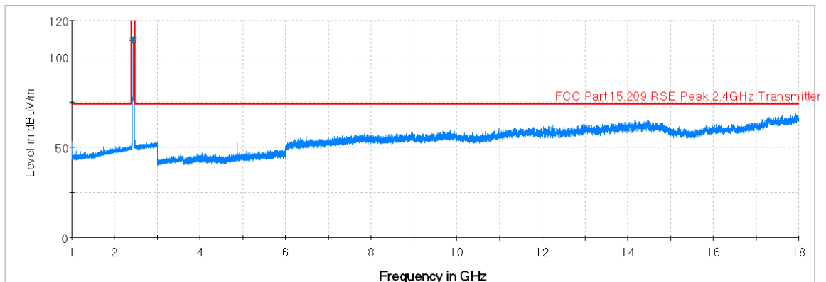
Plot 7-87. Radiated Spurious Plot above 1GHz (802.11b – Ch. 6, Ant. Pol. H)
