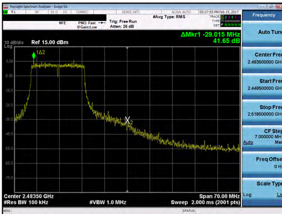
Plot 7-52. Band Edge Plot (20MHz 802.11g – Ch. 11)
