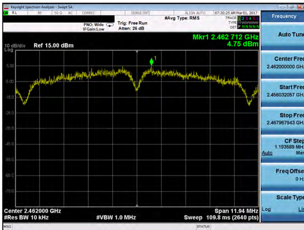
Plot 7-36. Power Spectral Density Plot (802.11b – Ch. 11)
