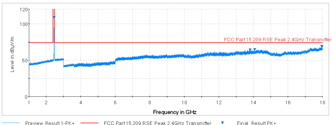
Plot 7-90. Radiated Spurious Plot above 1GHz (802.11b – Ch. 11, Ant. Pol. V)
