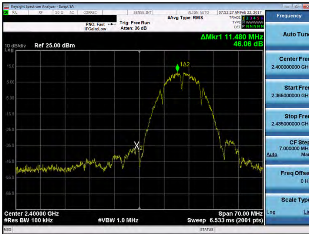
Plot 7-57. Band Edge Plot (20MHz 802.11b – Ch. 1)
