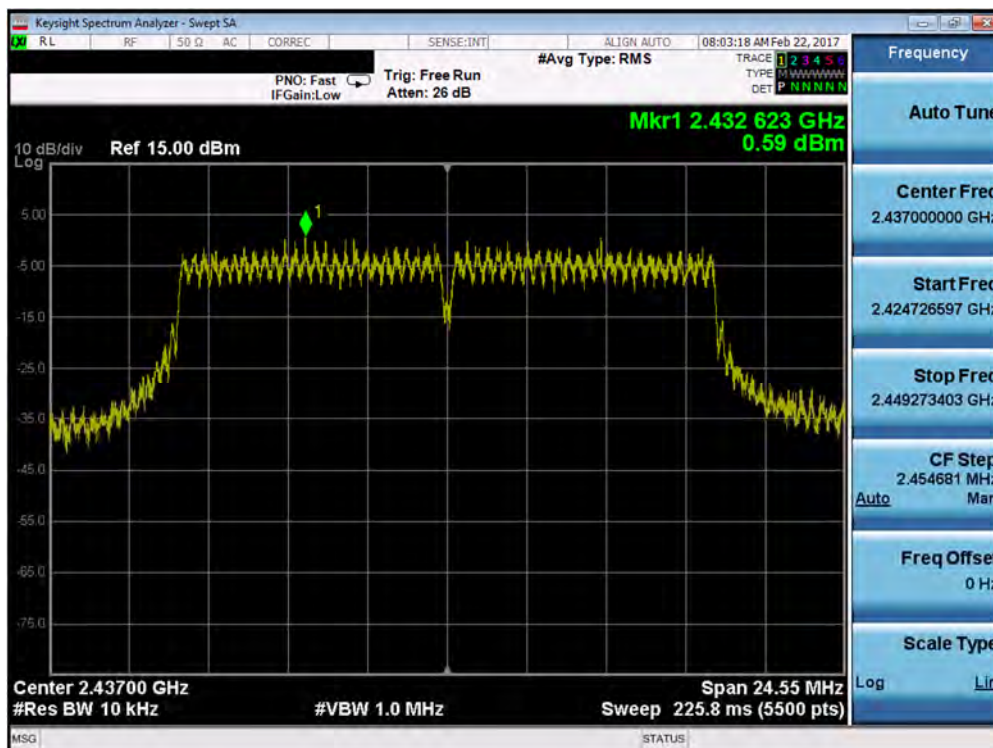
Plot 7-38. Power Spectral Density Plot (802.11g – Ch. 6)
