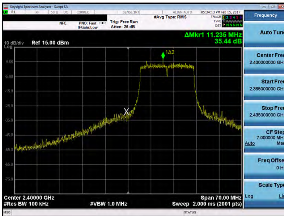
Plot 7-51. Band Edge Plot (20MHz 802.11g– Ch. 1)
