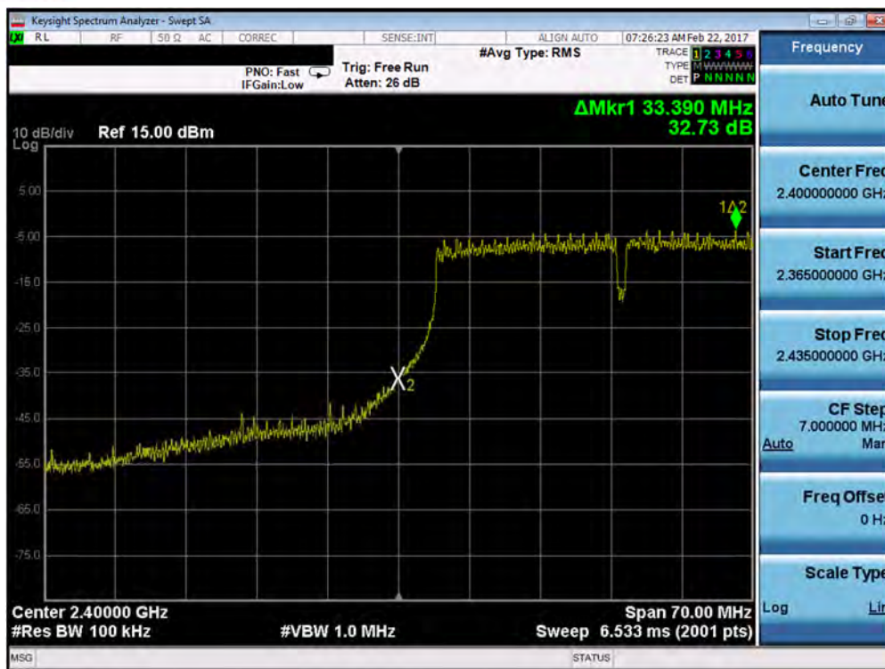
Plot 7-55. Band Edge Plot (40MHz 802.11n/ac – Ch. 3)
