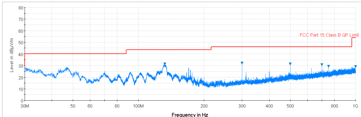
Plot 7-117. Radiated Spurious Plot below 1GHz (Pol. H)
