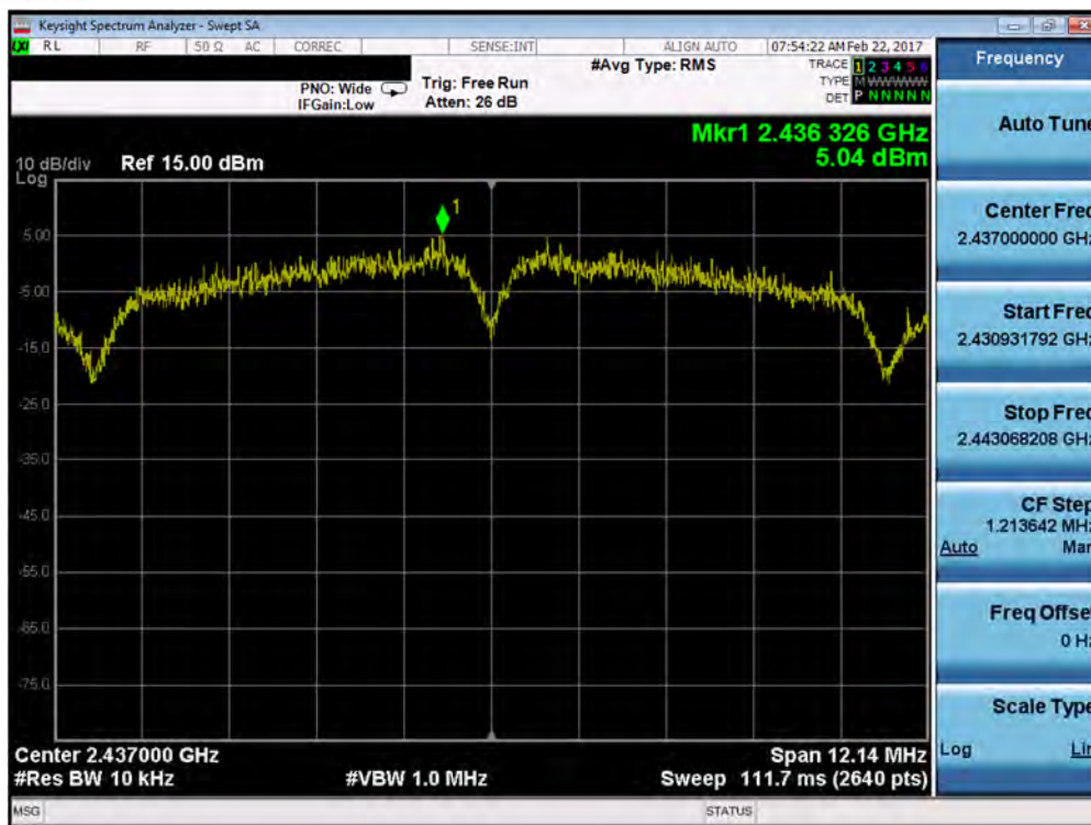
Plot 7-35. Power Spectral Density Plot (802.11b – Ch. 6)
