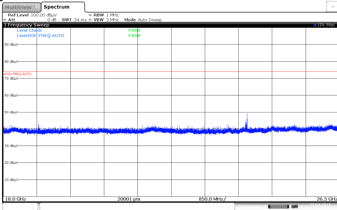
Plot 7-83. Radiated Spurious Plot above 18GHz (Pol. H)
