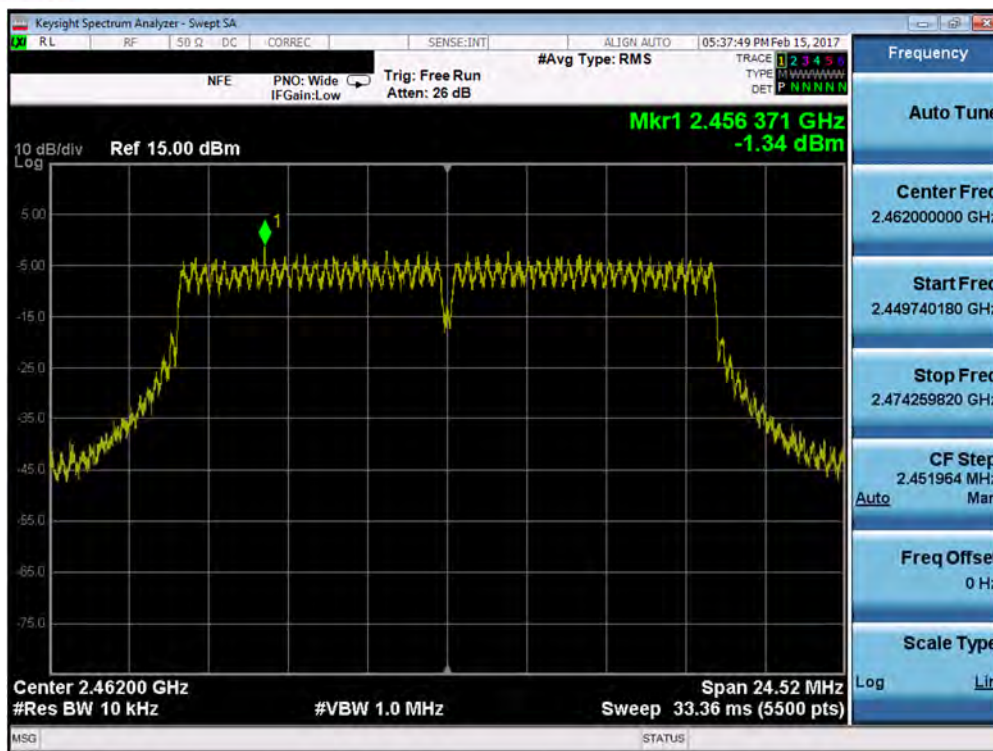
Plot 7-30. Power Spectral Density Plot (802.11g – Ch. 11)
