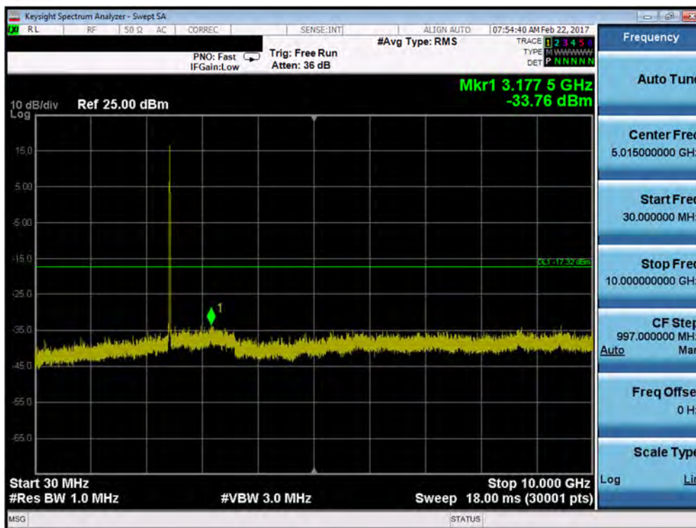
Plot 7-73. Conducted Spurious Plot (802.11b – Ch. 6)
