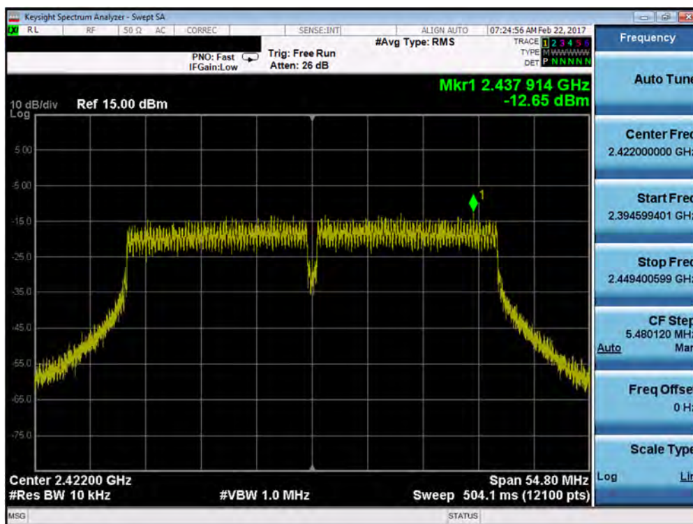
Plot 7-43. Power Spectral Density Plot (40MHz 802.11 n/ac – Ch. 3)
