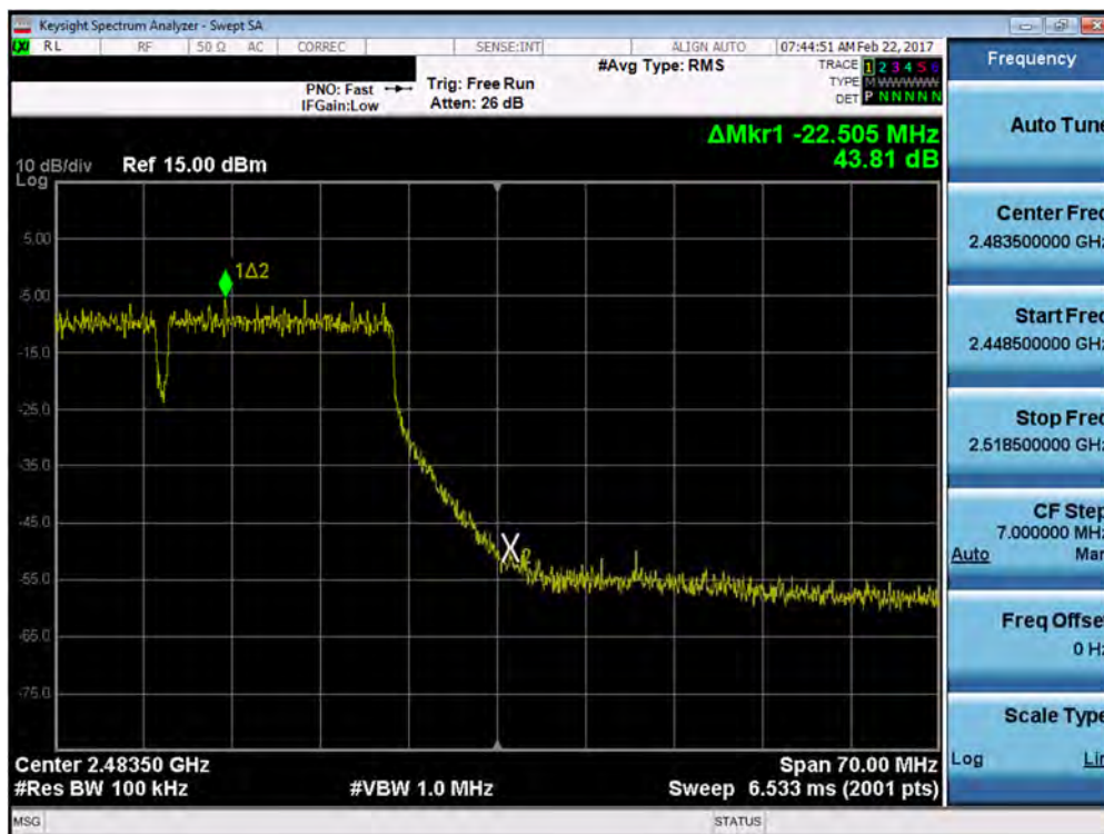
Plot 7-64. Band Edge Plot (40MHz 802.11n/ac – Ch. 10)
