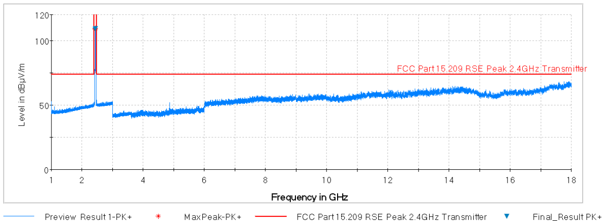
Plot 7-88. Radiated Spurious Plot above 1GHz (802.11b – Ch. 6, Ant. Pol. V)
