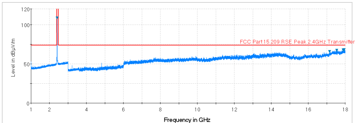
Plot 7-86. Radiated Spurious Plot above 1GHz (802.11b – Ch. 1, Ant. Pol. V)
