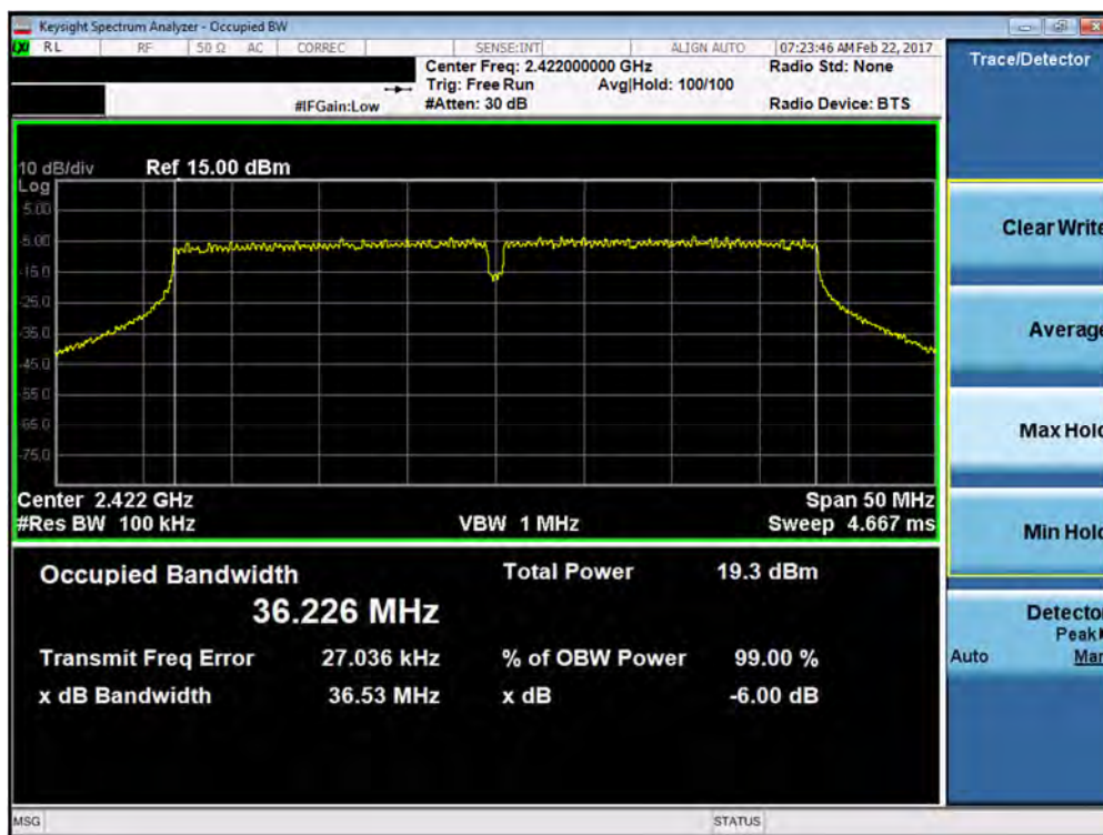
Plot 7-19. 6dB Bandwidth Plot (40MHz 802.11 n/ac – Ch. 3)
