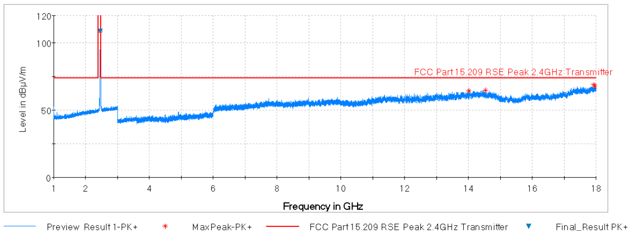
Plot 7-81. Radiated Spurious Plot above 1GHz (802.11b – Ch. 11, Ant. Pol. H)
