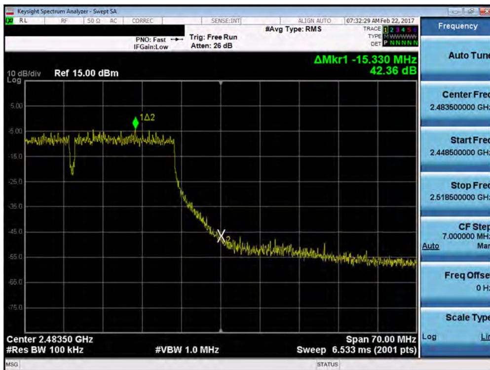
Plot 7-56. Band Edge Plot (40MHz 802.11n/ac – Ch. 10)
