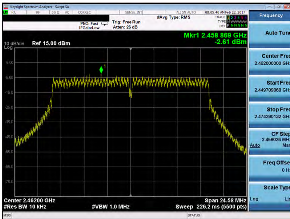
Plot 7-39. Power Spectral Density Plot (802.11g – Ch. 11)
