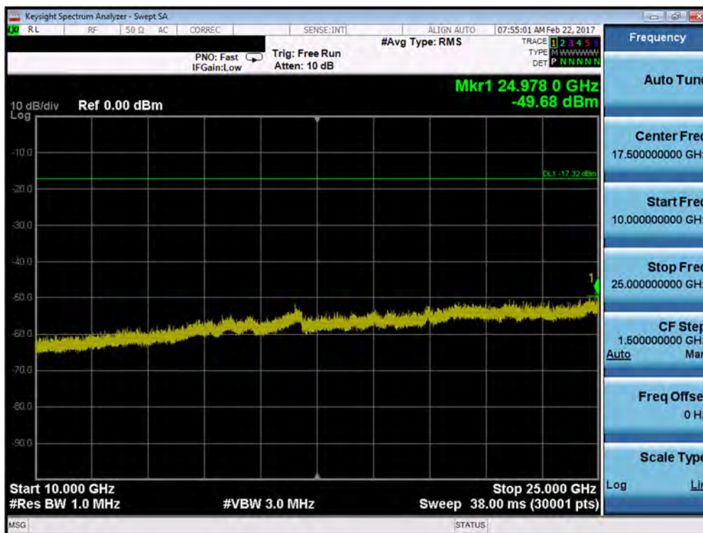
Plot 7-74. Conducted Spurious Plot (802.11b – Ch. 6)
