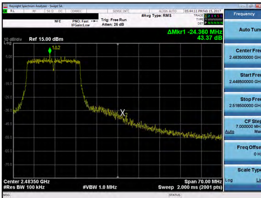
Plot 7-54. Band Edge Plot (20MHz 802.11n (2.4GHz) – Ch. 11)
