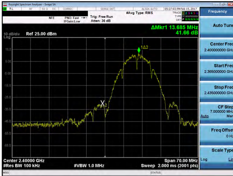
Plot 7-49. Band Edge Plot (20MHz 802.11b – Ch. 1)
