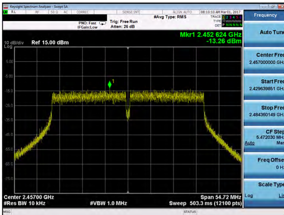
Plot 7-48. Power Spectral Density Plot (40MHz 802.11 n/ac – Ch. 10)
