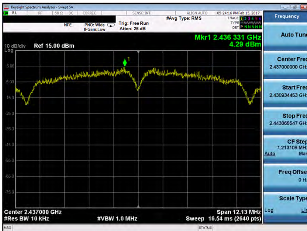
Plot 7-26. Power Spectral Density Plot (802.11b – Ch. 6)
