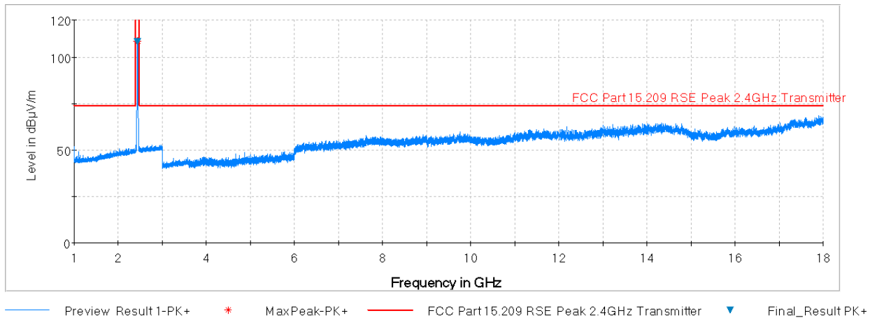
Plot 7-80. Radiated Spurious Plot above 1GHz (802.11b – Ch. 6, Ant. Pol. V)
