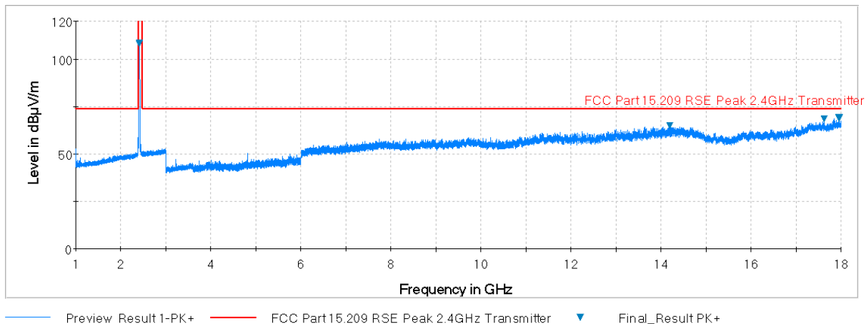
Plot 7-77. Radiated Spurious Plot above 1GHz (802.11b – Ch. 1, Ant. Pol. H)
