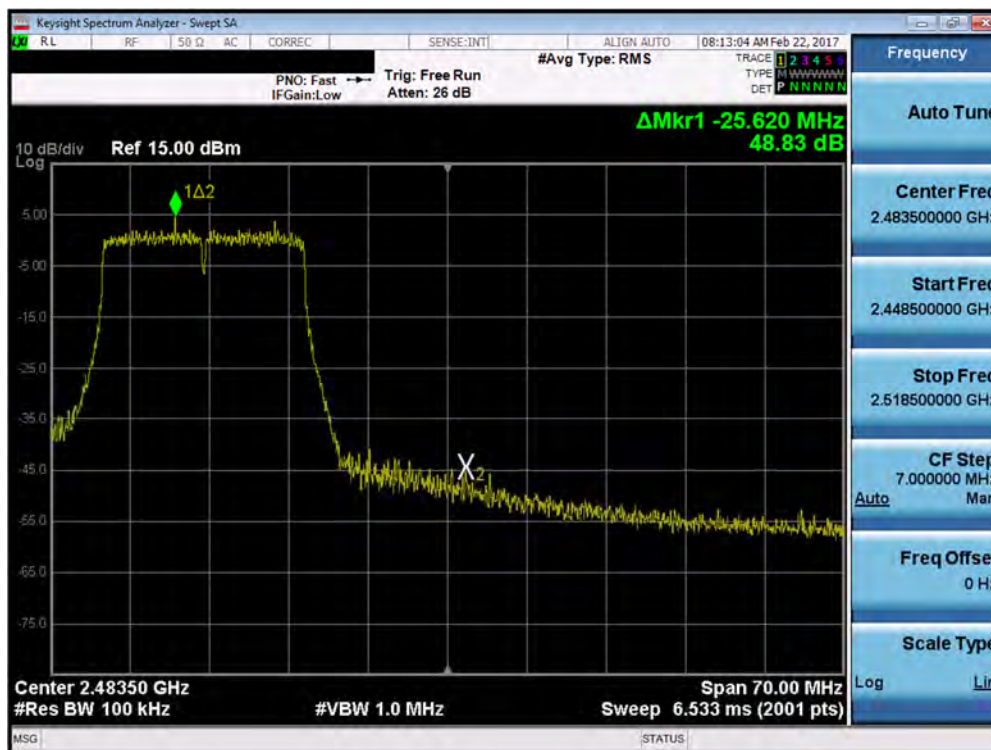
Plot 7-62. Band Edge Plot (20MHz 802.11n (2.4GHz) – Ch. 11)
