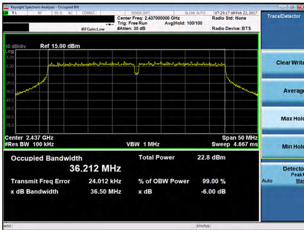
Plot 7-20. 6dB Bandwidth Plot (40MHz 802.11 n/ac – Ch. 6)
