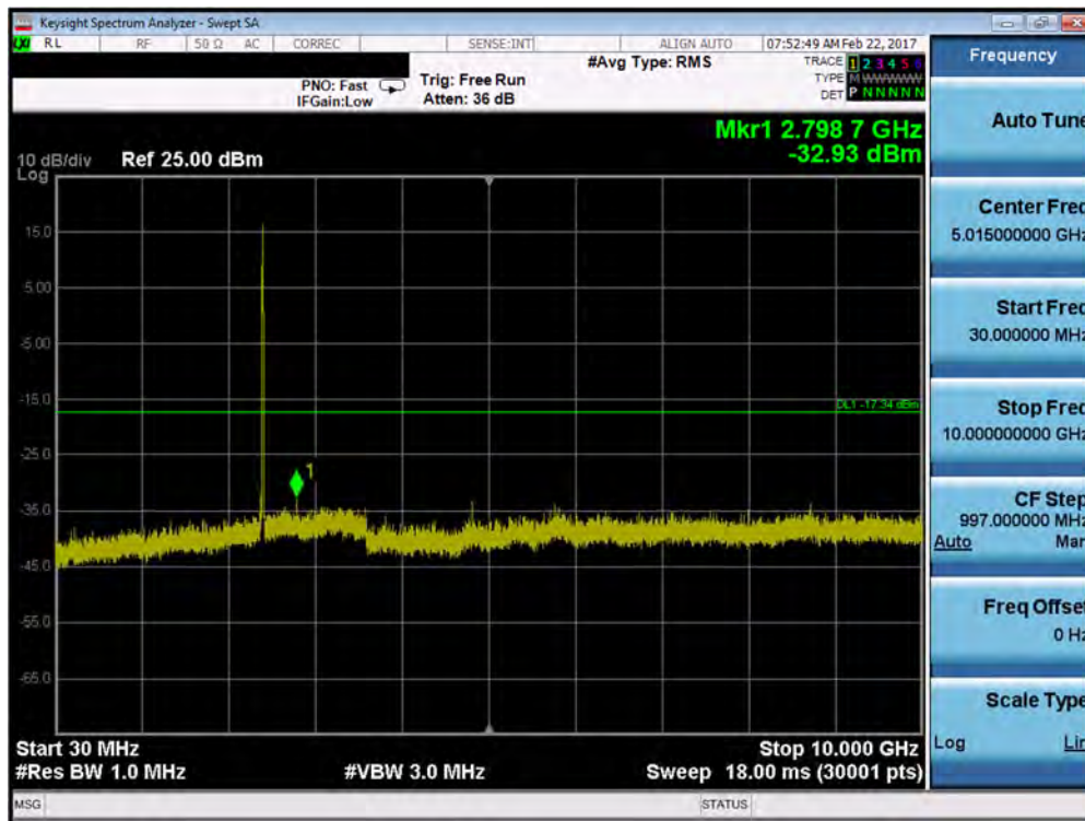
Plot 7-71. Conducted Spurious Plot (802.11b – Ch. 1)
