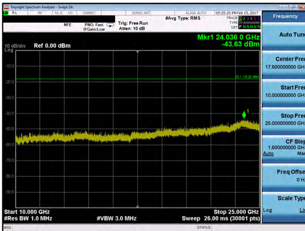
Plot 7-68. Conducted Spurious Plot (802.11b – Ch. 6)
