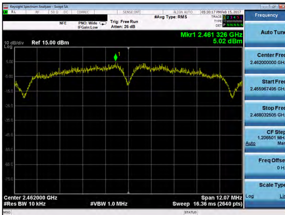
Plot 7-27. Power Spectral Density Plot (802.11b – Ch. 11)
