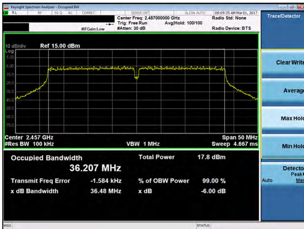
Plot 7-24. 6dB Bandwidth Plot (40MHz 802.11 n/ac – Ch. 10)
