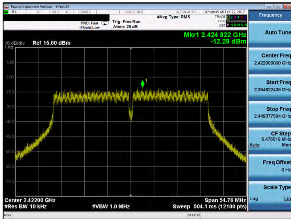
Plot 7-46. Power Spectral Density Plot (40MHz 802.11 n/ac – Ch. 3)
