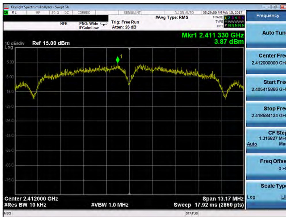
Plot 7-25. Power Spectral Density Plot (802.11b – Ch. 1)
