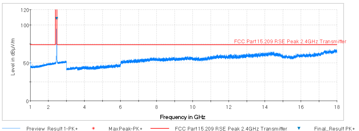
Plot 7-82. Radiated Spurious Plot above 1GHz (802.11b – Ch. 11, Ant. Pol. V)
