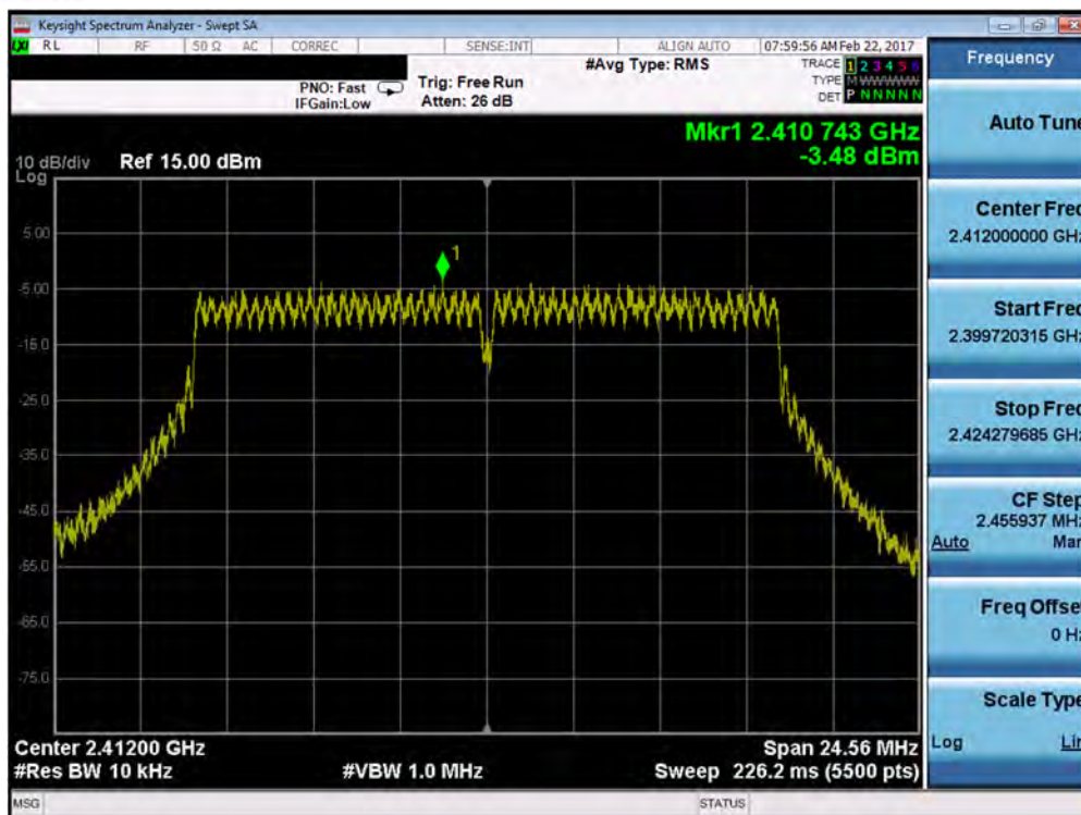
Plot 7-37. Power Spectral Density Plot (802.11g – Ch. 1)
