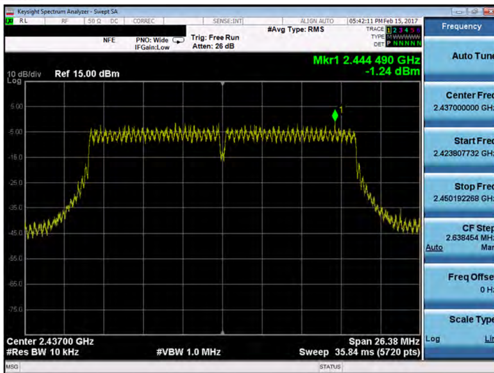
Plot 7-32. Power Spectral Density Plot (802.11n (2.4GHz) – Ch. 6)
