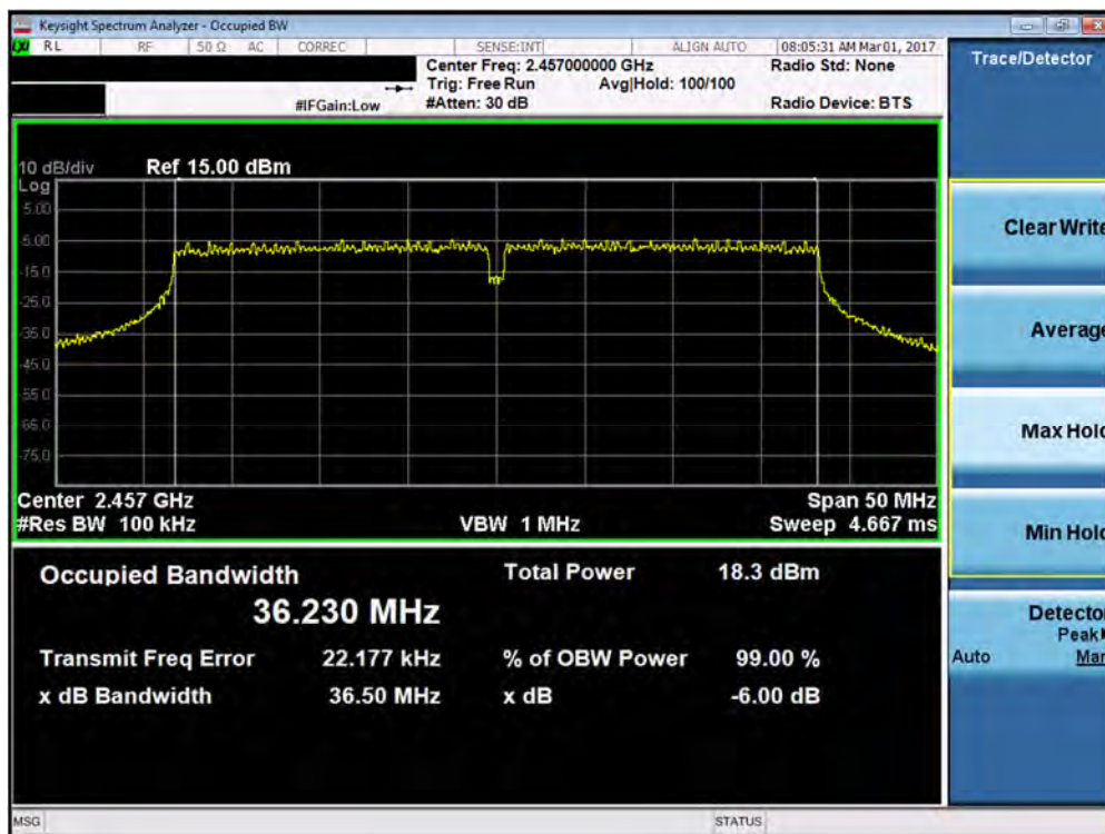
Plot 7-21. 6dB Bandwidth Plot (40MHz 802.11 n/ac – Ch. 10)
