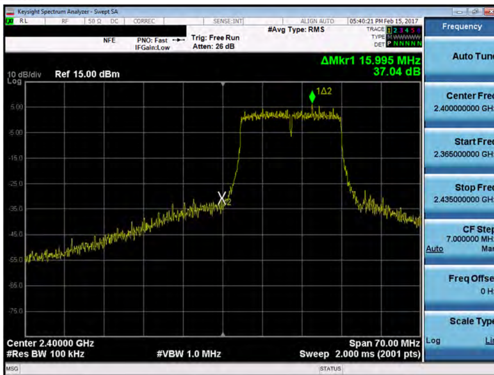
Plot 7-53. Band Edge Plot (20MHz 802.11n (2.4GHz) – Ch. 1)
