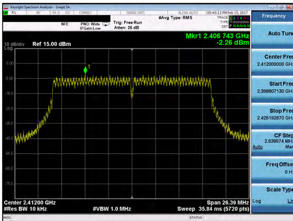
Plot 7-31. Power Spectral Density Plot (802.11n (2.4GHz) – Ch. 1)
