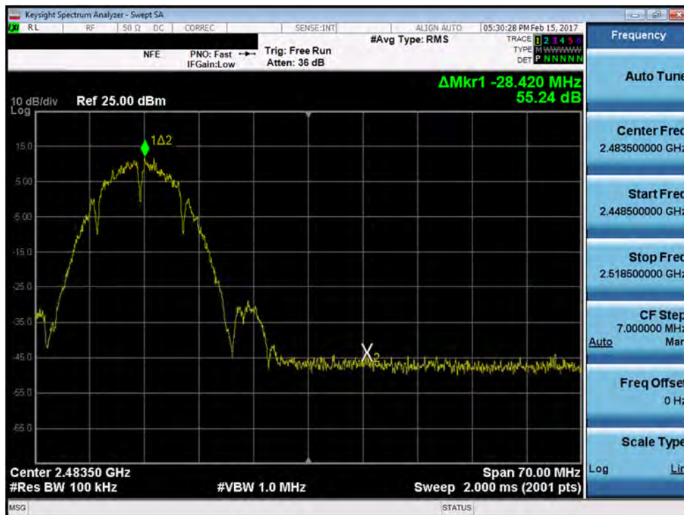
Plot 7-50. Band Edge Plot (20MHz 802.11b – Ch. 11)
