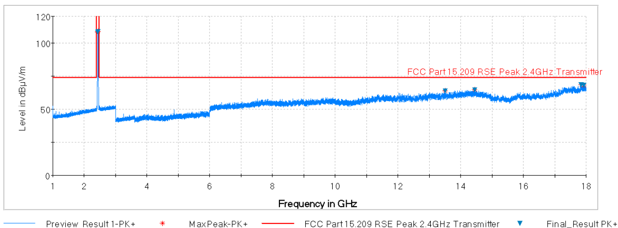
Plot 7-79. Radiated Spurious Plot above 1GHz (802.11b – Ch. 6, Ant. Pol. H)
