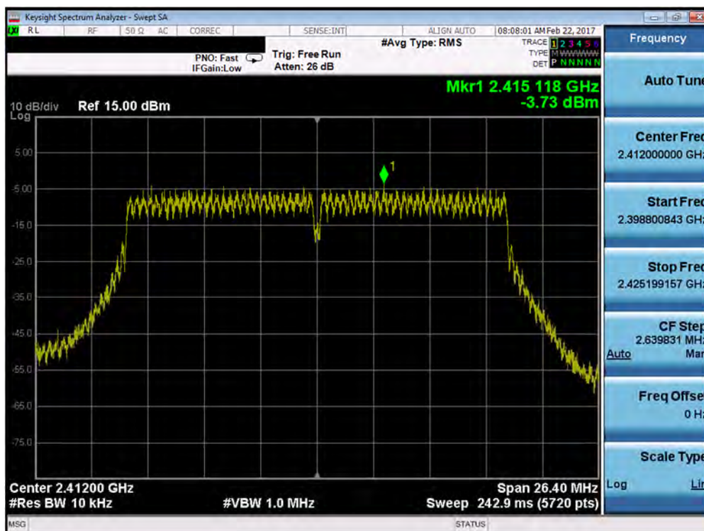
Plot 7-40. Power Spectral Density Plot (802.11n (2.4GHz) – Ch. 1)
