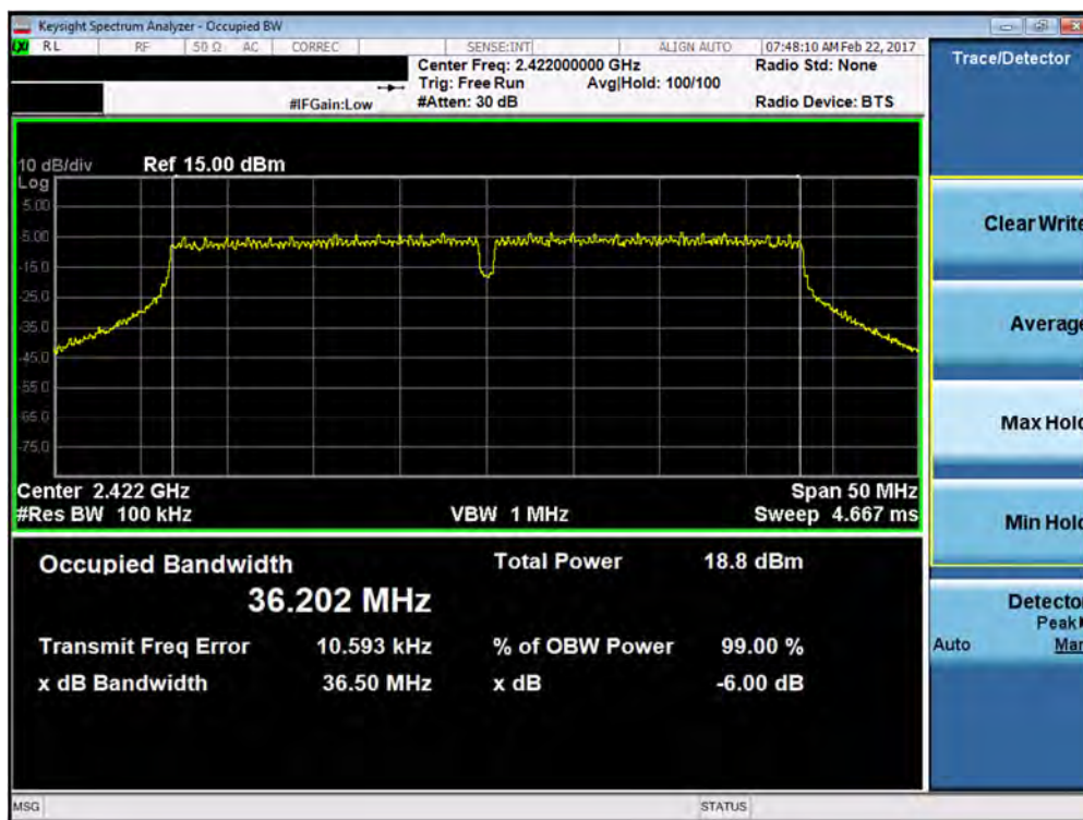
Plot 7-22. 6dB Bandwidth Plot (40MHz 802.11 n/ac – Ch. 3)
