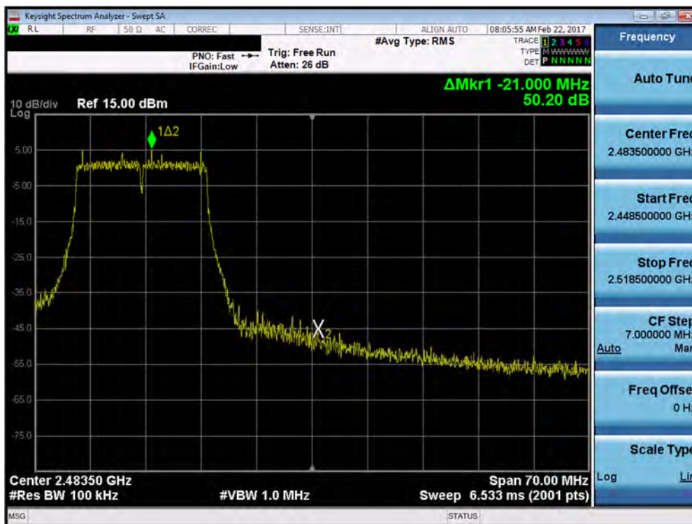
Plot 7-60. Band Edge Plot (20MHz 802.11g – Ch. 11)
