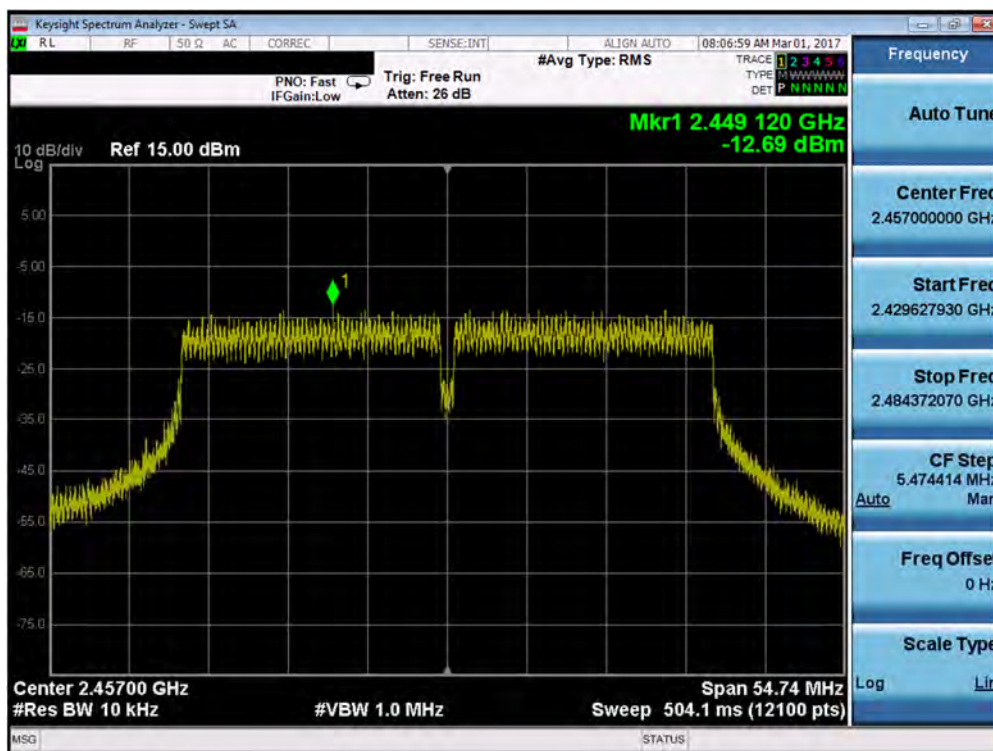
Plot 7-45. Power Spectral Density Plot (40MHz 802.11 n/ac (2.4GHz) – Ch. 10)
