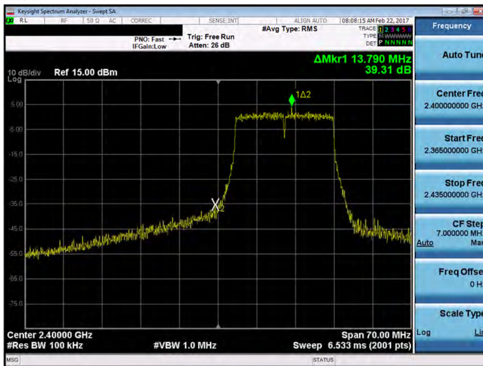
Plot 7-61. Band Edge Plot (20MHz 802.11n (2.4GHz) – Ch. 1)
