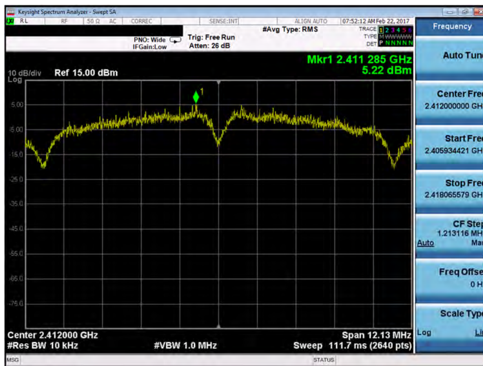
Plot 7-34. Power Spectral Density Plot (802.11b – Ch. 1)
