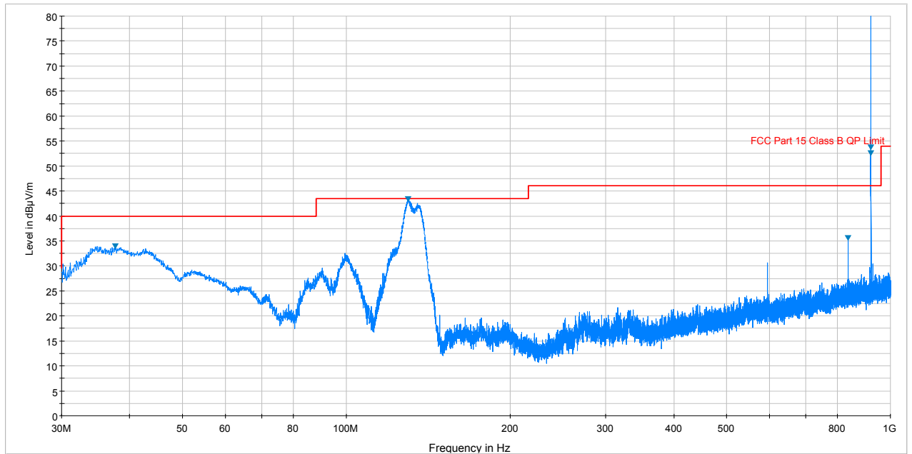
Plot 7-6. Radiated Spurious Plot below 1GHz (Zwave – 921.7MHz, Ant. Pol. V)
