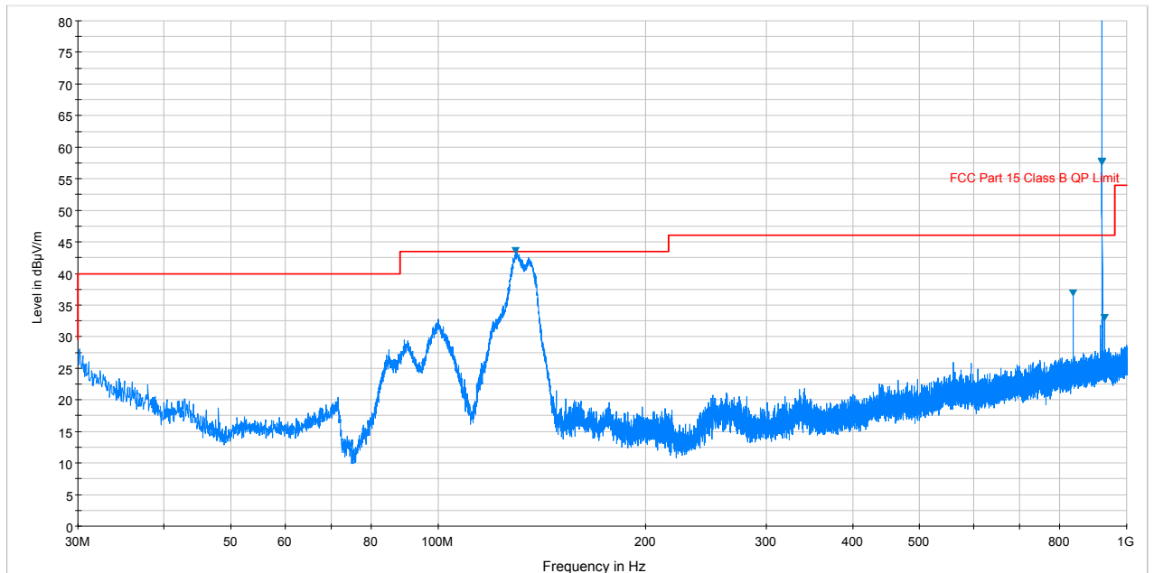
Plot 7-5. Radiated Spurious Plot below 1GHz (Zwave – 921.7MHz, Ant. Pol. H)
