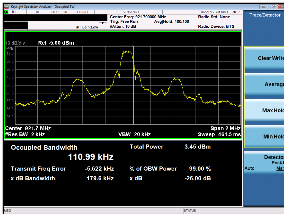
Plot 7-1. Occupied Bandwidth Plot (ZWave – Ch. 921.7MHz – 100kbps)
