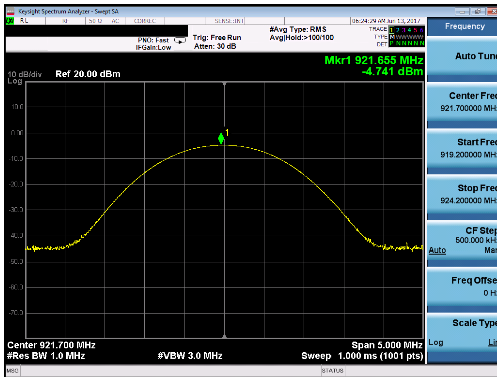
Plot 7-2. Peak Conducted Power (ZWave – 921.7MHz)
