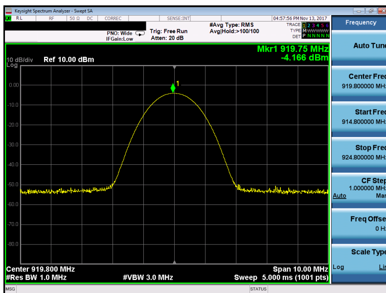
Plot 7-3. Peak Conducted Power (ZWave – 919.8MHz)
