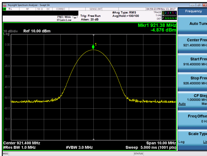
Plot 7-4. Peak Conducted Power (ZWave – 921.4MHz)
