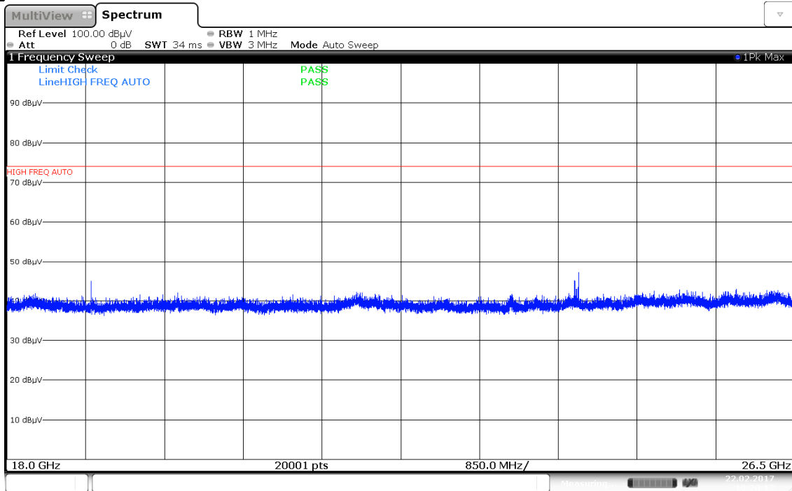
Plot 7-27. Radiated Spurious Plot above 18GHz (Pol. H)
