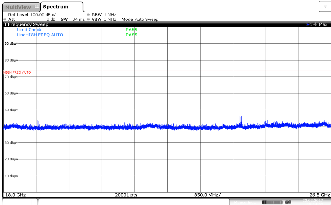
Plot 7-28. Radiated Spurious Plot above 18GHz (Pol. V)
