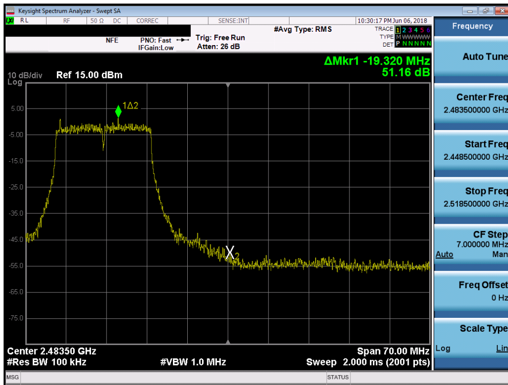
Plot 7-74. Band Edge Plot SISO ANT2 (20MHz 802.11g - Ch. 11)
