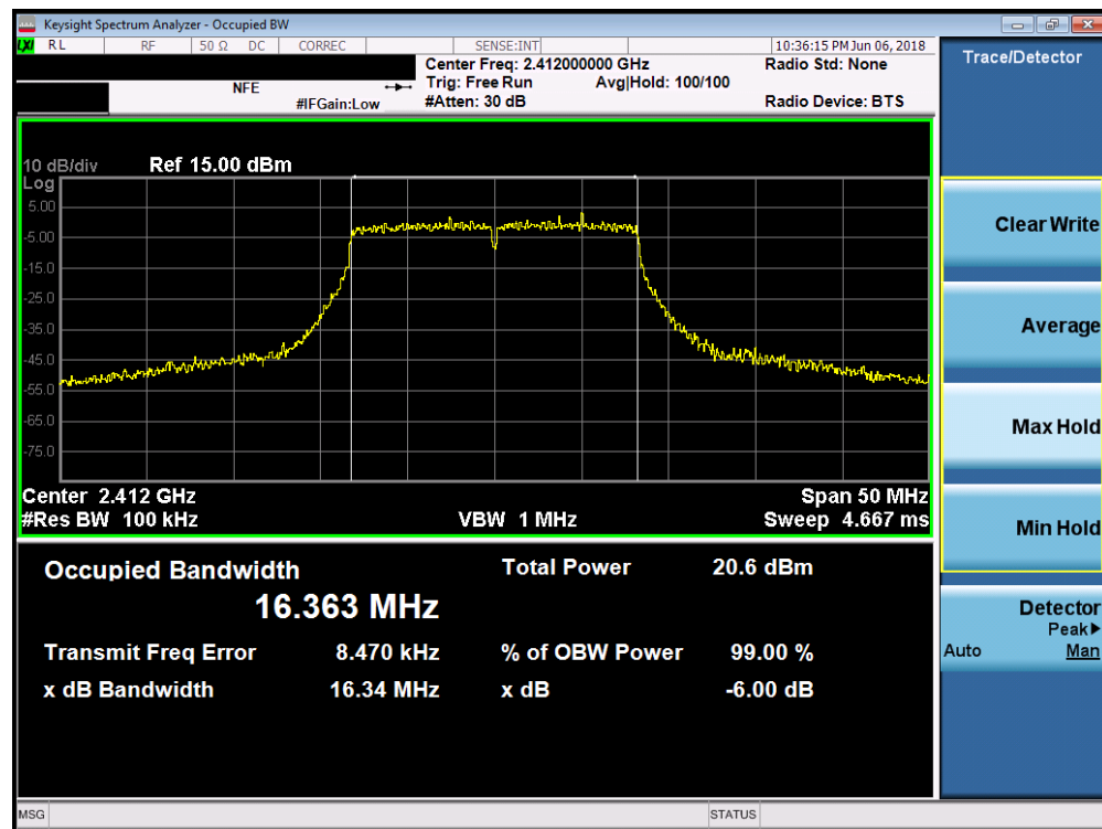
Plot 7-19. 6dB Bandwidth Plot SISO ANT2 (20MHz 802.11g – Ch. 1)
