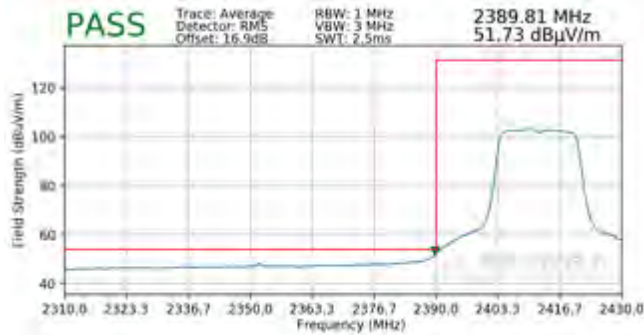
Plot 7-117. Radiated Restricted Lower Band Edge Measurement MIMO (Average)
