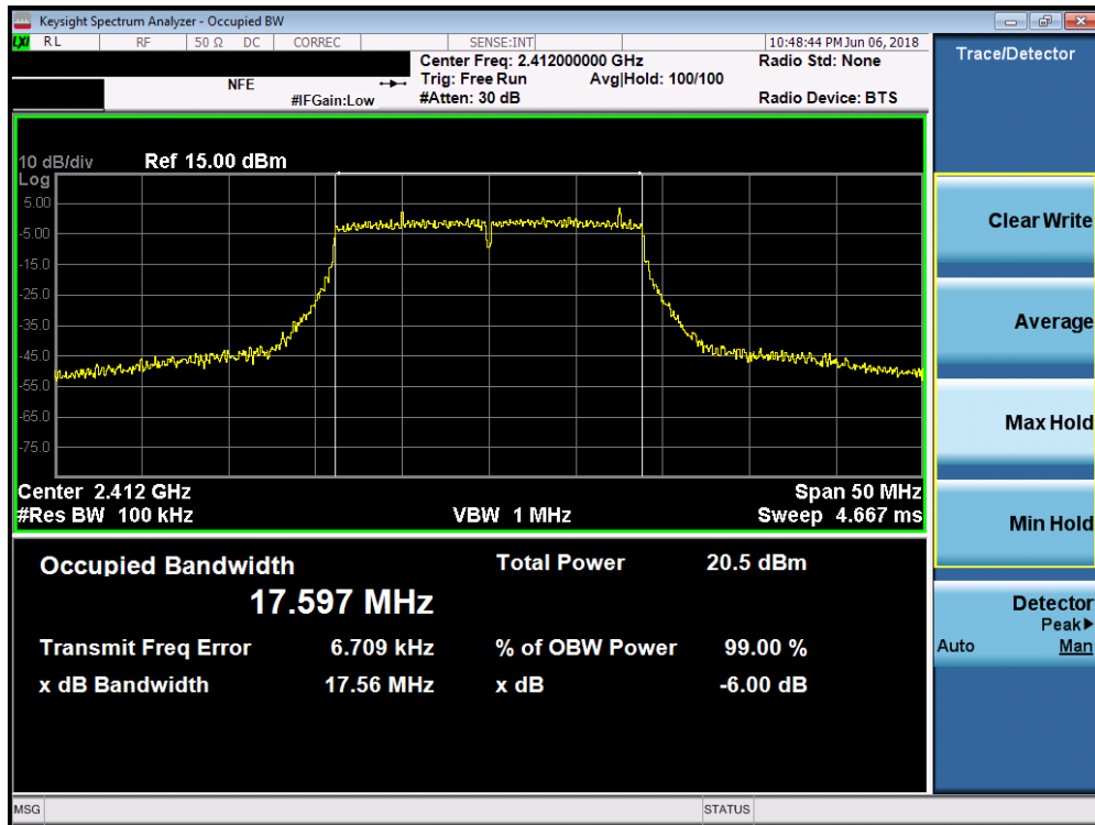
Plot 7-22. 6dB Bandwidth Plot SISO ANT2 (20MHz 802.11n (2.4GHz) – Ch. 1)
