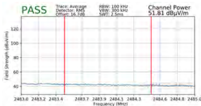
Plot 7-123. Radiated Restricted Upper Band Edge Measurement MIMO (Average)
