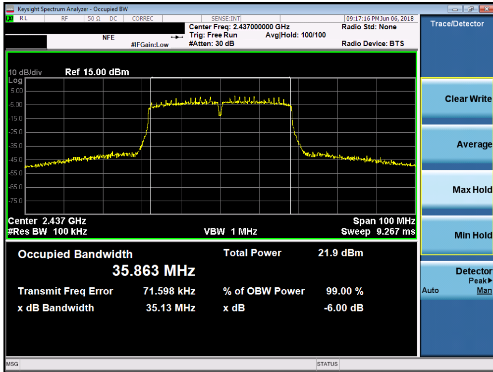
Plot 7-11. 6dB Bandwidth Plot SISO ANT1 (40MHz 802.11n (2.4GHz) – Ch. 6)
