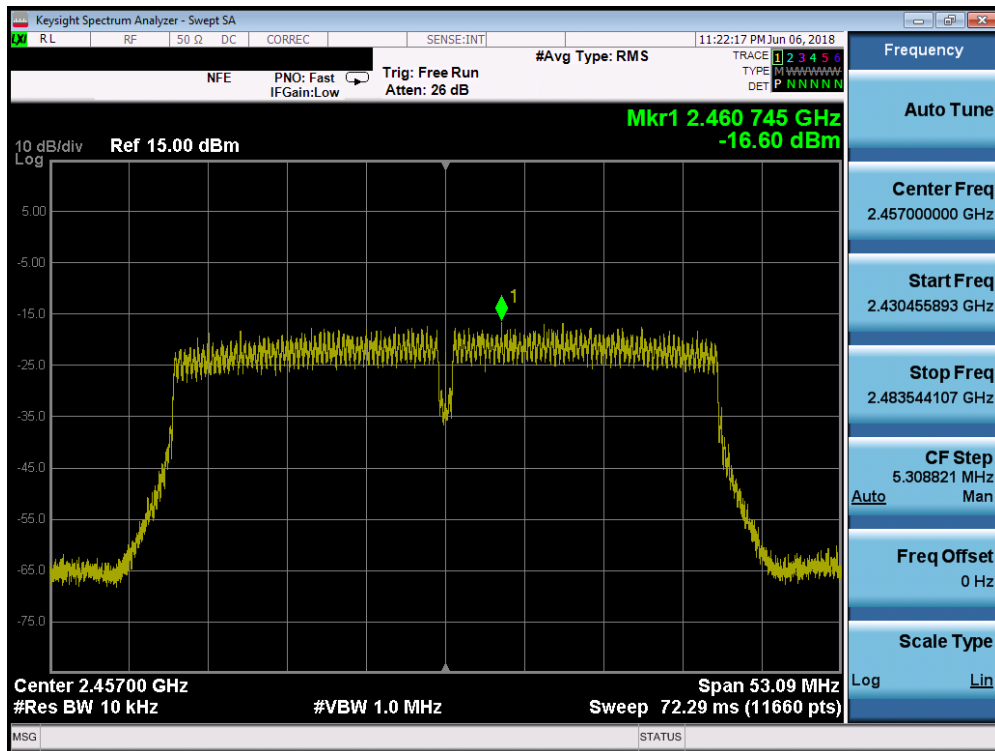
Plot 7-60. Power Spectral Density Plot SISO ANT2 (40MHz 802.11ac (2.4GHz) – Ch. 10)
