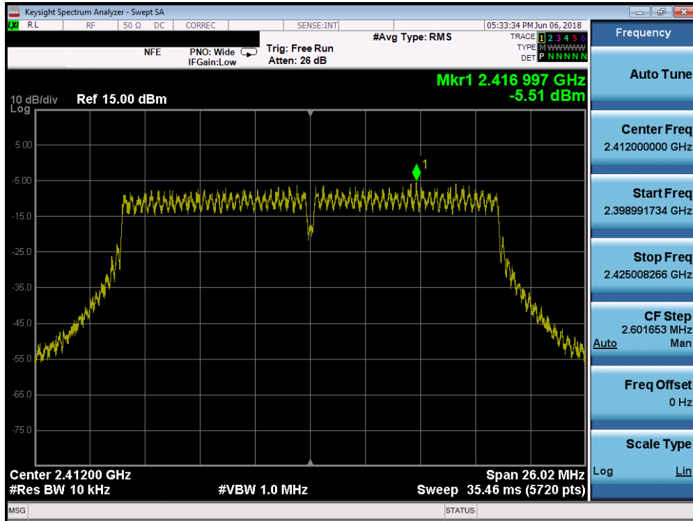
Plot 7-37. Power Spectral Density Plot SISO ANT1 (20MHz 802.11n (2.4GHz) – Ch. 1)
