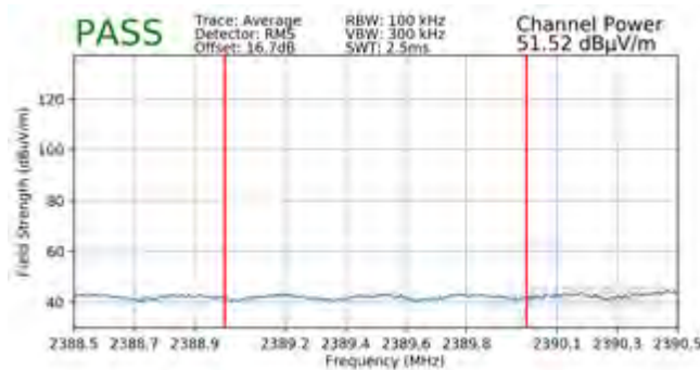
Plot 7-113. Radiated Restricted Lower Band Edge Measurement SISO ANT2 (Average)
