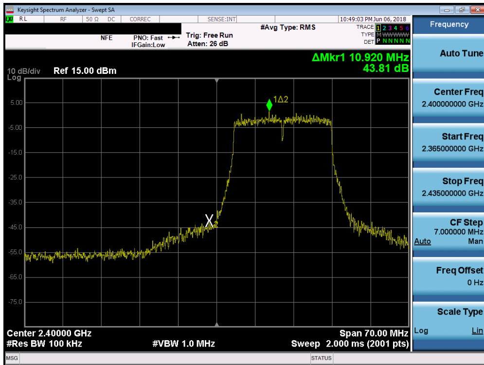
Plot 7-75. Band Edge Plot SISO ANT2 (20MHz 802.11n (2.4GHz) – Ch. 1)
