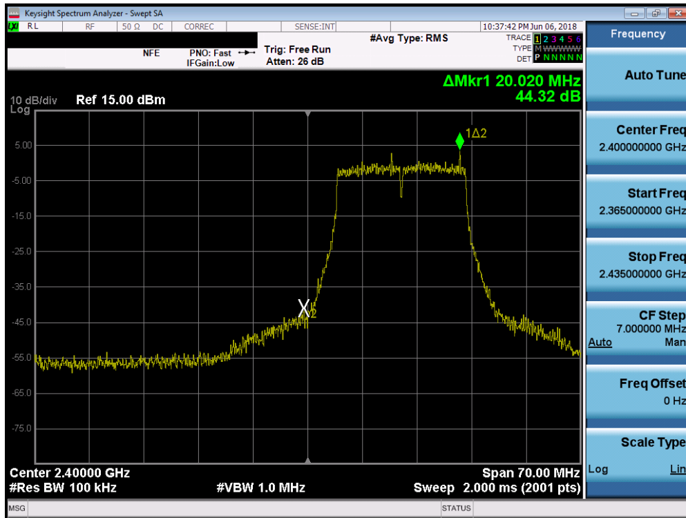
Plot 7-73. Band Edge Plot SISO ANT2 (20MHz 802.11g- Ch. 1)
