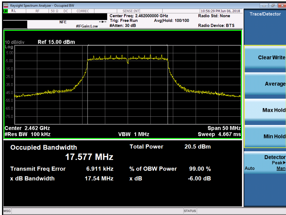
Plot 7-24. 6dB Bandwidth Plot SISO ANT2 (20MHz 802.11n (2.4GHz) – Ch. 11)
