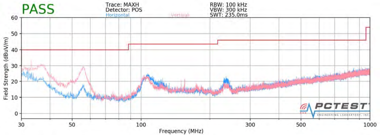
Plot 7-130. Radiated Spurious Plot below 1GHz SISO ANT2
