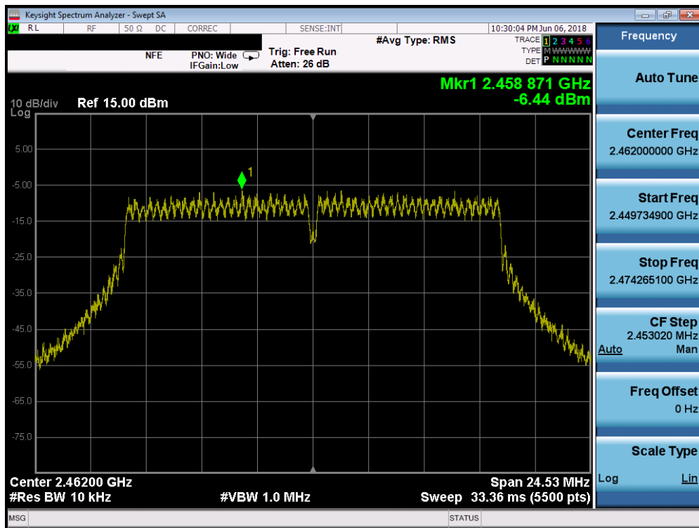
Plot 7-51. Power Spectral Density Plot SISO ANT2 (20MHz 802.11g – Ch. 11)
