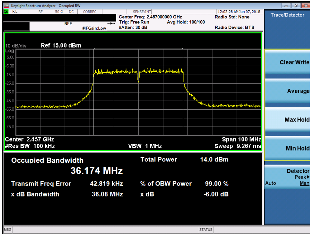
Plot 7-30. 6dB Bandwidth Plot SISO ANT2 (40MHz 802.11ac (2.4GHz) – Ch. 10)
