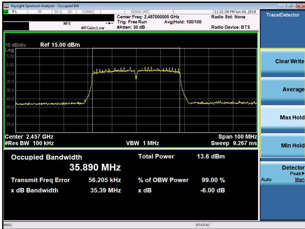
Plot 7-27. 6dB Bandwidth Plot SISO ANT2 (40MHz 802.11n (2.4GHz) – Ch. 10)
