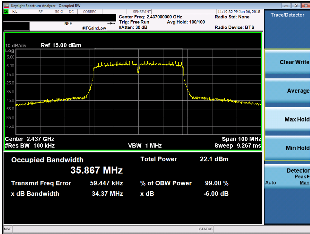
Plot 7-26. 6dB Bandwidth Plot SISO ANT2 (40MHz 802.11n (2.4GHz) – Ch. 6)
