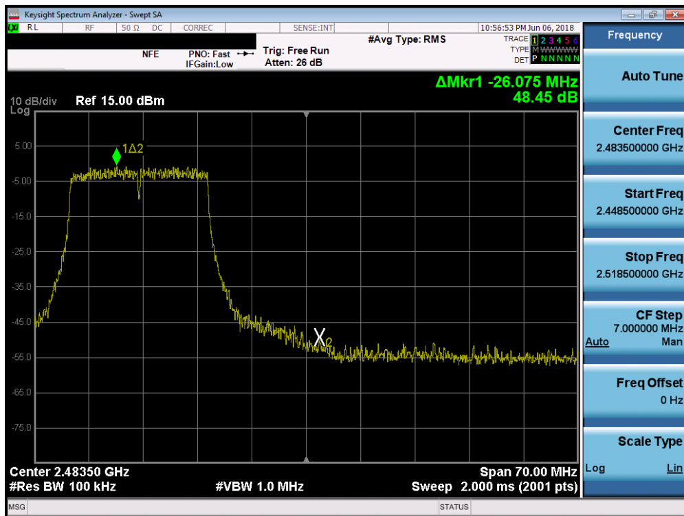
Plot 7-76. Band Edge Plot SISO ANT2 (20MHz 802.11n (2.4GHz) – Ch. 11)
