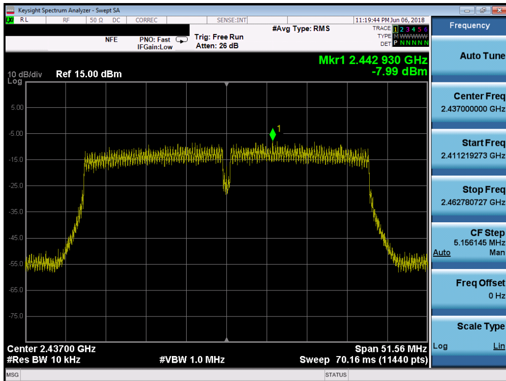
Plot 7-56. Power Spectral Density Plot SISO ANT2 (40MHz 802.11n (2.4GHz) – Ch. 6)
