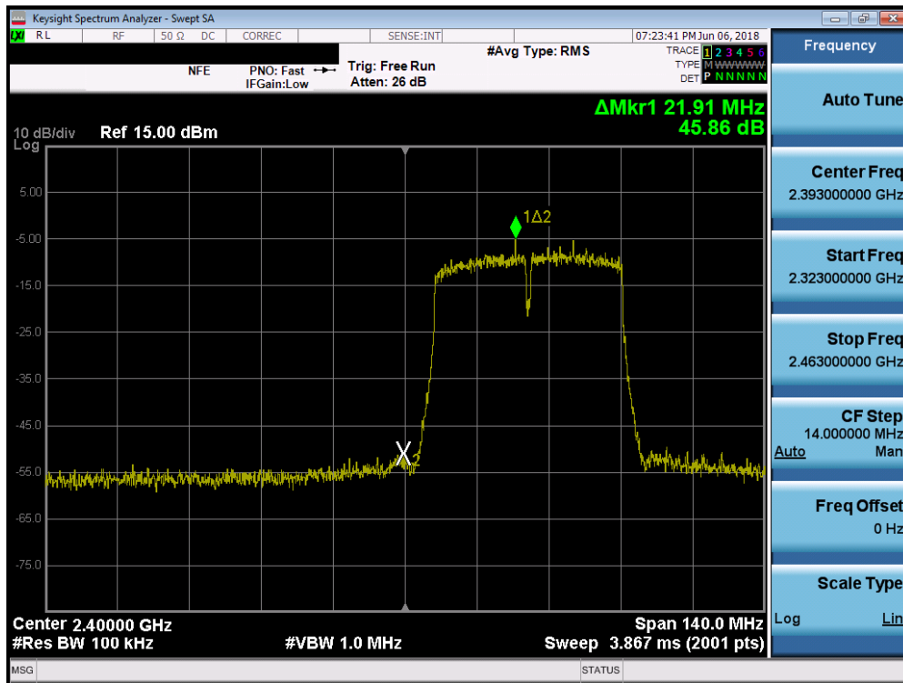
Plot 7-67. Band Edge Plot SISO ANT1 (40MHz 802.11n (2.4GHz) – Ch. 3)
