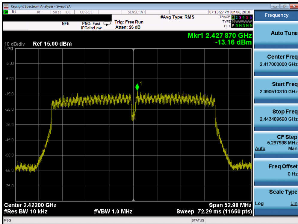
Plot 7-40. Power Spectral Density Plot SISO ANT1 (40MHz 802.11n (2.4GHz) – Ch. 3)
