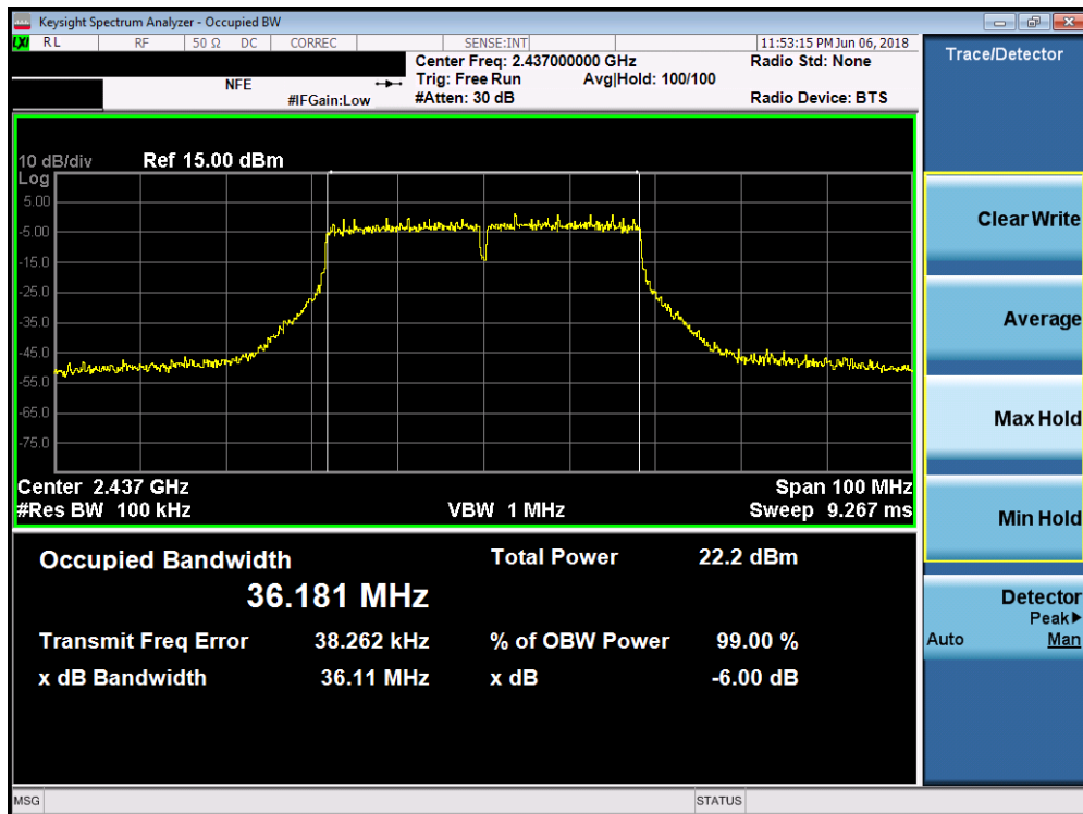
Plot 7-29. 6dB Bandwidth Plot SISO ANT2 (40MHz 802.11ac (2.4GHz) – Ch. 6)
