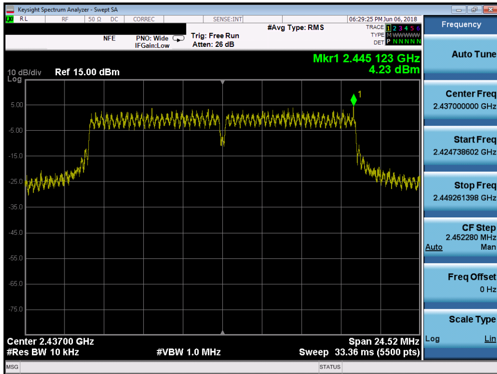
Plot 7-35. Power Spectral Density Plot SISO ANT1 (20MHz 802.11g – Ch. 6)
