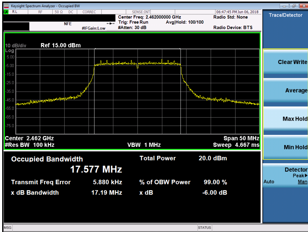
Plot 7-9. 6dB Bandwidth Plot SISO ANT1 (20MHz 802.11n (2.4GHz) – Ch. 11)
