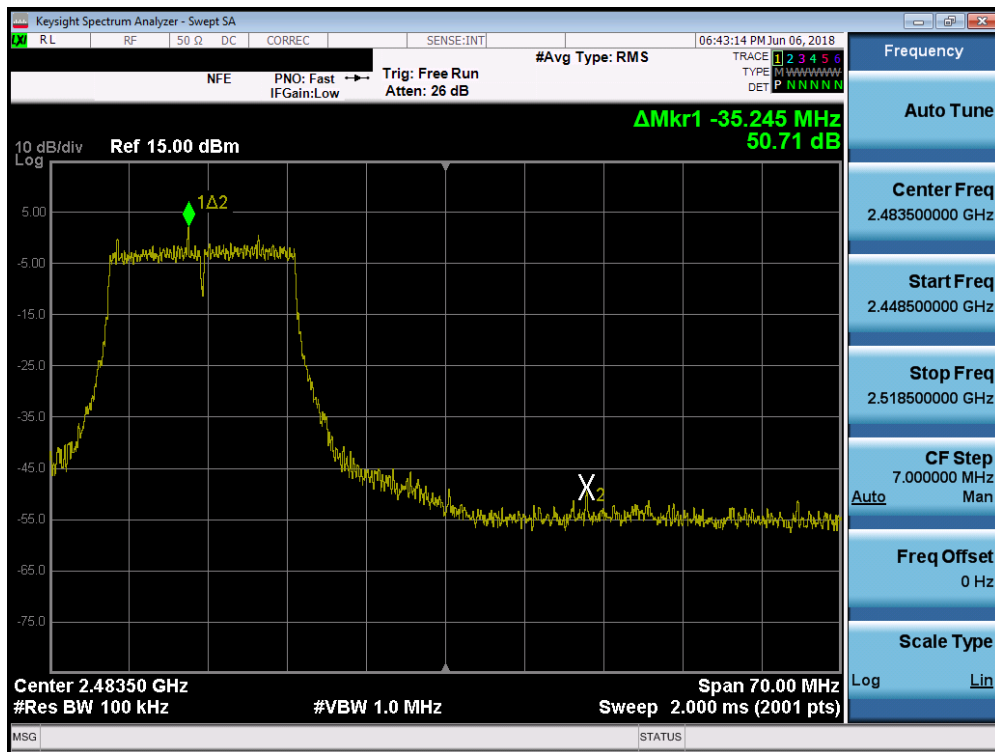
Plot 7-64. Band Edge Plot SISO ANT1 (20MHz 802.11g – Ch. 11)
