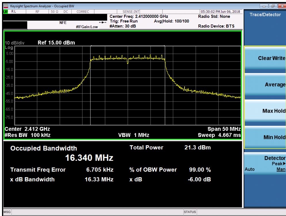
Plot 7-4. 6dB Bandwidth Plot SISO ANT1 (20MHz 802.11g – Ch. 1)
