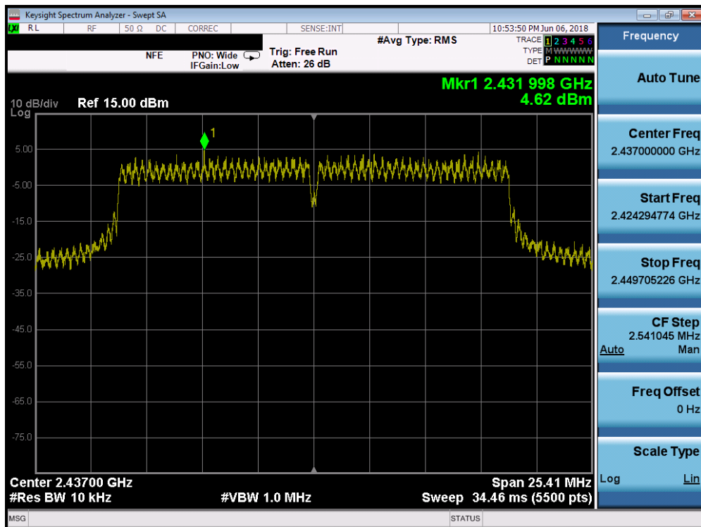
Plot 7-53. Power Spectral Density Plot SISO ANT2 (20MHz 802.11n (2.4GHz) – Ch. 6)
