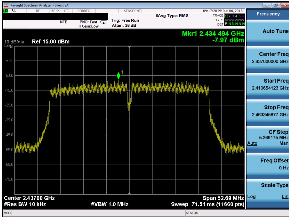
Plot 7-41. Power Spectral Density Plot SISO ANT1 (40MHz 802.11n (2.4GHz) – Ch. 6)
