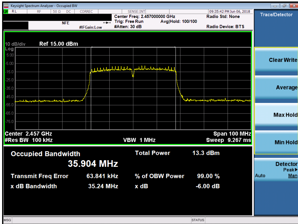
Plot 7-12. 6dB Bandwidth Plot SISO ANT1 (40MHz 802.11n (2.4GHz) – Ch. 10)
