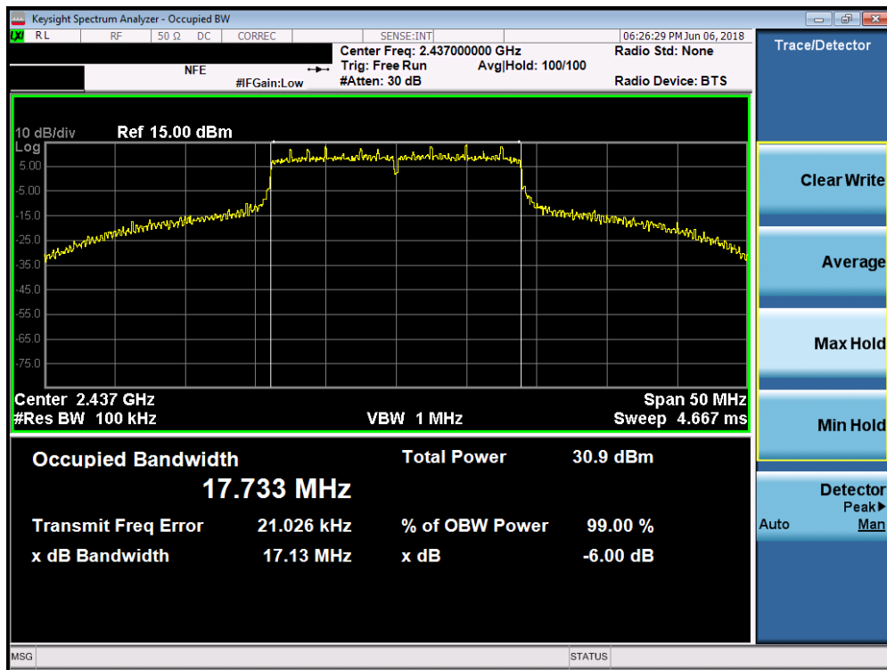
Plot 7-8. 6dB Bandwidth Plot SISO ANT1 (20MHz 802.11n (2.4GHz) – Ch. 6)
