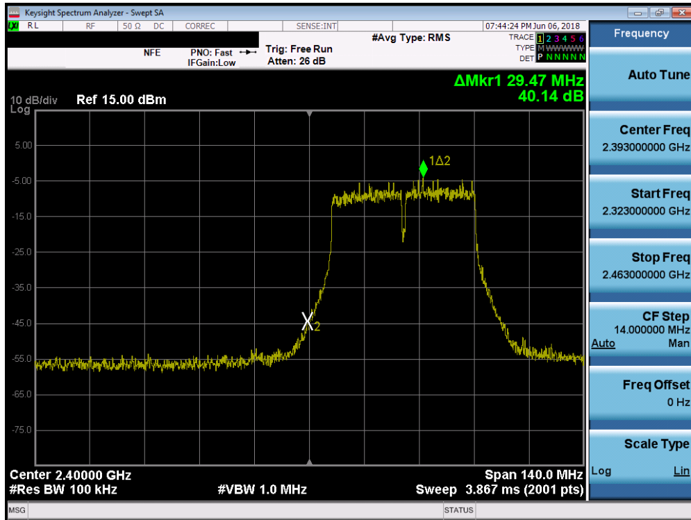
Plot 7-69. Band Edge Plot SISO ANT1 (40MHz 802.11ac (2.4GHz) – Ch. 3)
