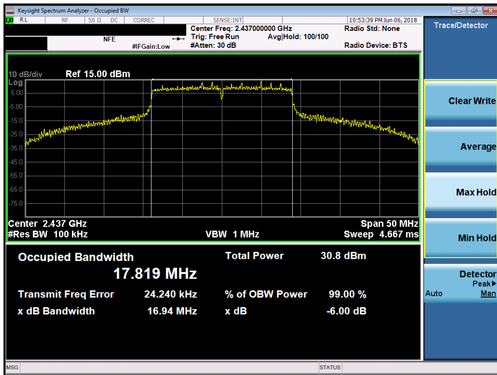
Plot 7-23. 6dB Bandwidth Plot SISO ANT2 (20MHz 802.11n (2.4GHz) – Ch. 6)
