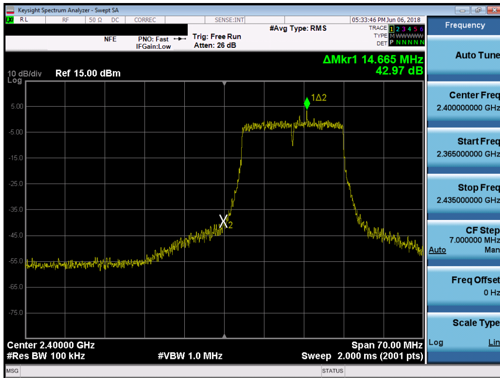
Plot 7-65. Band Edge Plot SISO ANT1 (20MHz 802.11n (2.4GHz) – Ch. 1)
