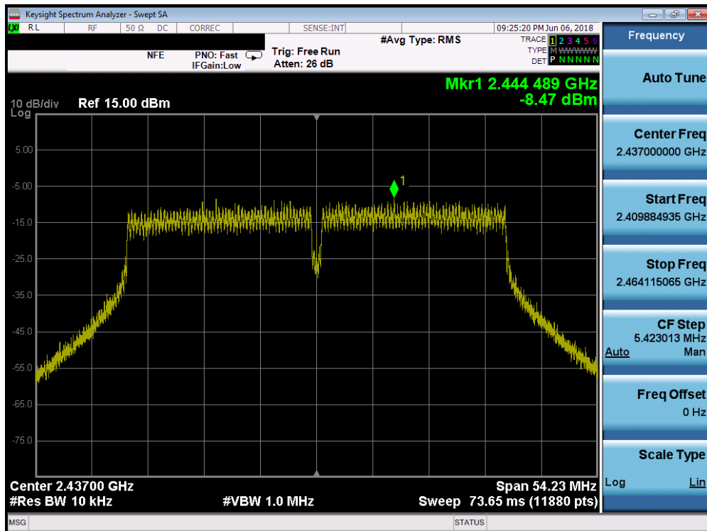
Plot 7-44. Power Spectral Density Plot SISO ANT1 (40MHz 802.11ac (2.4GHz) – Ch. 6)
