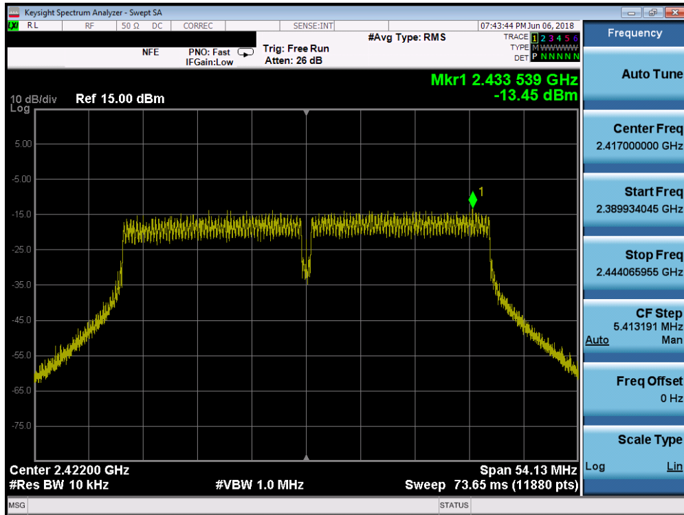
Plot 7-43. Power Spectral Density Plot SISO ANT1 (40MHz 802.11ac (2.4GHz) – Ch. 3)
