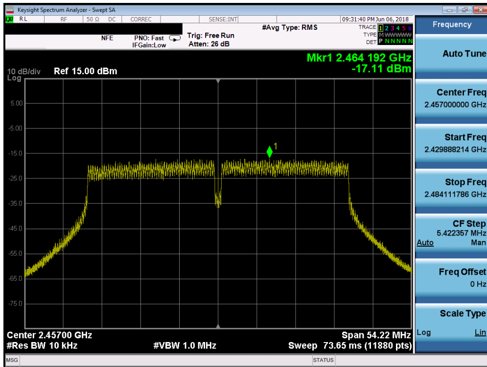
Plot 7-45. Power Spectral Density Plot SISO ANT1 (40MHz 802.11ac (2.4GHz) – Ch. 10)
