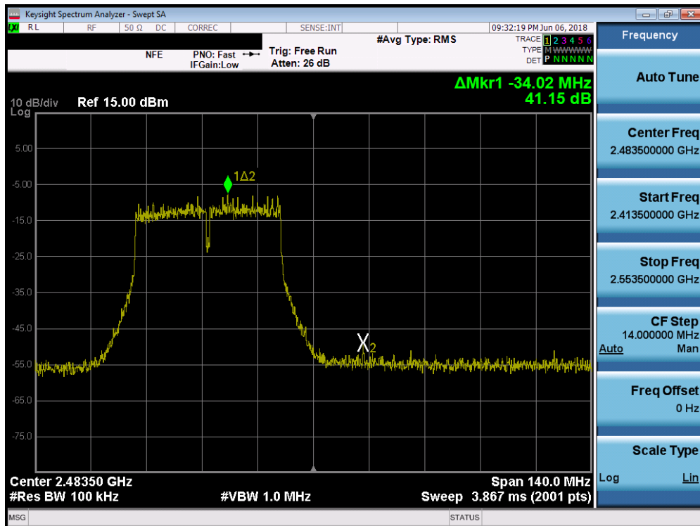
Plot 7-70. Band Edge Plot SISO ANT1 (40MHz 802.11ac (2.4GHz) – Ch. 10)
