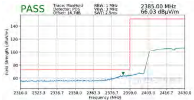
Plot 7-114. Radiated Restricted Lower Band Edge Measurement SISO ANT2 (Peak)
