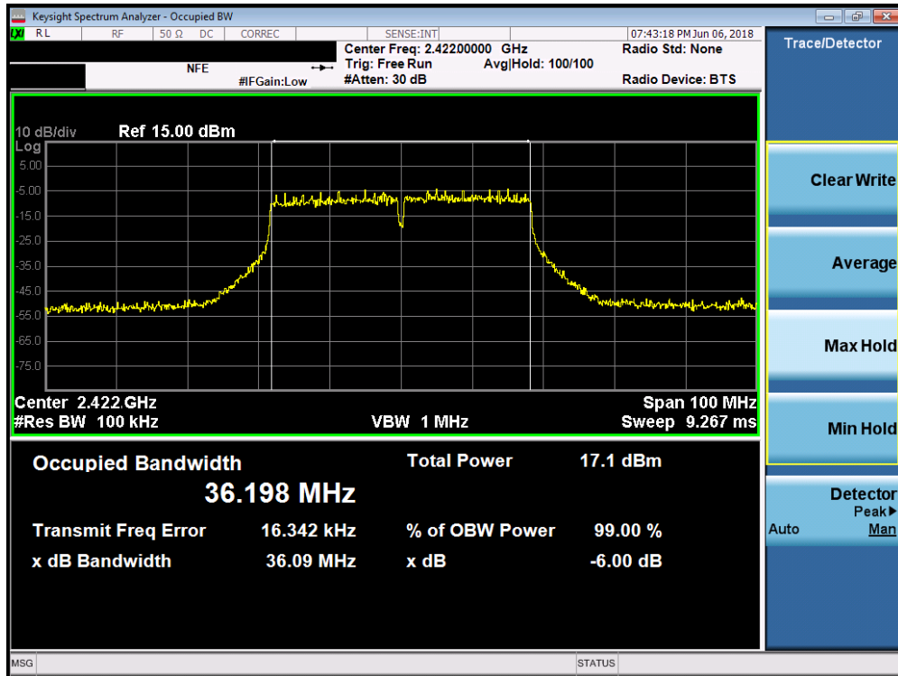
Plot 7-13. 6dB Bandwidth Plot SISO ANT1 (40MHz 802.11ac (2.4GHz) – Ch. 3)
