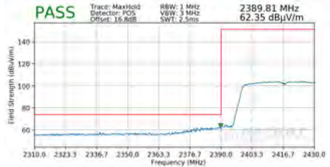
Plot 7-106. Radiated Restricted Lower Band Edge Measurement SISO ANT1 (Peak)
