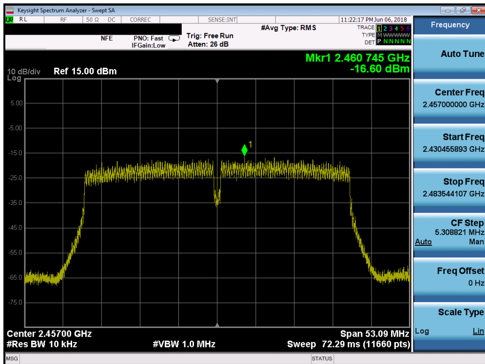
Plot 7-57. Power Spectral Density Plot SISO ANT2 (40MHz 802.11n (2.4GHz) – Ch. 10)
