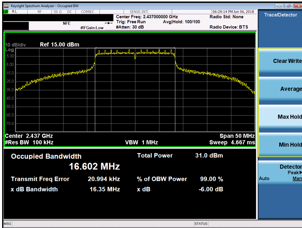
Plot 7-5. 6dB Bandwidth Plot SISO ANT1 (20MHz 802.11g – Ch. 6)
