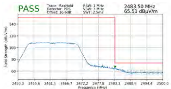
Plot 7-112. Radiated Restricted Upper Band Edge Measurement SISO ANT2 (Peak)
