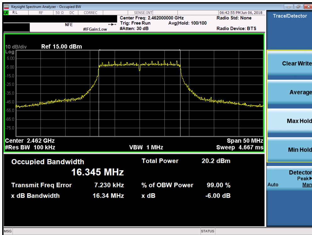
Plot 7-6. 6dB Bandwidth Plot SISO ANT1 (20MHz 802.11g – Ch. 11)
