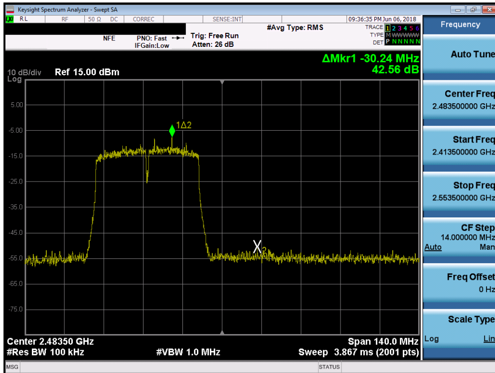
Plot 7-68. Band Edge Plot SISO ANT1 (40MHz 802.11n (2.4GHz) – Ch. 10)
