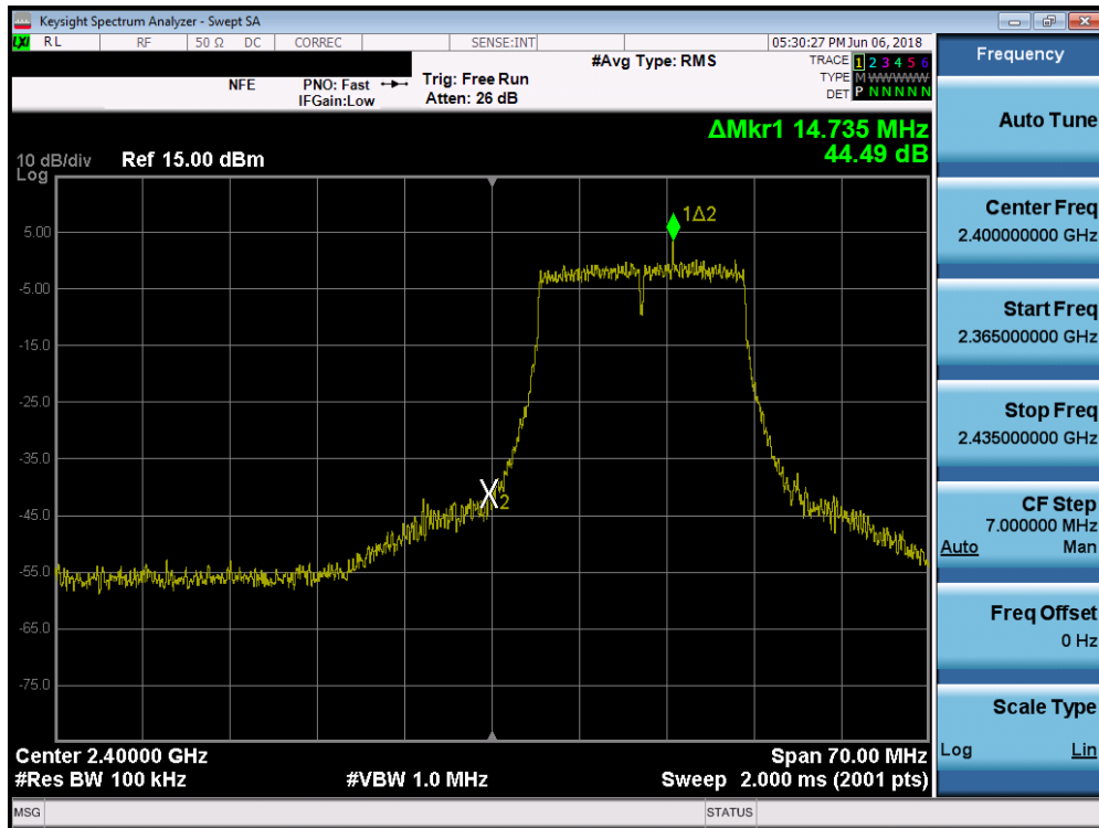
Plot 7-63. Band Edge Plot SISO ANT1 (20MHz 802.11g– Ch. 1)
