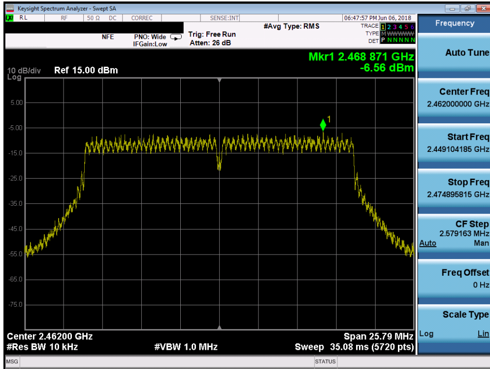
Plot 7-39. Power Spectral Density Plot SISO ANT1 (20MHz 802.11n (2.4GHz) – Ch. 11)
