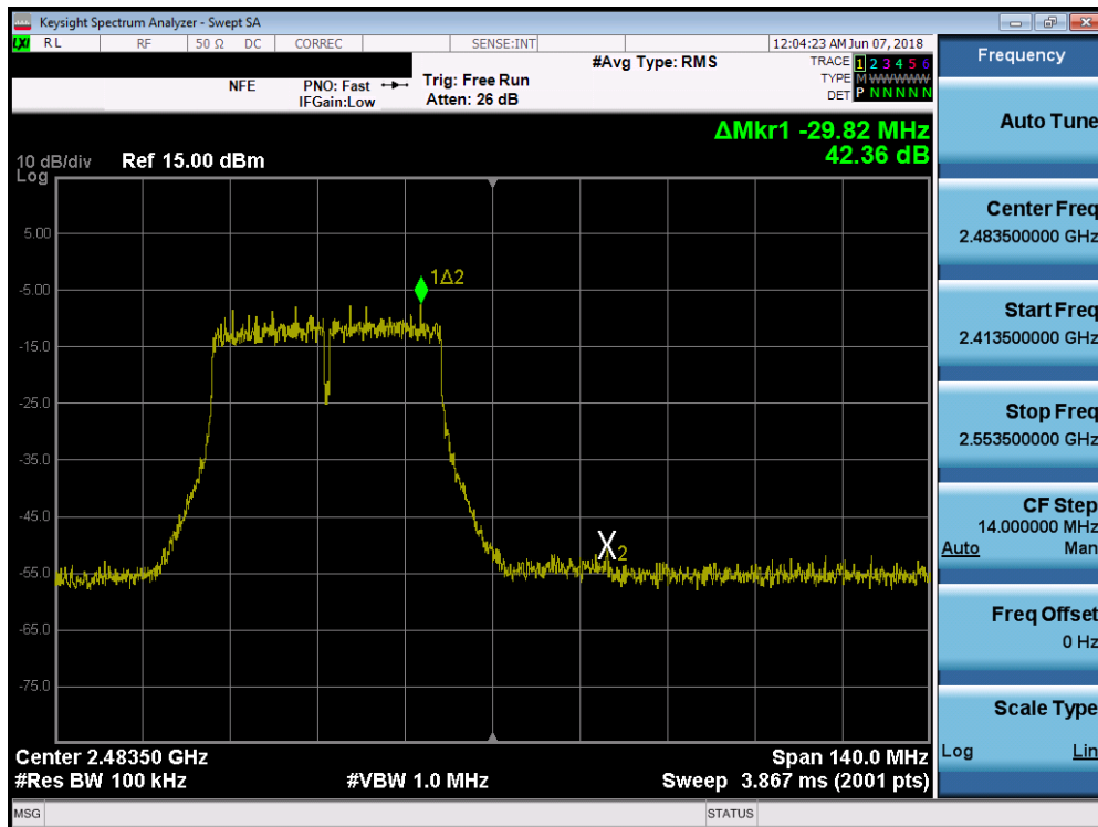
Plot 7-80. Band Edge Plot SISO ANT2 (40MHz 802.11ac (2.4GHz) – Ch. 10)
