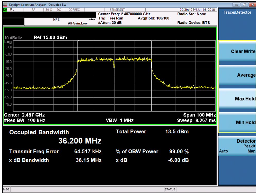
Plot 7-15. 6dB Bandwidth Plot SISO ANT1 (40MHz 802.11ac (2.4GHz) – Ch. 10)
