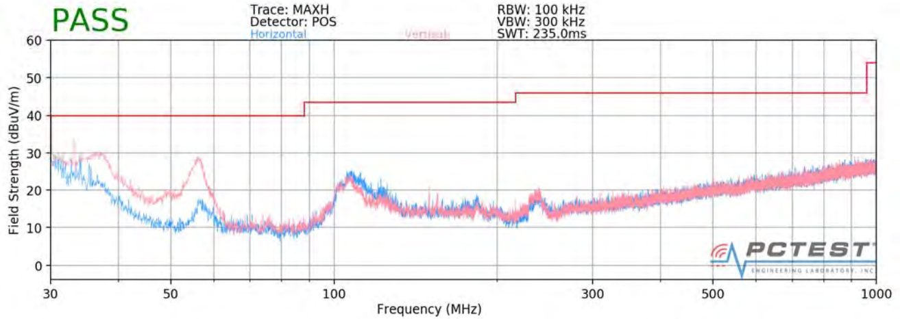
Plot 7-129. Radiated Spurious Plot below 1GHz SISO ANT1
