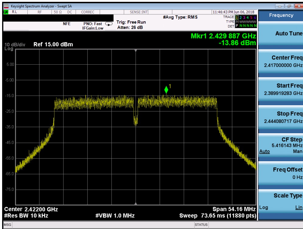
Plot 7-58. Power Spectral Density Plot SISO ANT2 (40MHz 802.11ac (2.4GHz) – Ch. 3)
