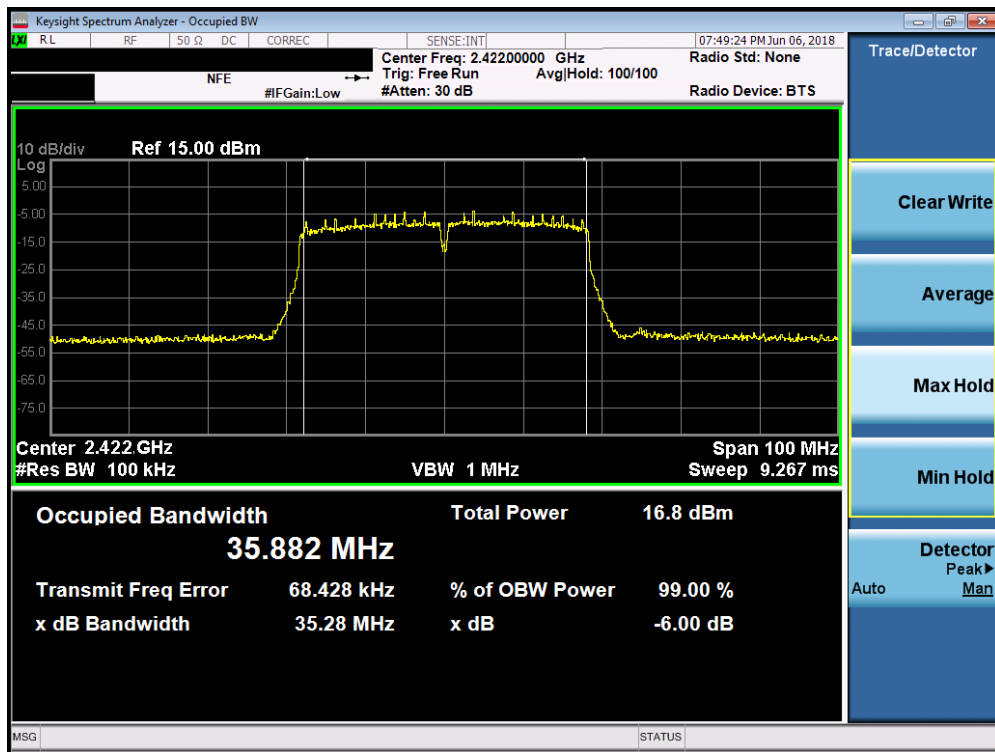
Plot 7-10. 6dB Bandwidth Plot SISO ANT1 (40MHz 802.11n (2.4GHz) – Ch. 3)
