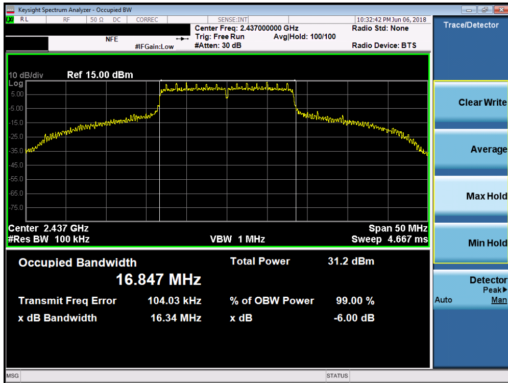
Plot 7-20. 6dB Bandwidth Plot SISO ANT2 (20MHz 802.11g – Ch. 6)
