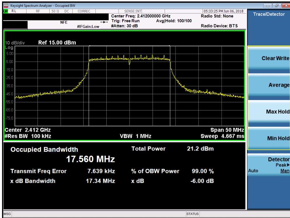
Plot 7-7. 6dB Bandwidth Plot SISO ANT1 (20MHz 802.11n (2.4GHz) – Ch. 1)
