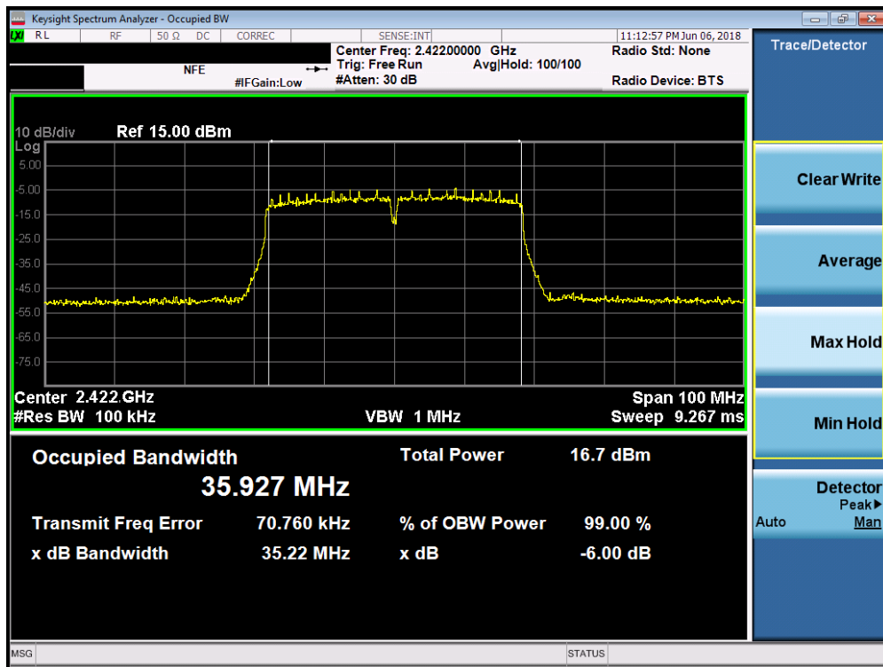
Plot 7-25. 6dB Bandwidth Plot SISO ANT2 (40MHz 802.11n (2.4GHz) – Ch. 3)
