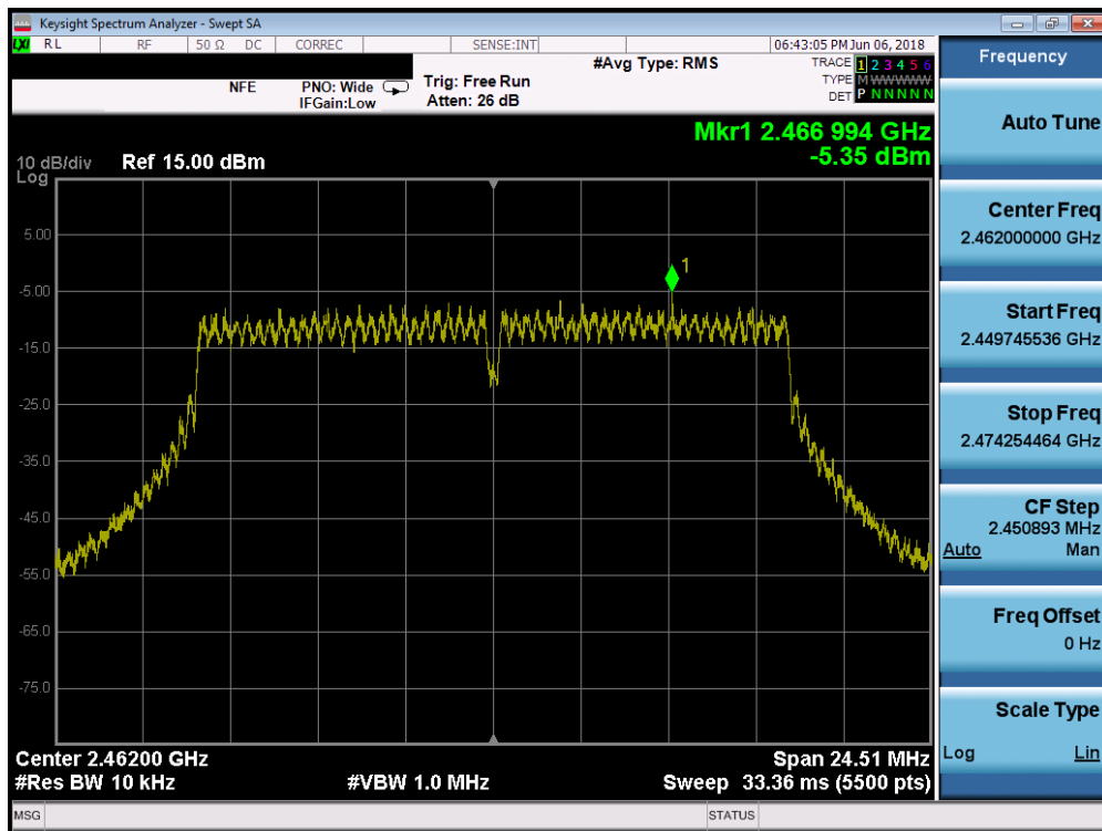
Plot 7-36. Power Spectral Density Plot SISO ANT1 (20MHz 802.11g – Ch. 11)
