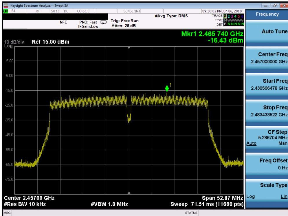
Plot 7-42. Power Spectral Density Plot SISO ANT1 (40MHz 802.11n (2.4GHz) – Ch. 10)
