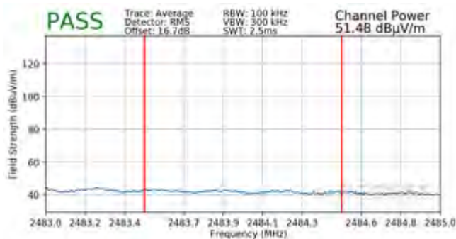
Plot 7-119. Radiated Restricted Upper Band Edge Measurement MIMO (Average)
