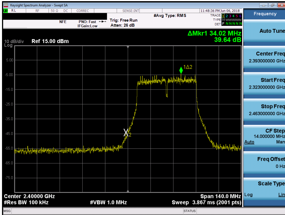
Plot 7-79. Band Edge Plot SISO ANT2 (40MHz 802.11ac (2.4GHz) – Ch. 3)
