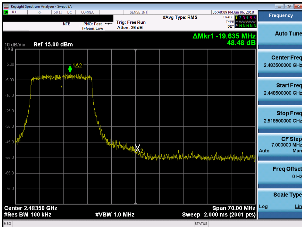
Plot 7-66. Band Edge Plot SISO ANT1 (20MHz 802.11n (2.4GHz) – Ch. 11)
