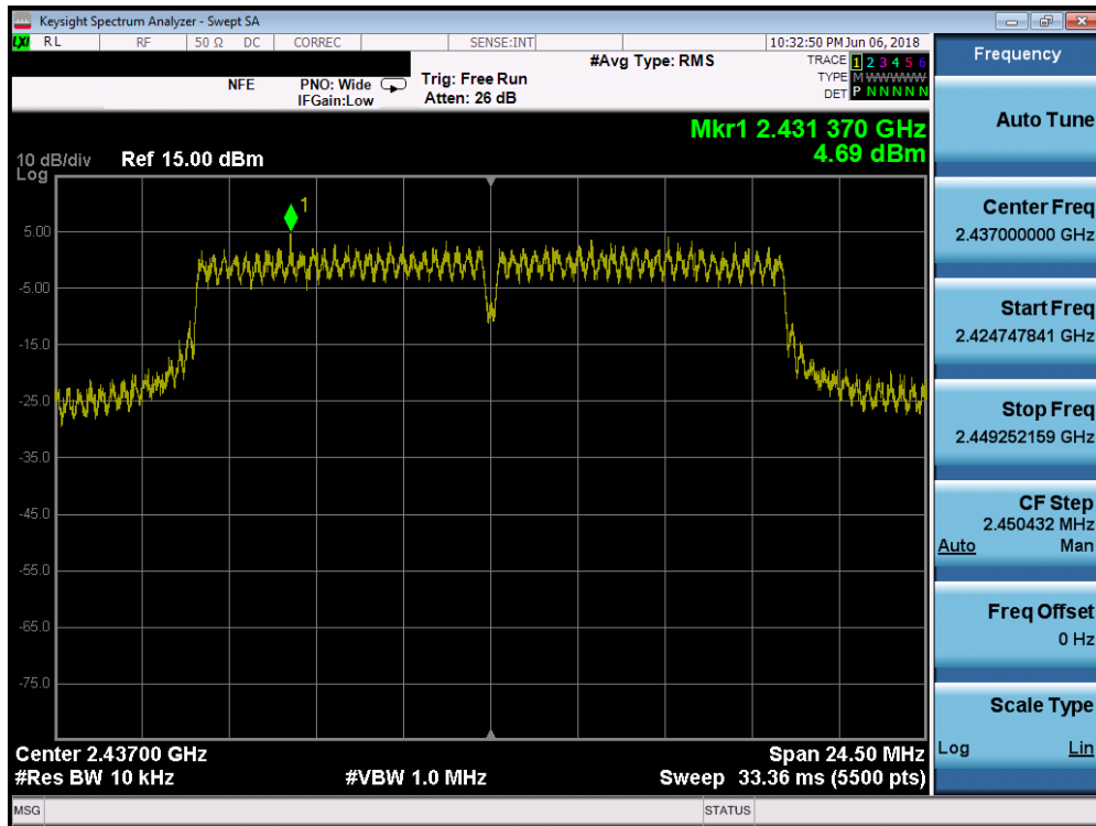
Plot 7-50. Power Spectral Density Plot SISO ANT2 (20MHz 802.11g – Ch. 6)
