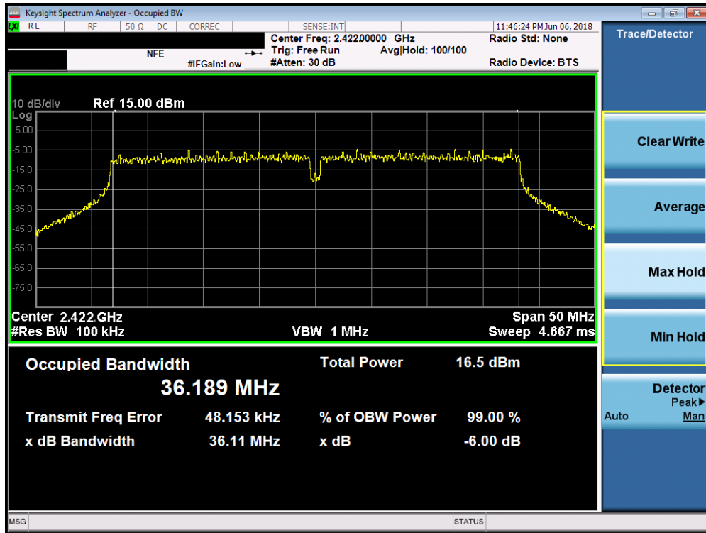
Plot 7-28. 6dB Bandwidth Plot SISO ANT2 (40MHz 802.11ac (2.4GHz) – Ch. 3)
