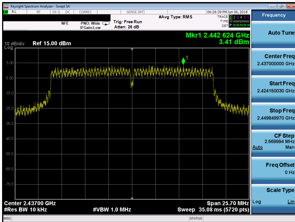
Plot 7-38. Power Spectral Density Plot SISO ANT1 (20MHz 802.11n (2.4GHz) – Ch. 6)
