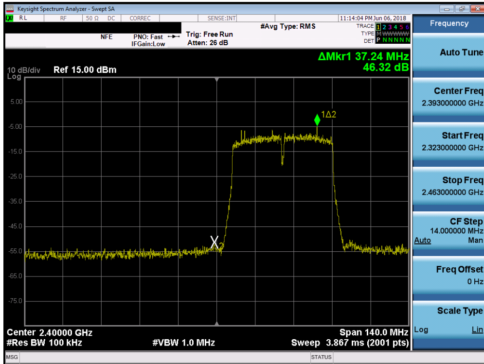
Plot 7-77. Band Edge Plot SISO ANT2 (40MHz 802.11n (2.4GHz) – Ch. 3)
