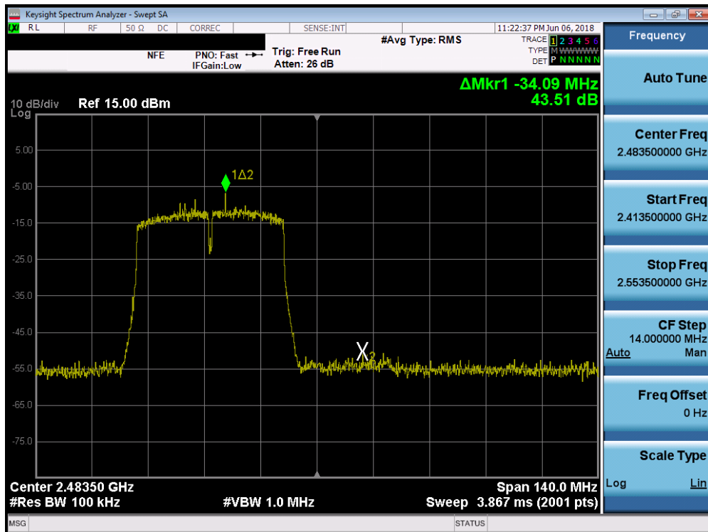
Plot 7-78. Band Edge Plot SISO ANT2 (40MHz 802.11n (2.4GHz) – Ch. 10)
