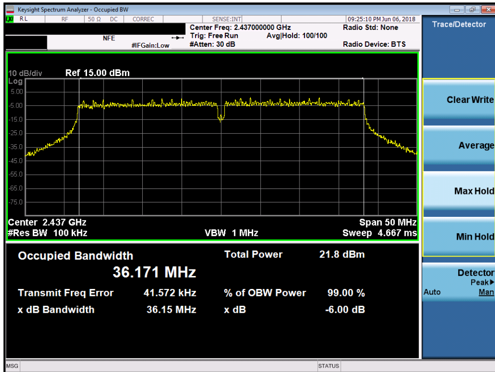
Plot 7-14. 6dB Bandwidth Plot SISO ANT1 (40MHz 802.11ac (2.4GHz) – Ch. 6)
