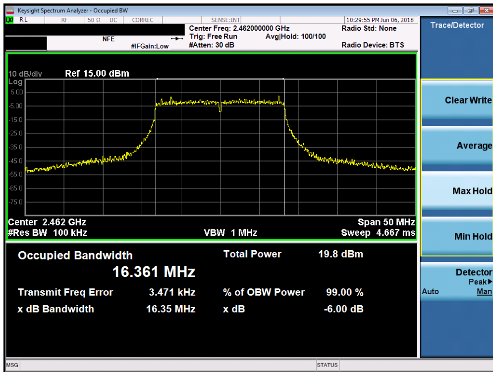
Plot 7-21. 6dB Bandwidth Plot SISO ANT2 (20MHz 802.11g – Ch. 11)
