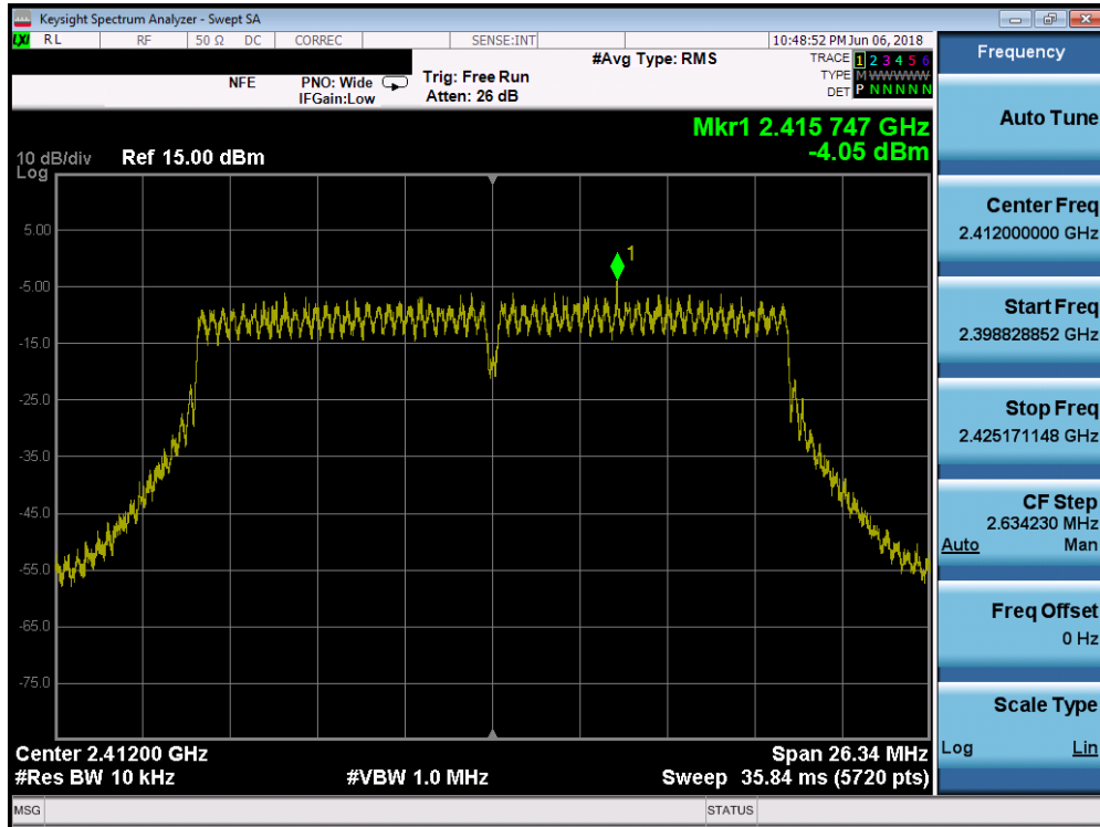
Plot 7-52. Power Spectral Density Plot SISO ANT2 (20MHz 802.11n (2.4GHz) – Ch. 1)
