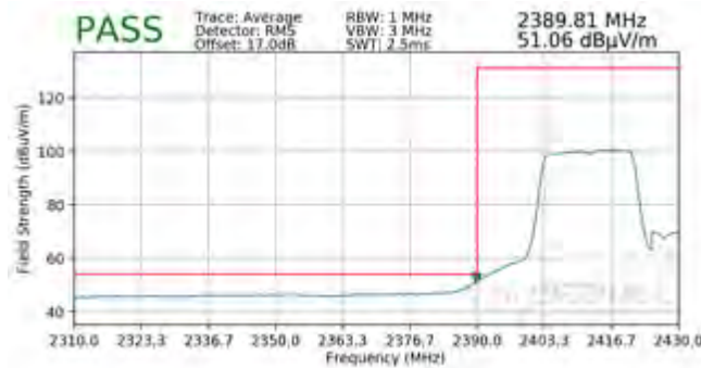
Plot 7-109. Radiated Restricted Lower Band Edge Measurement SISO ANT2 (Average)
