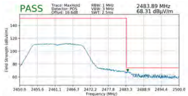
Plot 7-120. Radiated Restricted Upper Band Edge Measurement MIMO (Peak)
