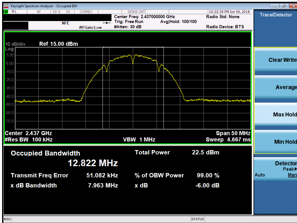
Plot 7-17. 6dB Bandwidth Plot SISO ANT2 (802.11b – Ch. 6)
