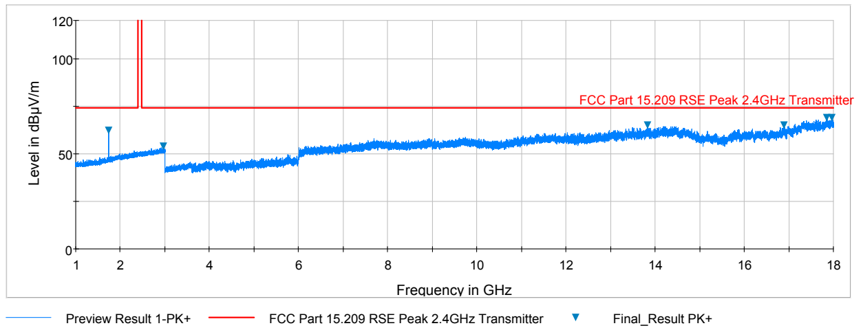
Plot 7-3. Radiated Spurious Plot above 1GHz (Pol. H)
