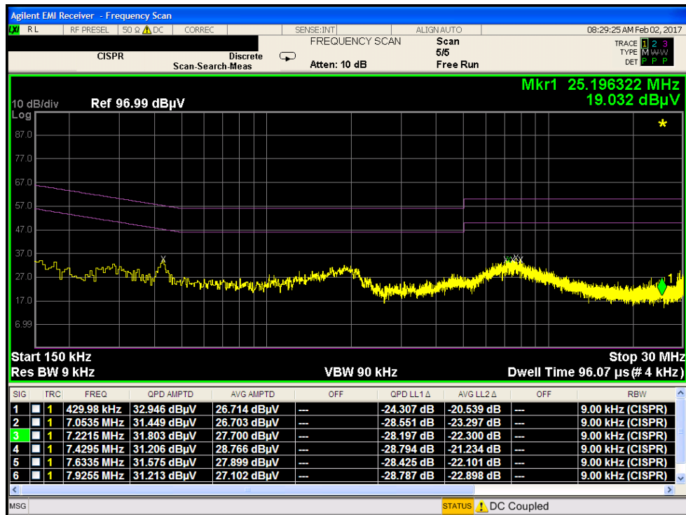
Plot 7-5. Line Conducted Plot (N)
