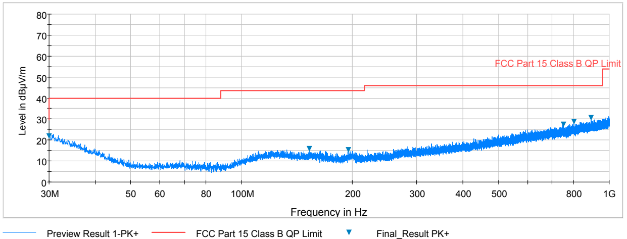
Plot 7-2. Radiated Spurious Plot below 1GHz (Pol. V)
