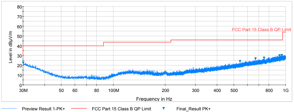
Plot 7-1. Radiated Spurious Plot below 1GHz (Pol. H)
