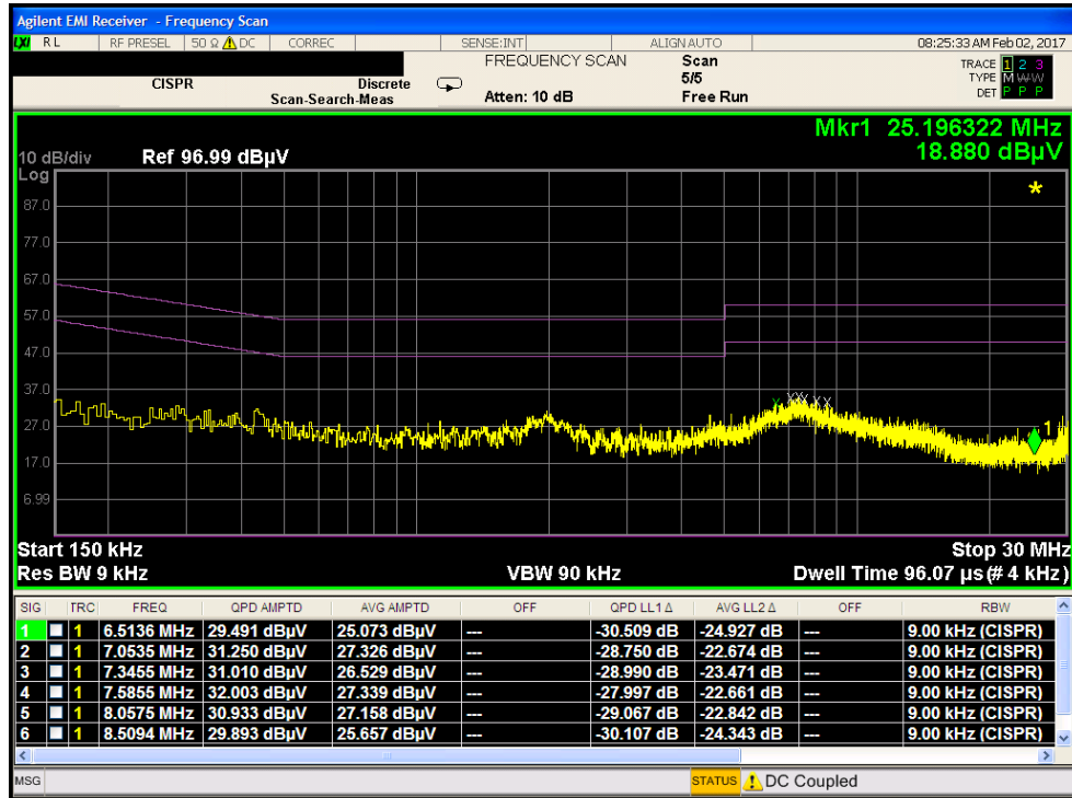
Plot 7-4. Line Conducted Plot (L1)
