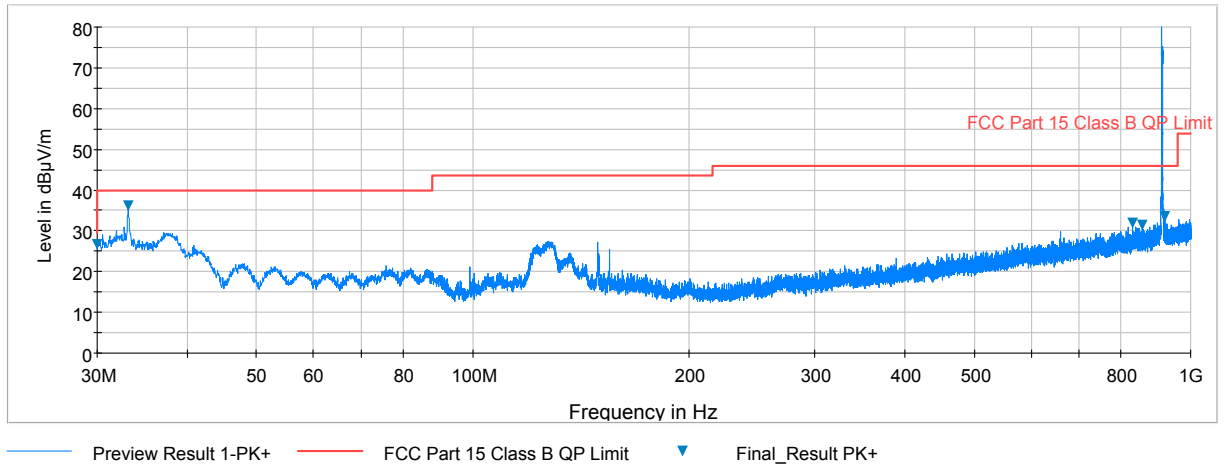
Plot 7-9. Radiated Spurious Plot below 1GHz (Zwave – 916MHz, Ant. Pol. H)
