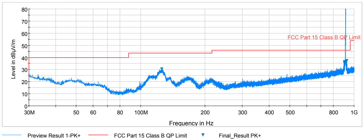
Plot 7-10. Radiated Spurious Plot below 1GHz (Zwave – 916MHz, Ant. Pol. H)
