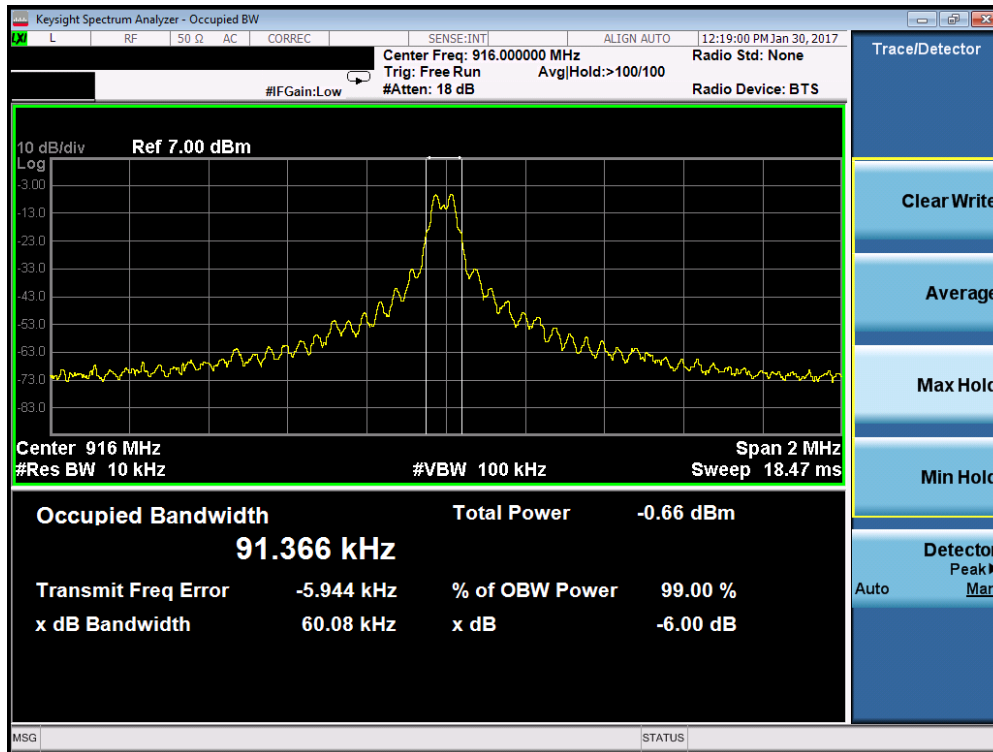
Plot 7-2. Occupied Bandwidth Plot (ZWave – Ch. 916MHz))
