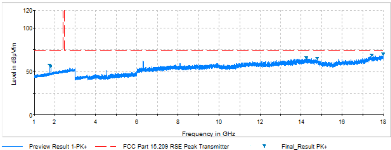
Plot 7-6. Radiated Spurious Plot above 1GHz (Zwave – 916MHz, Ant. Pol. V)
