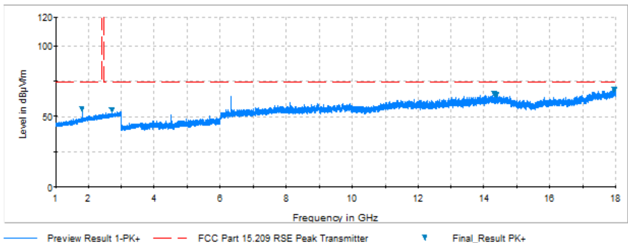
Plot 7-4. Radiated Spurious Plot above 1GHz (Zwave – 908.4MHz, Ant. Pol. V)
