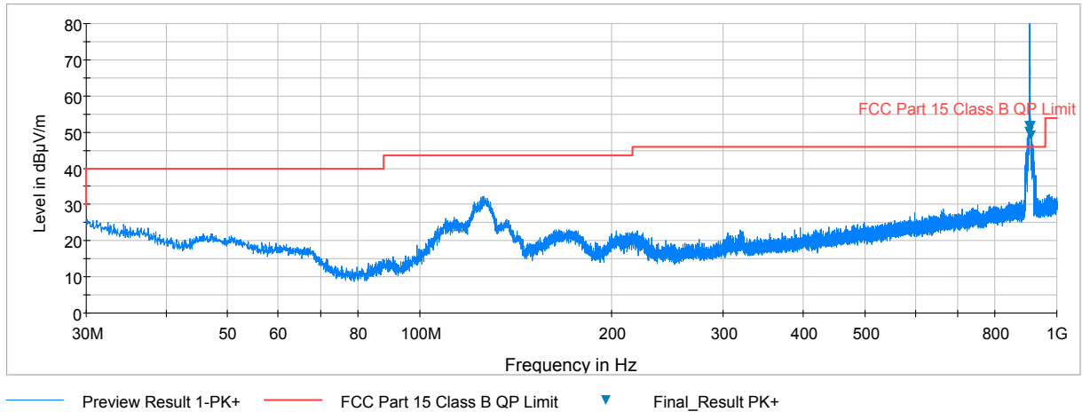
Plot 7-8. Radiated Spurious Plot below 1GHz (Zwave – 908.4MHz, Ant. Pol. H)
