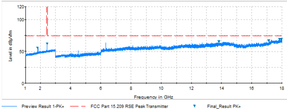
Plot 7-5. Radiated Spurious Plot above 1GHz (Zwave – 916MHz, Ant. Pol. H)
