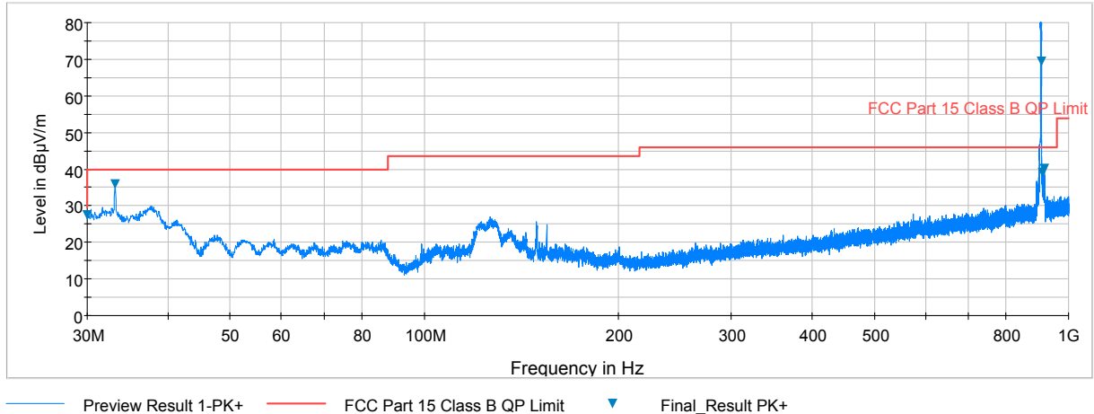
Plot 7-7. Radiated Spurious Plot below 1GHz (Zwave – 908.4MHz, Ant. Pol. H)
