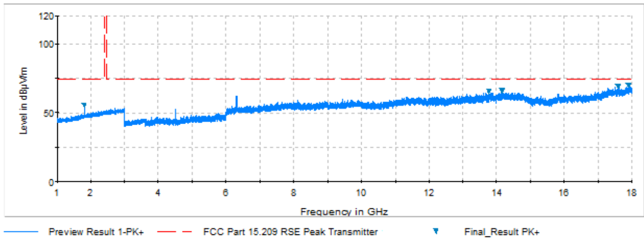
Plot 7-3. Radiated Spurious Plot above 1GHz (Zwave – 908.4MHz, Ant. Pol. H)
