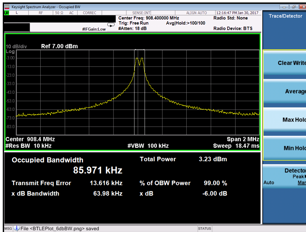
Plot 7-1. Occupied Bandwidth Plot (ZWave – Ch. 908.4MHz)
