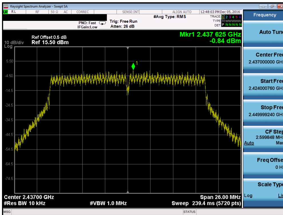
Plot 7-56. Power Spectral Density Plot (802.11n (2.4GHz) – Ch. 6)
