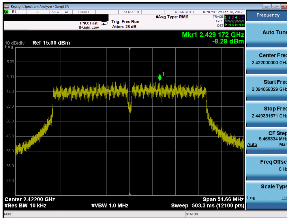
Plot 7-85. Power Spectral Density Plot (40MHz 802.11ac – Ch. 3)
