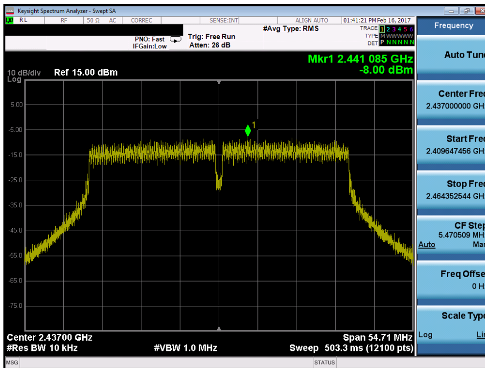
Plot 7-95. Power Spectral Density Plot (40MHz 802.11ac – Ch. 6)
