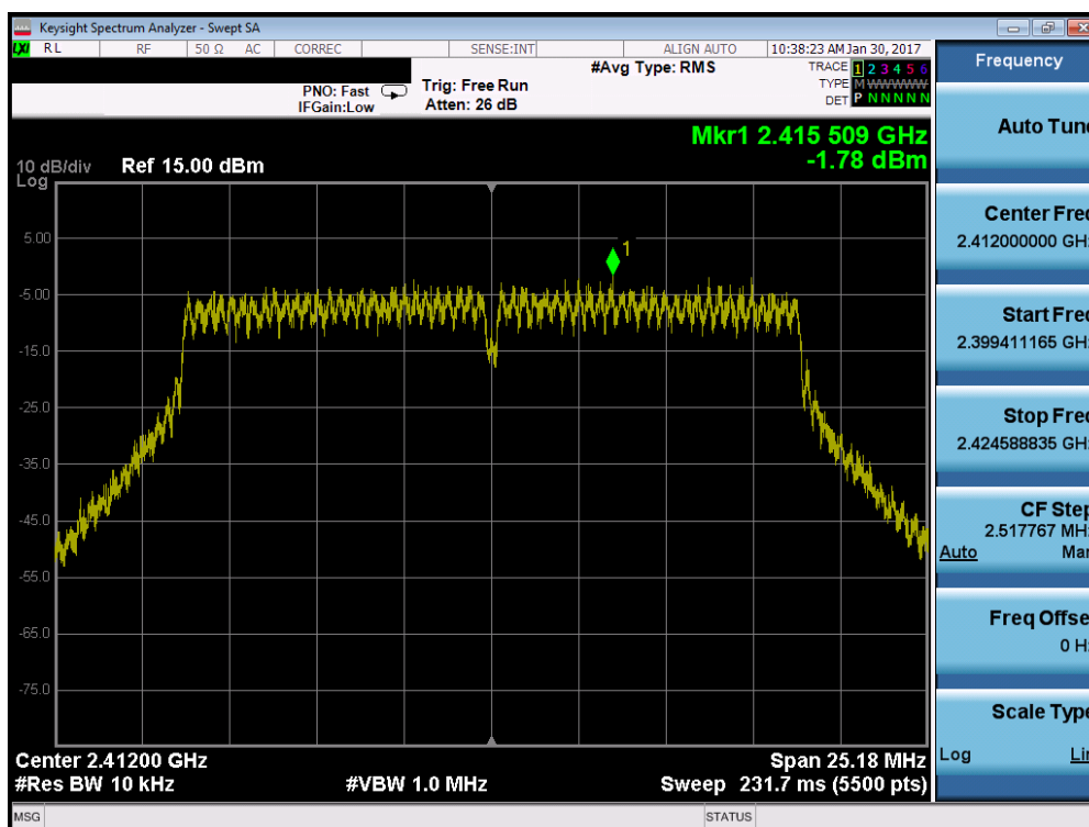
Plot 7-64. Power Spectral Density Plot (802.11n (2.4GHz) – Ch. 1)
