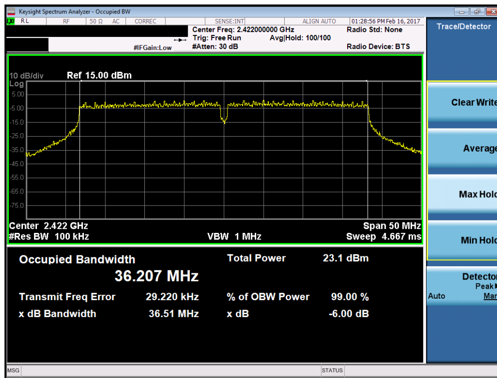
Plot 7-43. 6dB Bandwidth Plot (40MHz 802.11ac – Ch. 3)
