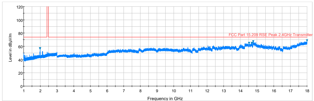
Plot 7-3. Radiated Spurious Plot above 1GHz (Pol. H)
