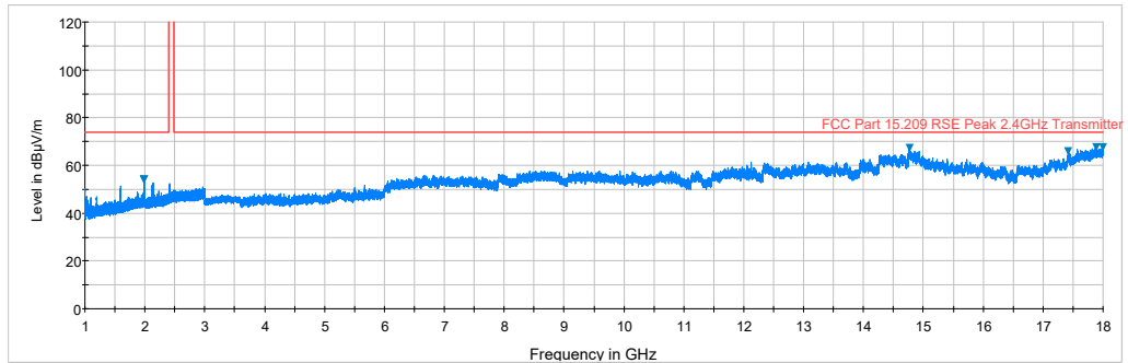
Plot 7-4. Radiated Spurious Plot above 1GHz (Pol. V)
