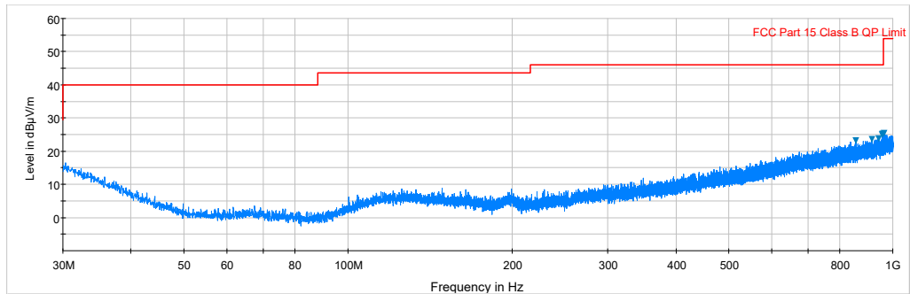
Plot 7-2. Radiated Spurious Plot below 1GHz (Pol. V)
