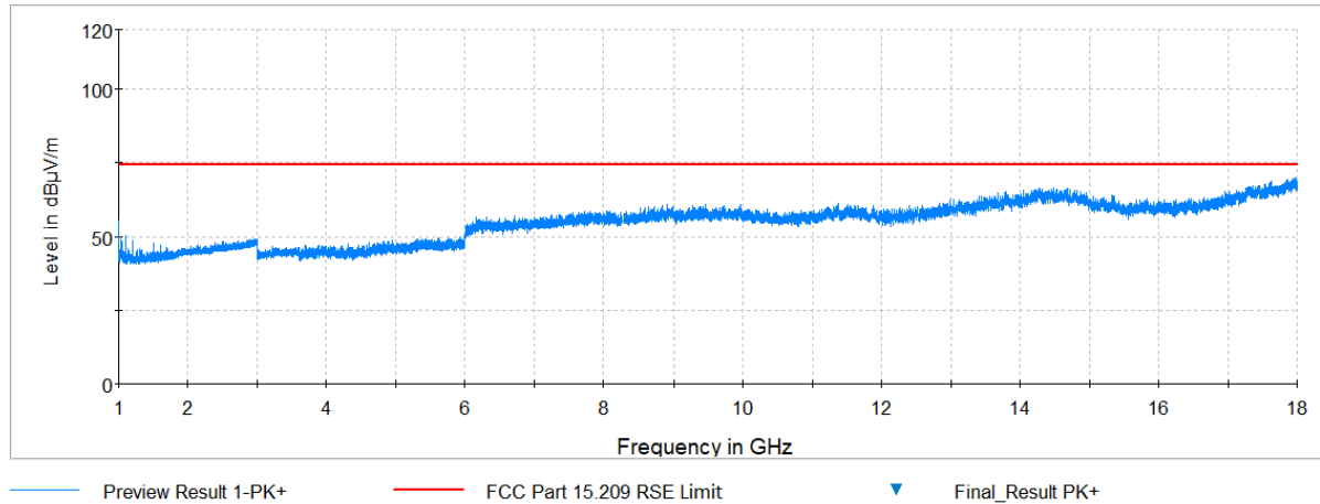
Plot 7-2. Radiated Spurious Plot above 1GHz (Zwave – 921.7MHz, Ant. Pol. H)
