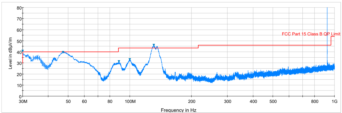
Plot 7-5. Radiated Spurious Plot below 1GHz (Zwave – 921.7MHz, Ant. Pol. V)
