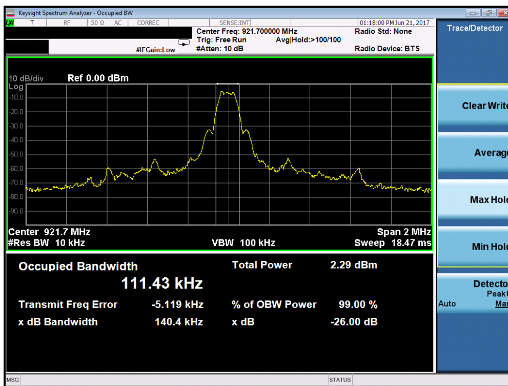
Plot 7-1. Occupied Bandwidth Plot (ZWave – Ch. 921.7MHz)
