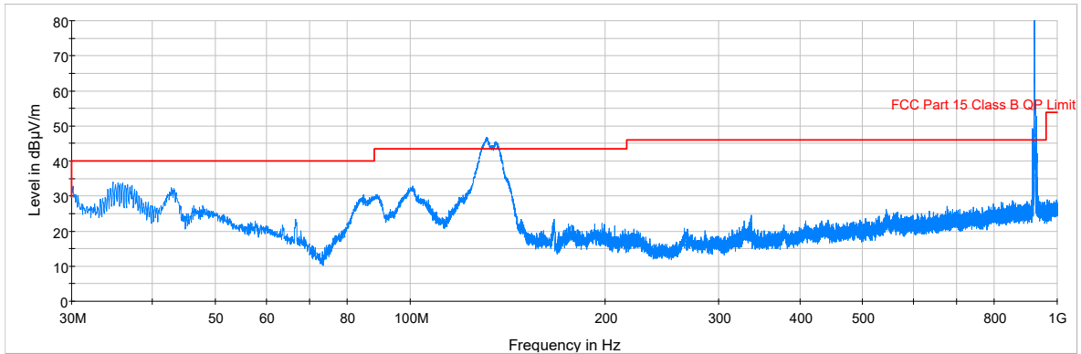
Plot 7-4. Radiated Spurious Plot below 1GHz (Zwave – 921.7MHz, Ant. Pol. H)
