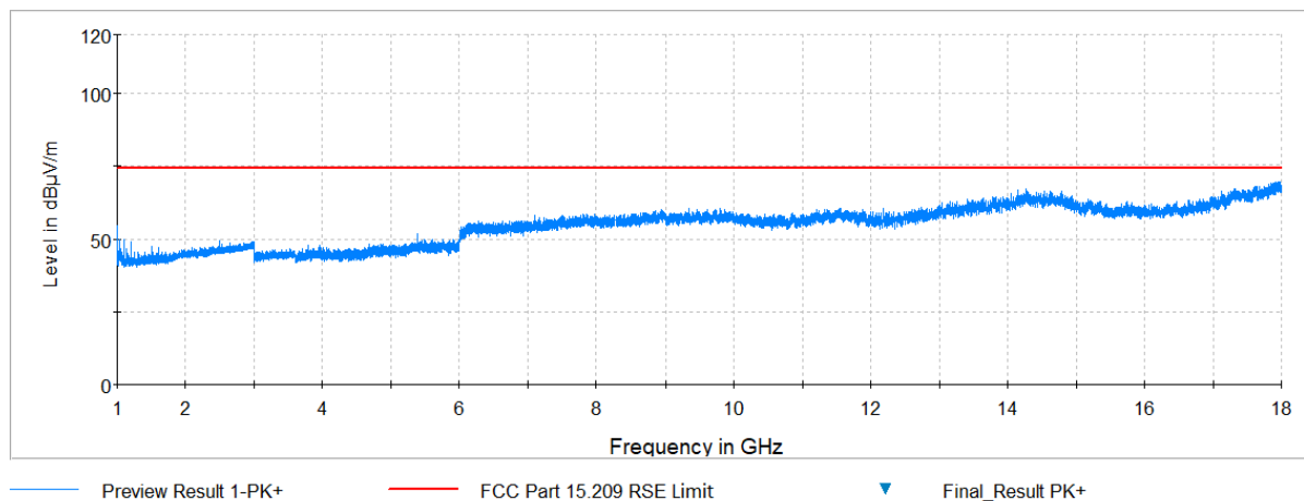
Plot 7-3. Radiated Spurious Plot above 1GHz (Zwave – 921.7MHz, Ant. Pol. V)
