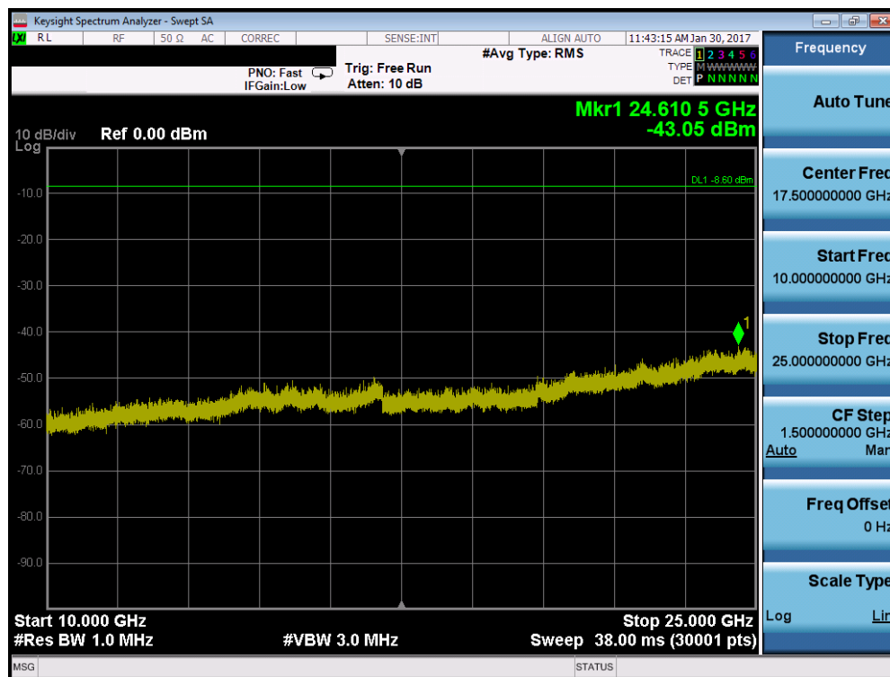
Plot 7-10. Conducted Spurious Plot (ZigBee – Ch. 11)
