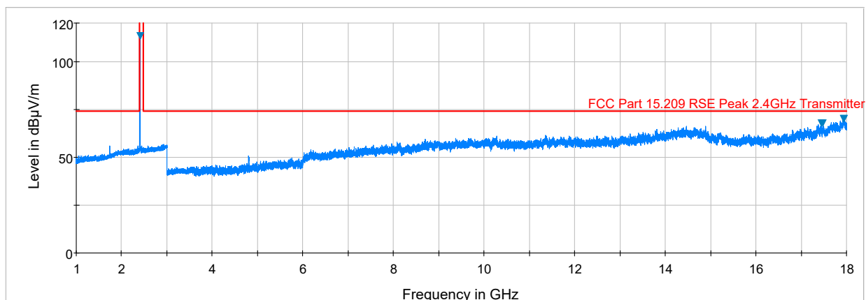
Plot 7-16. Radiated Spurious Plot above 1GHz (Zigbee – Ch. 11, Ant. Pol. V)
