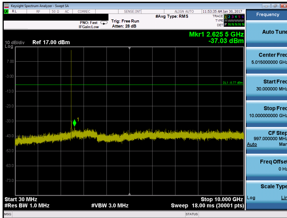
Plot 7-13. Conducted Spurious Plot (ZigBee – Ch. 25)
