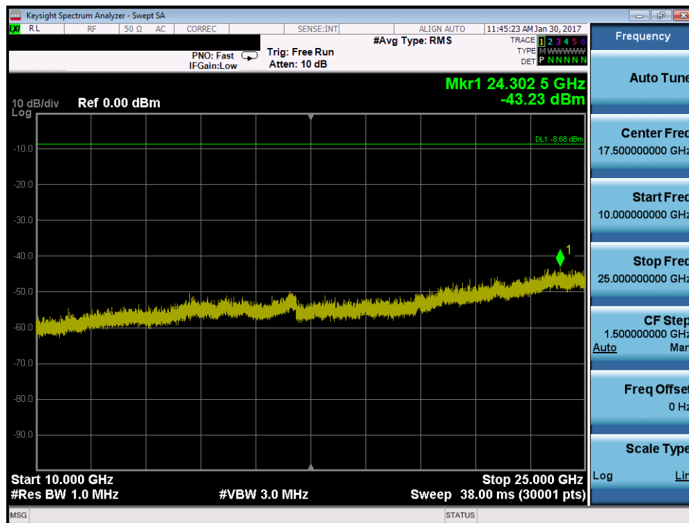
Plot 7-12. Conducted Spurious Plot (ZigBee – Ch. 18)
