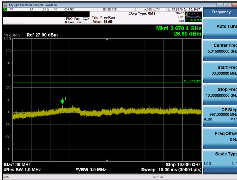
Plot 7-11. Conducted Spurious Plot (ZigBee – Ch. 18)
