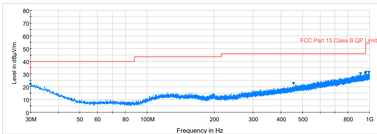
Plot 7-26. Radiated Spurious Plot below 1GHz (Pol. V)
