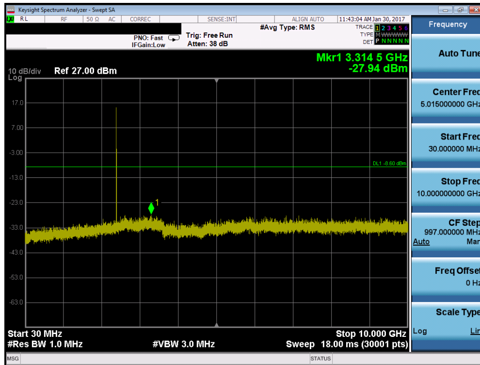
Plot 7-9. Conducted Spurious Plot (ZigBee – Ch. 11)
