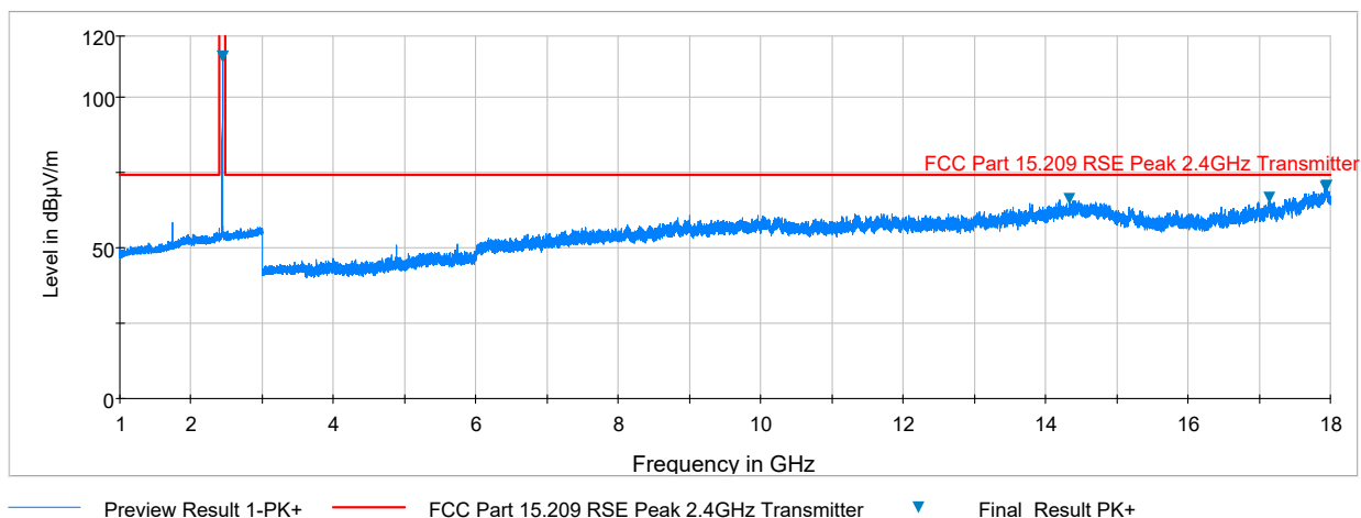
Plot 7-18. Radiated Spurious Plot above 1GHz (Zigbee– Ch. 18, Ant. Pol. V)
