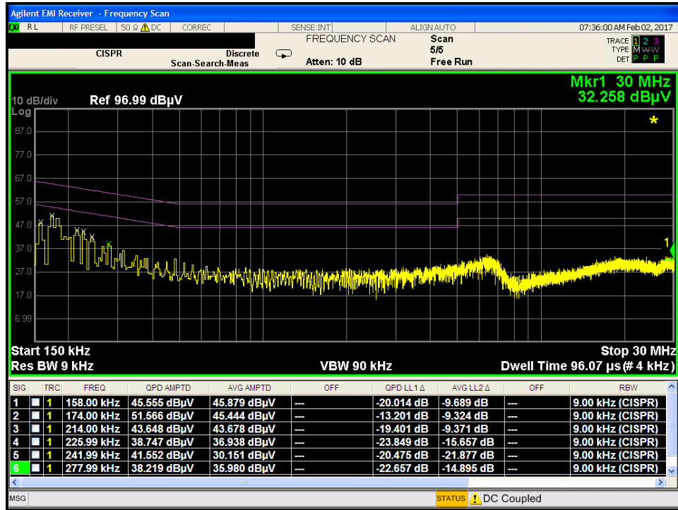
Plot 7-27. Line Conducted Plot with ZigBee (L1)
