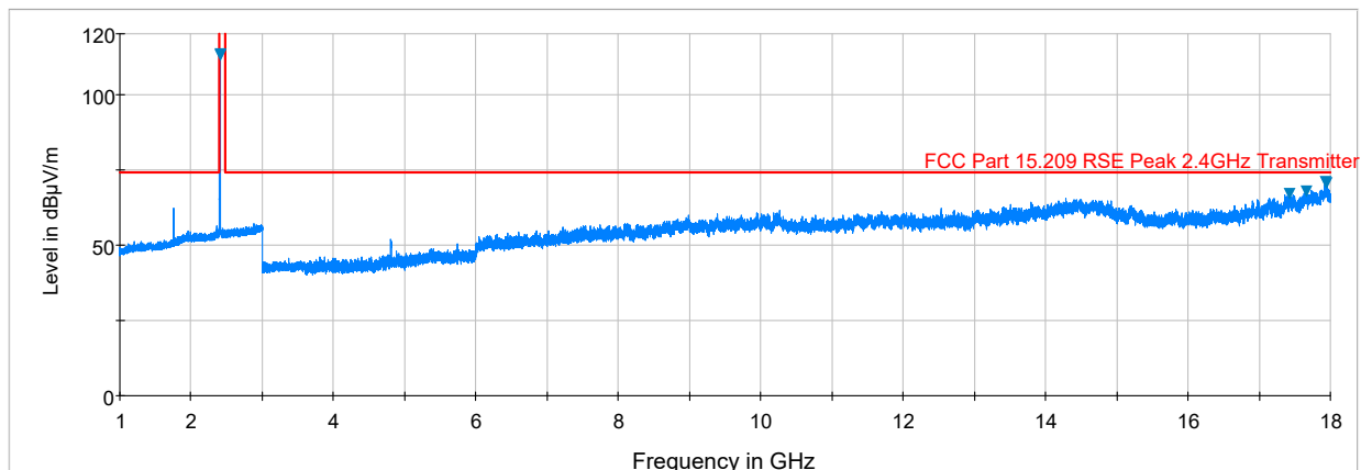
Plot 7-15. Radiated Spurious Plot above 1GHz (Zigbee – Ch. 11, Ant. Pol. H)
