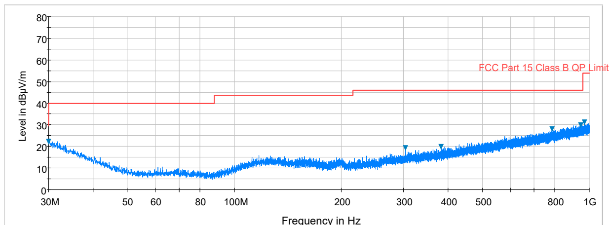
Plot 7-25. Radiated Spurious Plot below 1GHz (Pol. H)
