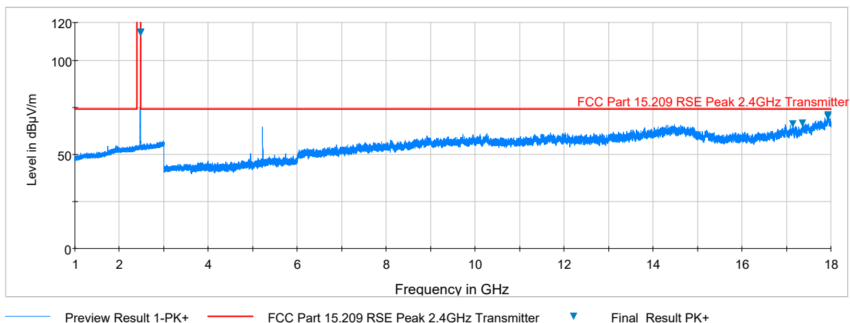
Plot 7-20. Radiated Spurious Plot above 1GHz (Zigbee – Ch. 25, Ant. Pol. V)
