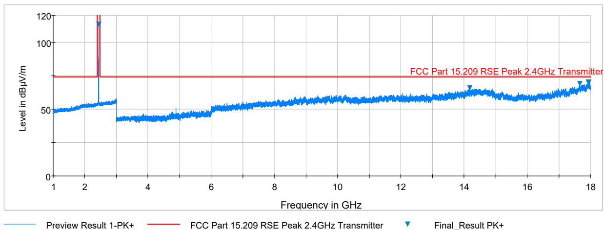
Plot 7-17. Radiated Spurious Plot above 1GHz (Zigbee – Ch. 18, Ant. Pol. H)
