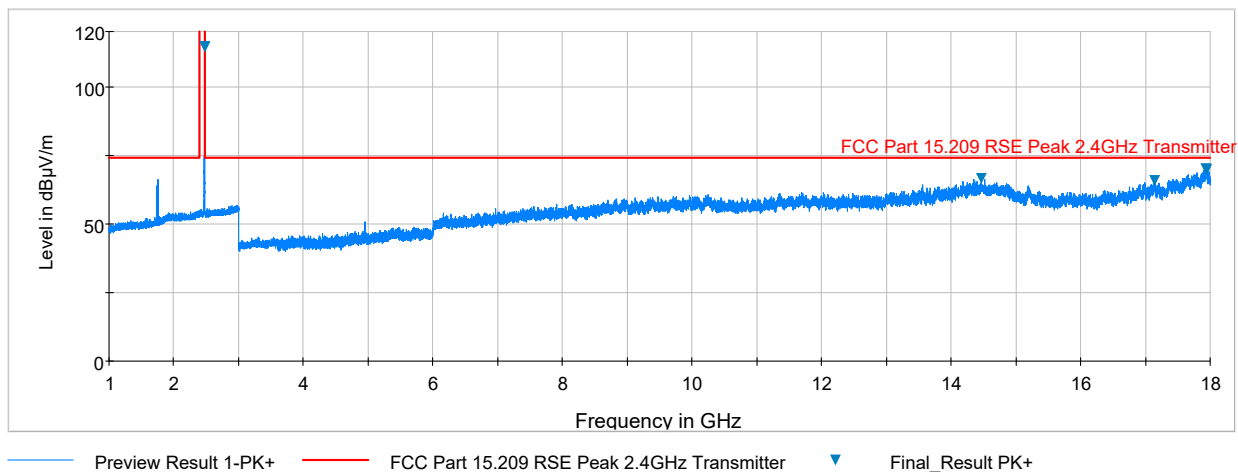
Plot 7-19. Radiated Spurious Plot above 1GHz (Zigbee – Ch. 25, Ant. Pol. H)
