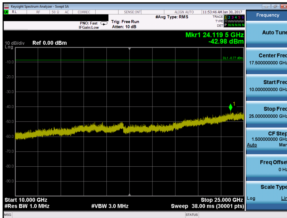
Plot 7-14. Conducted Spurious Plot (ZigBee – Ch. 25)
