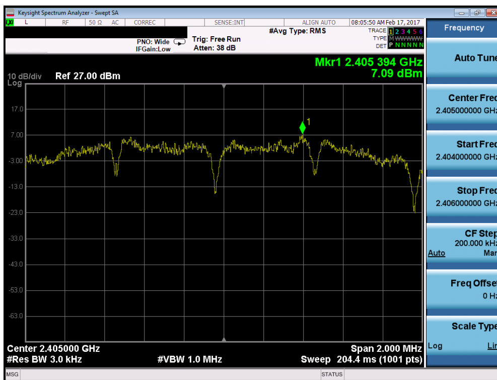
Plot 7-4. Power Spectral Density Plot (ZigBee – Ch. 11)
