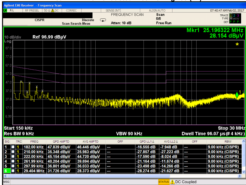
Plot 7-28. Line Conducted Plot with ZigBee (N)
