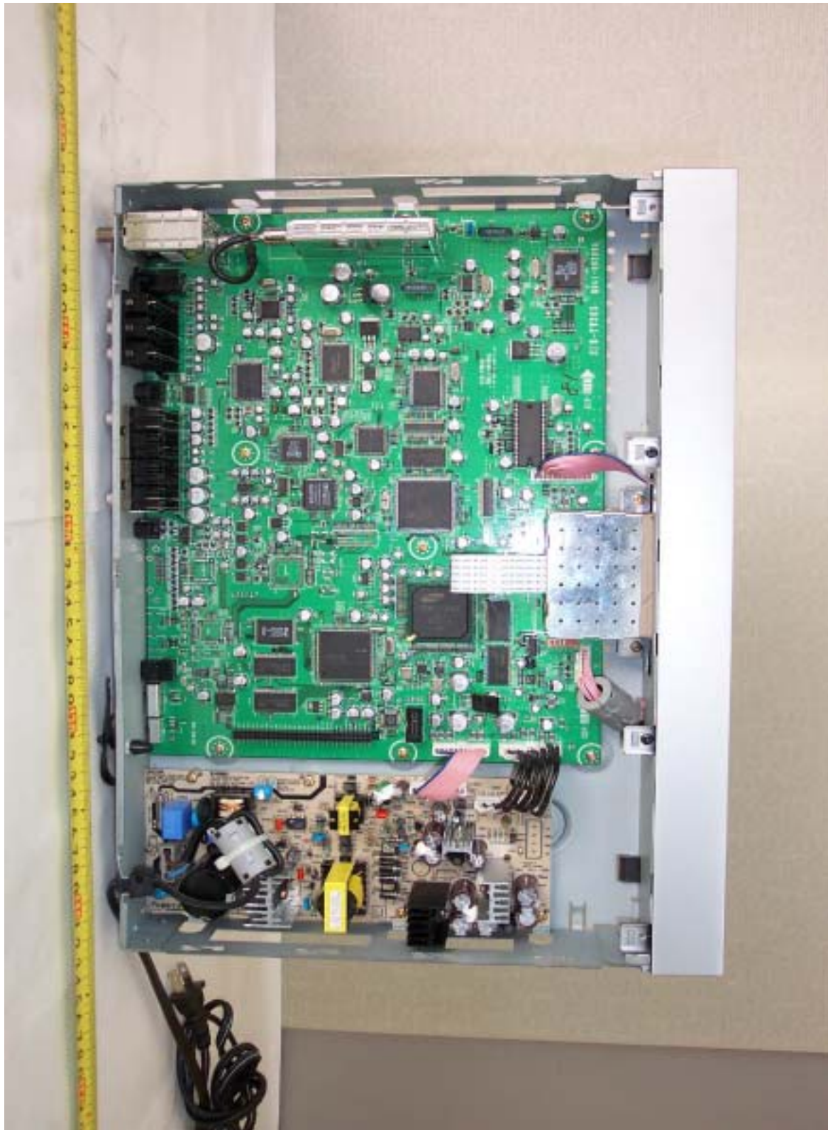
EUT Internal View
