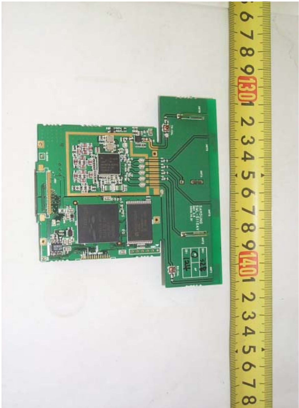
RF Module Top View
