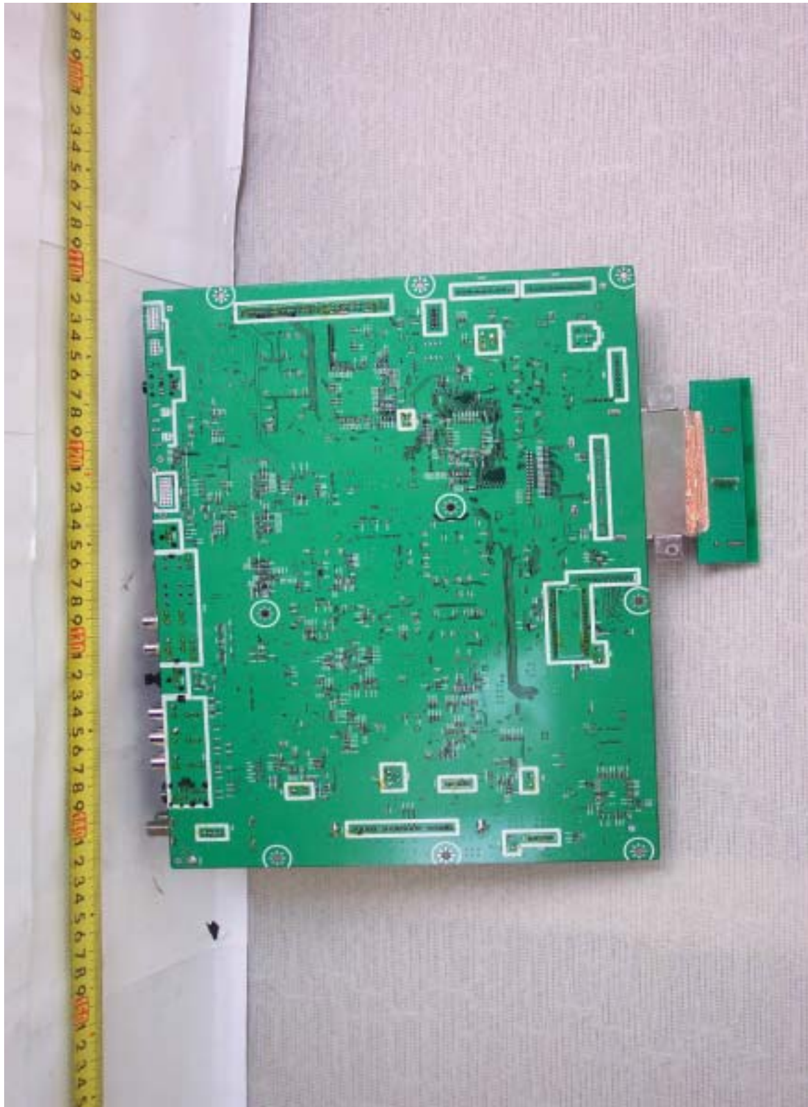
Main Board Bottom View
