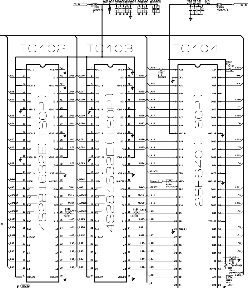
Flash memory configuration
