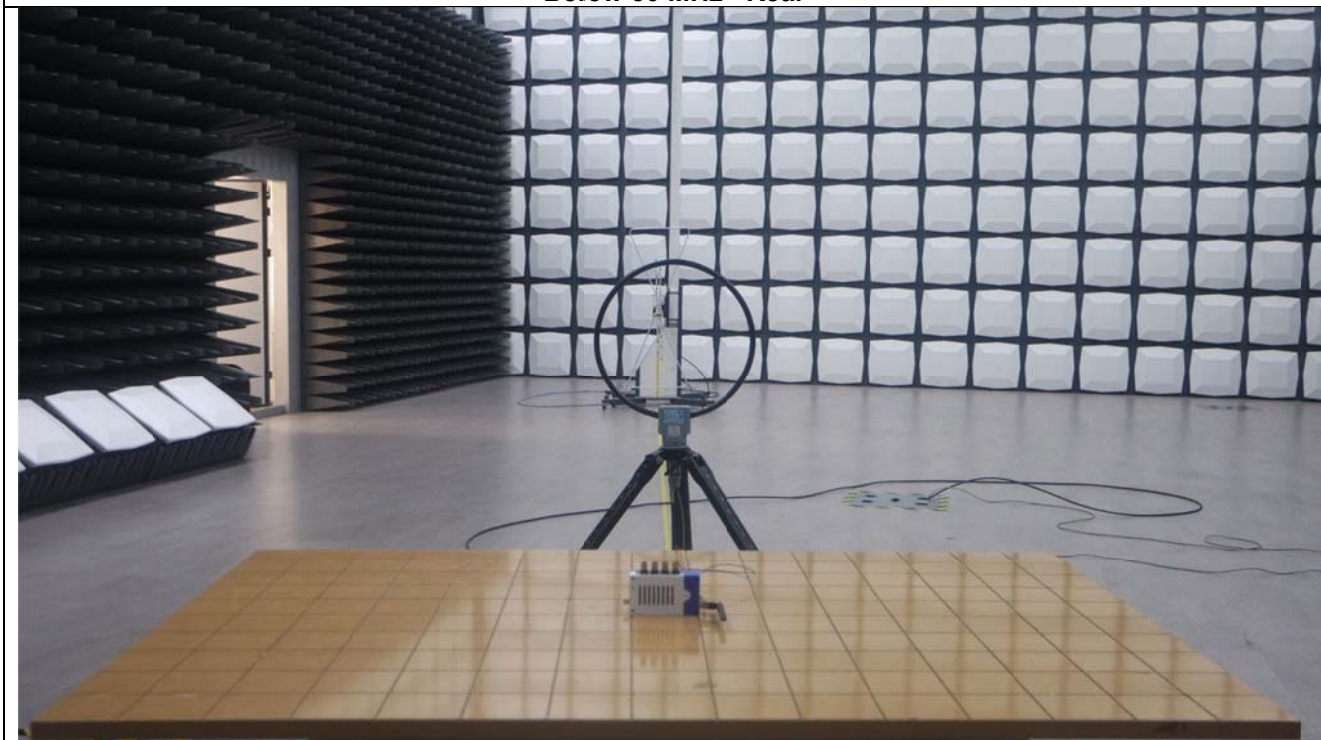
Below 30 MHz - Rear
