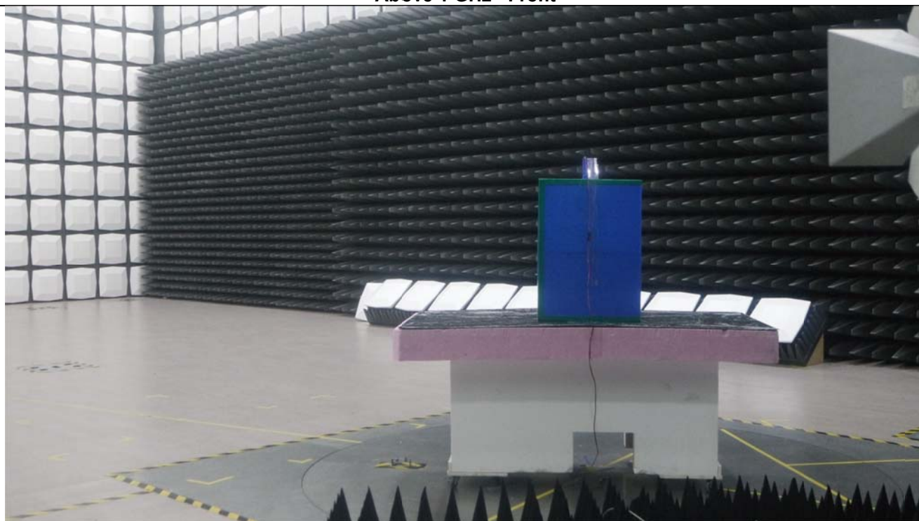
Above 1 GHz - Rear
