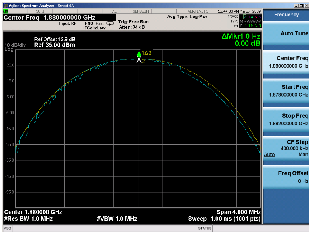
Plot 7-12. Peak-Average Ratio Plot (PCS EDGE GSM Mode – Ch. 661)
